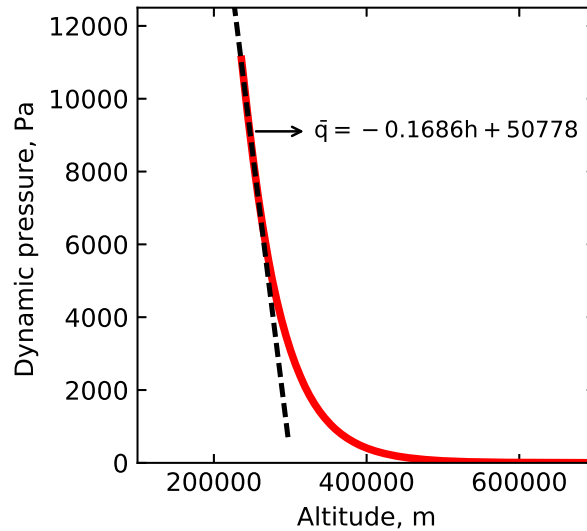
Fig. 22 Actual dynamic pressure profile (solid line) and linear approximation (dashed line) of the used to calculate guidance gain parameters. Based on the method developed by Cerimele and Gamble [55].
