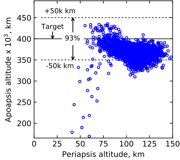
Fig. 18 Apoapsis vs periapsis altitude for reduced atmospheric uncertainty (retrograde entry). Note the improvement compared to the full range of F_{minmax} (Fig. 14)
