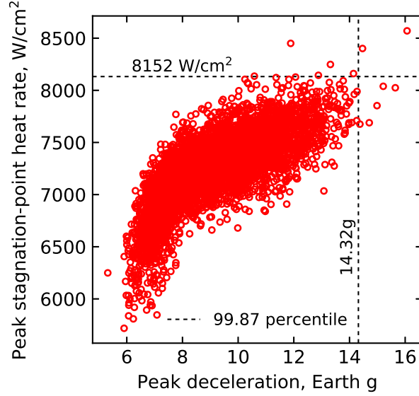
Fig. 15 Peak deceleration and peak stagnation-point heat rate for maximum range of F_{minmax} (retrograde).
