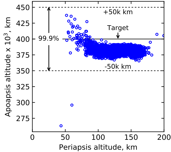
Fig. 19 Apoapsis vs periapsis altitude for reduced atmospheric uncertainty (prograde entry). 99.9% of the cases achieved apoapsis within 50,000 km of the target.
