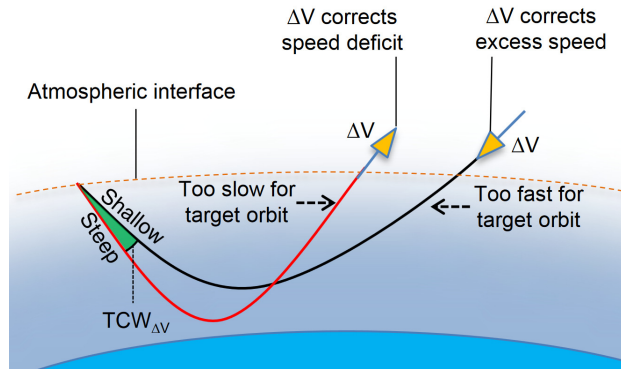
Fig. 9 Second approach where a propulsive \Delta V at atmospheric exit augments control authority.
