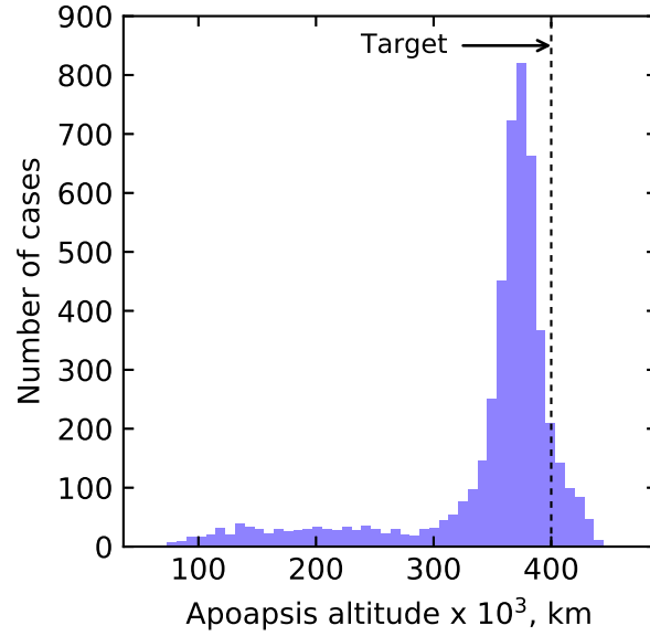
Fig. 13 Histogram of achieved apoapsis altitude for maximum range of F_{minmax} . Some cases resulted in significant undershoot (below 300,000 km).
