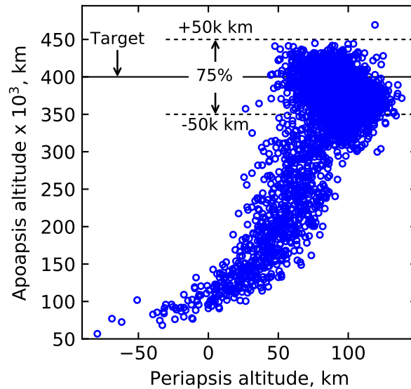
Fig. 14 Apoapsis dispersion for maximum range of F_{minmax} (retrograde). 75% of the cases achieved apoapsis within 50,000 km of the target.
