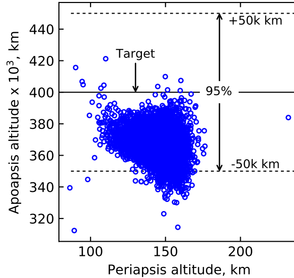
Fig. 20 Apoapsis vs periapsis altitude for very low atmospheric uncertainty (retrograde entry). Note the significant improvement compared to Figs. 14 and 18.
