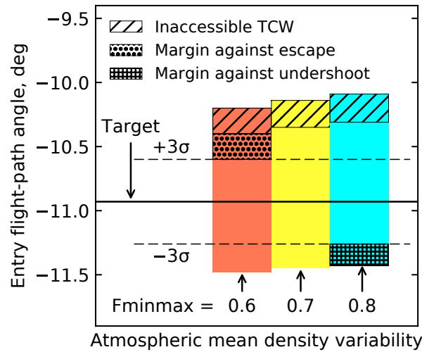
Fig. 12 Reduced atmospheric uncertainty from a pathfinder probe allows target EFPA selection such that both +3\sigma and -3\sigma delivery errors fall within the usable corridor.
