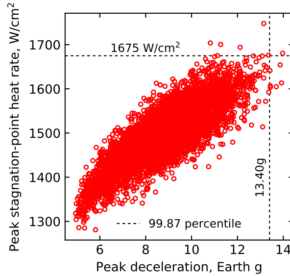
Fig. 17 Peak deceleration vs peak stagnation-point heat rate for maximum range of F_{minmax} (prograde). Note the reduction in heat rate compared to retrograde entry (Fig. 15).
