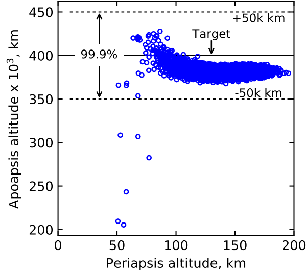
Fig. 21 Apoapsis vs periapsis altitude for very low atmospheric uncertainty (prograde entry). The accuracy is significantly improved compared to Fig. 16, but is similar to Fig. 19.
