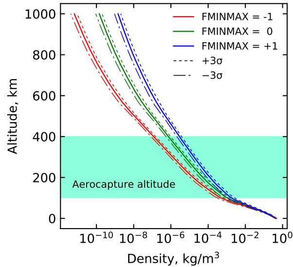
Fig. 3 Mean density profile variations from Neptune-GRAM by varying F_{minmax} from -1 to +1 and \pm 3\sigma uncertainties about the mean profiles.
