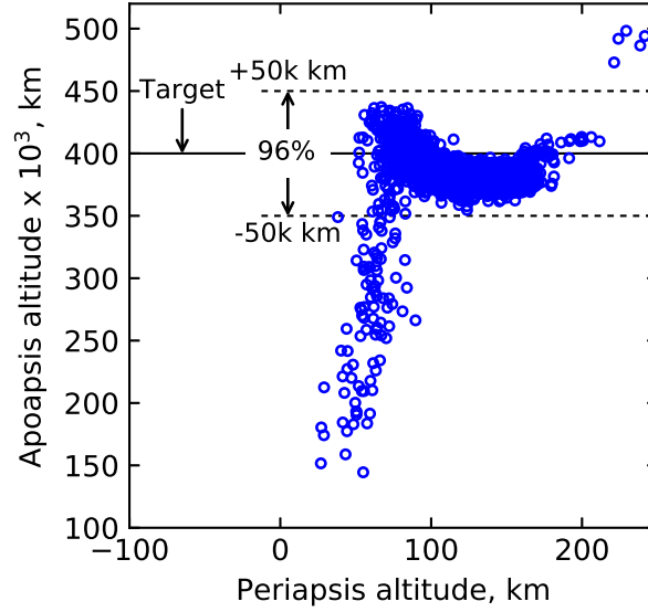
Fig. 16 Apoapsis vs periapsis altitude for maximum range of F_{minmax} (prograde). 96% of the cases achieved apoapsis altitude within 50,000 km of the target.
