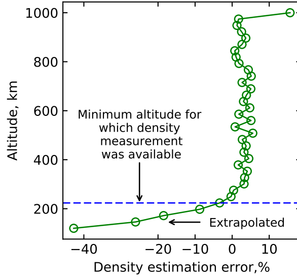
Fig. 7 Density estimation error. Below the minimum altitude for which on-board measurements are available, an exponential extrapolation is used.
