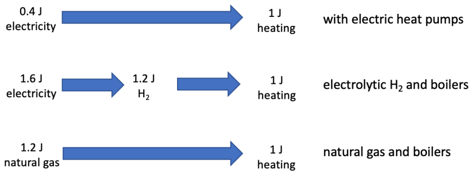
Figure 2. Comparative efficiencies of heat decarbonisation pathways.
