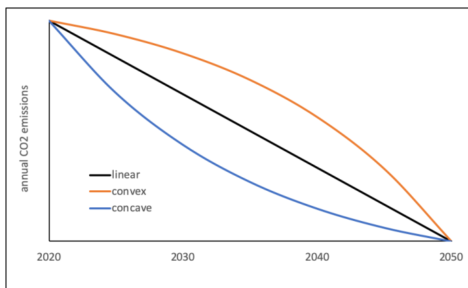
Figure 1. Sketch of concave and convex CO 2 emissions trajectories.
