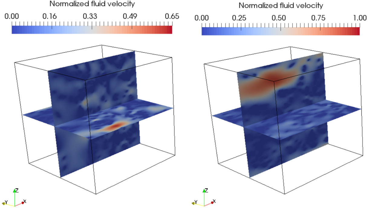
Fig. 2 Normalized velocity contours for TT (left) and IP (right) oriented FiberForm for pressure driven Argon flow. Featured planes are parallel to the flow direction. Dark blue spots depict zero fluid velocity.
