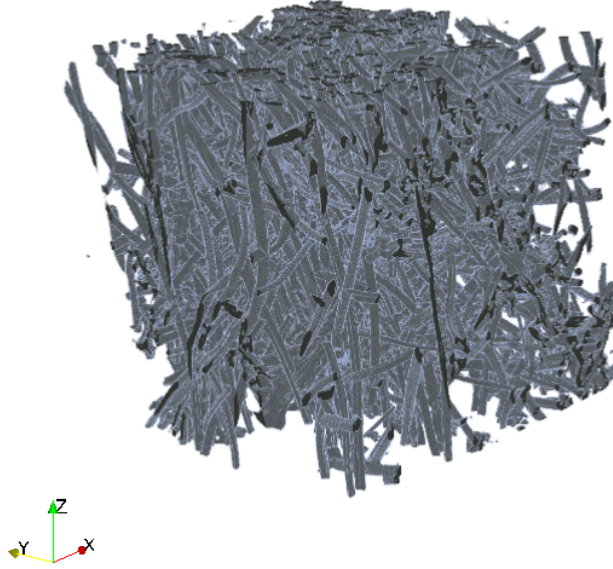
Fig. 1 Voxelized representation of a FiberForm sample, obtained by x-ray micro-computed tomography [24]. TT orientation is along x -axis, IP orientations are in the yz -plane.
