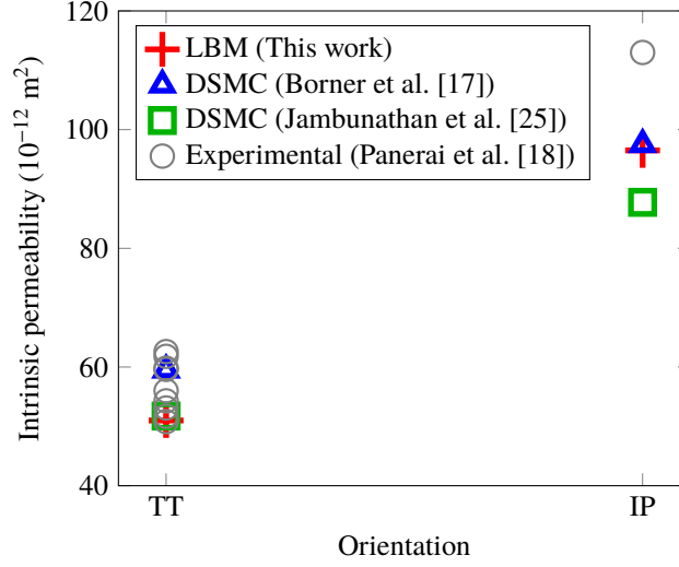
Fig. 3 Intrinsic permeability values for TT and IP FiberForm orientations.
