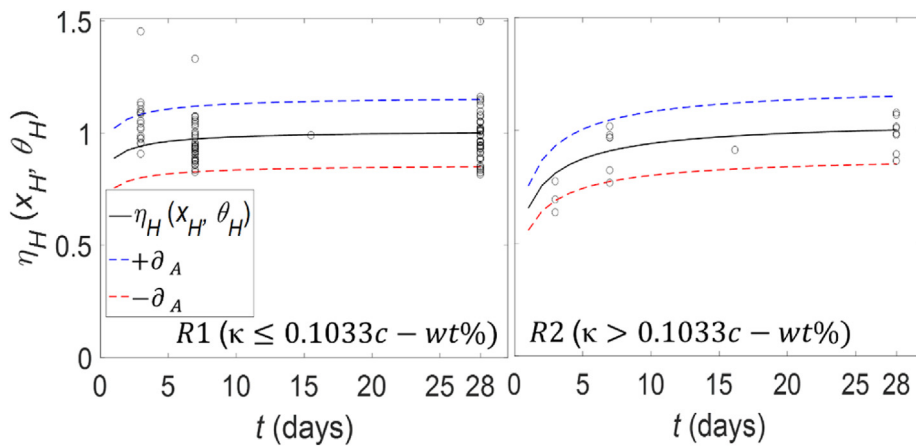
Fig. 3. Estimated vs. measured \eta_H(x_H, \theta_H) as a function of t and its interaction with \kappa .
