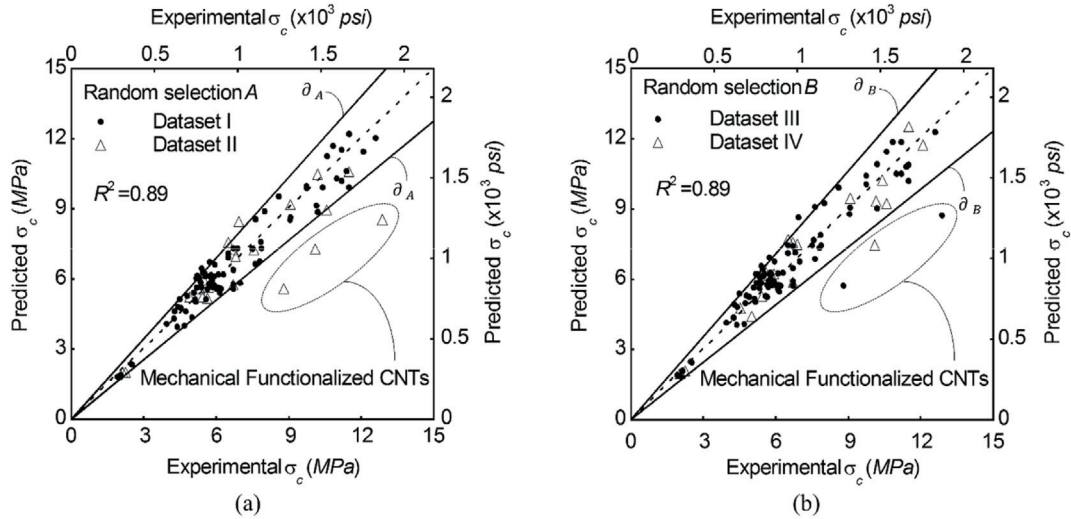
Fig. 1. Predicted value of flexural strength versus experimental results (a) random selection A (b) random selection B (datasets I & III are used for model development and datasets II & IV are used for model validation).
