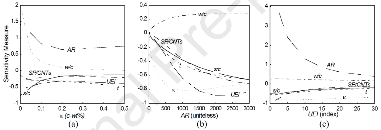
Fig. 10. Sensitivity measures for flexural strength as functions of (a) \kappa (b) AR (c) UEI
