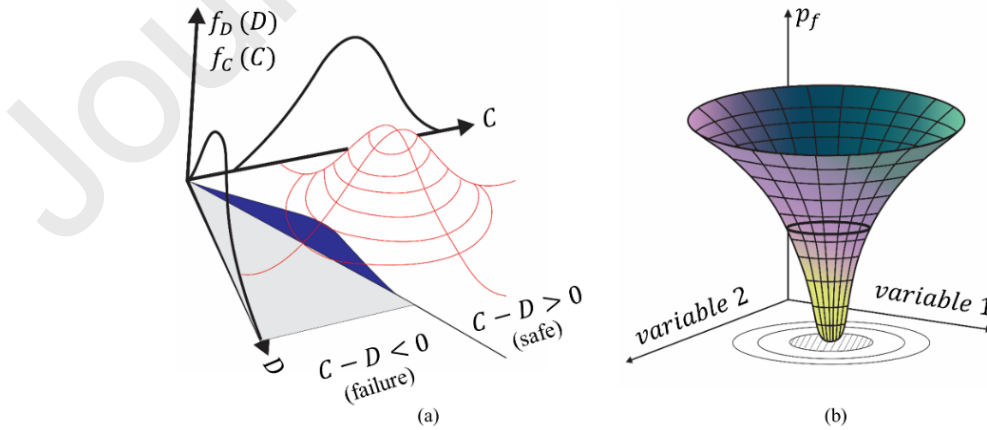
Fig. 5. Visualization of probability of failure: (a) joint probability density function (b) isoprobability lines
