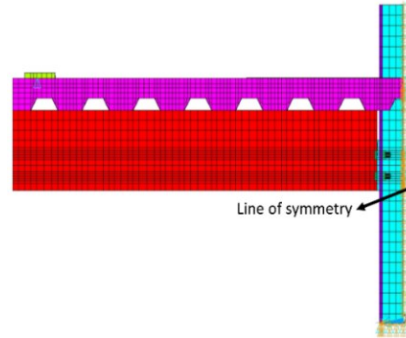
Figure 2. Typical finite element model with Boundary conditions.
