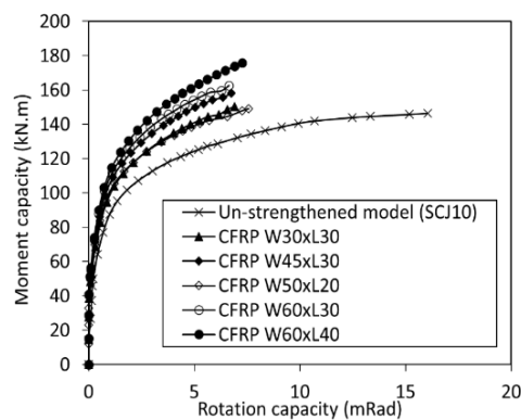
Figure 8. Moment-rotation curves for un-strengthened and strengthened models.
