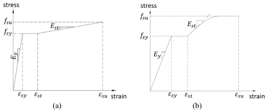
Figure 4. Stress-strain curve for (a) steel reinforcement bars (b) beam, column, bolts and steel deck.
