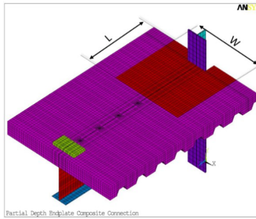
Figure 7. Typical FE model of a composite connection strengthened with CFRP laminate.
