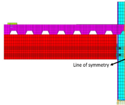
Figure 2. Typical finite element model with Boundary conditions.
