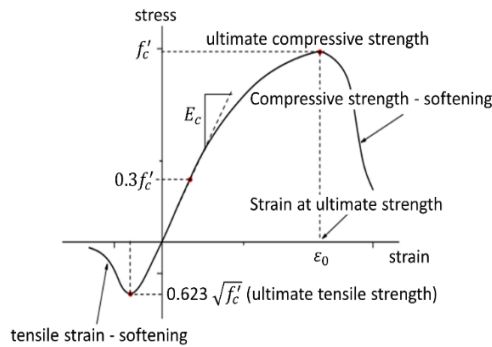
Figure 3. Uniaxial stress-strain curve adopted for concrete.
