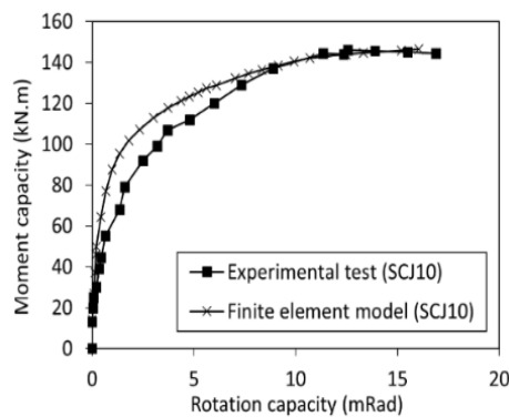
Figure 5. Comparisons between experimental and FEM results.
