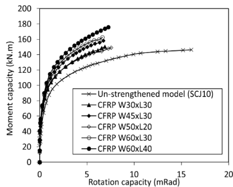
Figure 8. Moment-rotation curves for un-strengthened and strengthened models.
