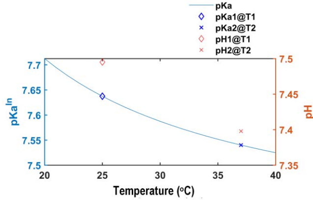
Figure 26. pK_a^{\text{In}} versus temperature. The continuous line is the pK_a estimated using Equation (22). Two randomly measured pHs (at T_1=25 °C and T_2=37 °C ) are also shown.
