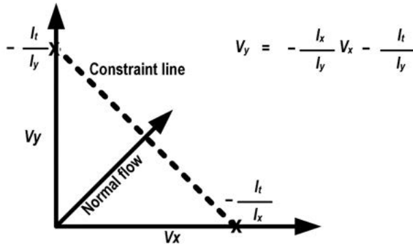
Figure 12. A graphical representation of optical flow constrained equation (Equation (8)). The flow vectors V_x and V_y can be anywhere on the constraint line.
