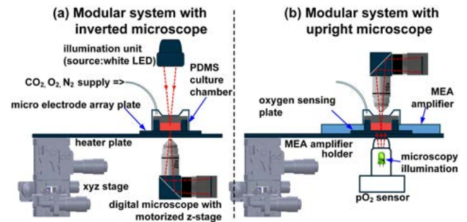
FIGURE 1. Modular microscopy schematic arrangement for (a) inverted microscopy and (b) upright microscopy with optical fluorometric oxygen sensor and MEA amplifier.
