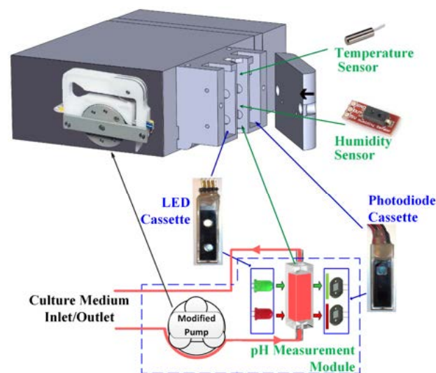
Fig. 1. Modular incubator compatible measurement system. Check [7] for pH sensor module details. Measurement cuvette: 10mm Quartz flow through cuvette (Z804983/Sigma Aldrich). Pump: Modified peristaltic pump (ISM 596/REGLO Digital MS-2/12/IDEX). Temperature sensor: Platinum resistive thermometer (Heraeus 30500109/PT100 in stainless steel housing). Humidity sensor: Thermoset polymer capacitive sensor (HIH-5030/5031/Honeywell-factory calibrated).
