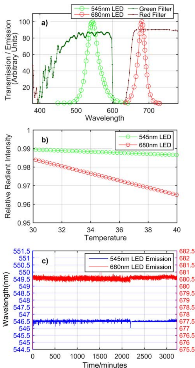
Fig. 2. a) Emission and transmission spectra of green and red LEDs (545-03, 680-02AU/Roithner Laser Technik) and green (Dielectric shortpass FES0600/Thorlabs) and red (Dichroic Red 647 nm LWP/Opticalfiltershop) filter. b) Relative radiant intensity as a function of the temperature for the green and red LEDs in the cassette module. An intensity change of \pm 0.15\% and \pm 1\% need to be expected in green and red channels respectively for \pm 5^\circ\text{C} change around the incubator temperature. c) Spectral stability of the green and red LEDs measured with a spectrometer. The jump seen at \sim 2200 min is when the LEDs were restarted after 2 min pause. Nevertheless, wavelength standard deviation computed is 0.1340 nm and 0.2398 nm for green and red LED, respectively, indicating relatively stable emissive spectral consistency over time.
