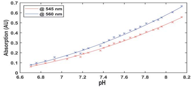
Figure 24. DMEM/F12 absorptions as a function of pH at 545 nm and 560 nm.
