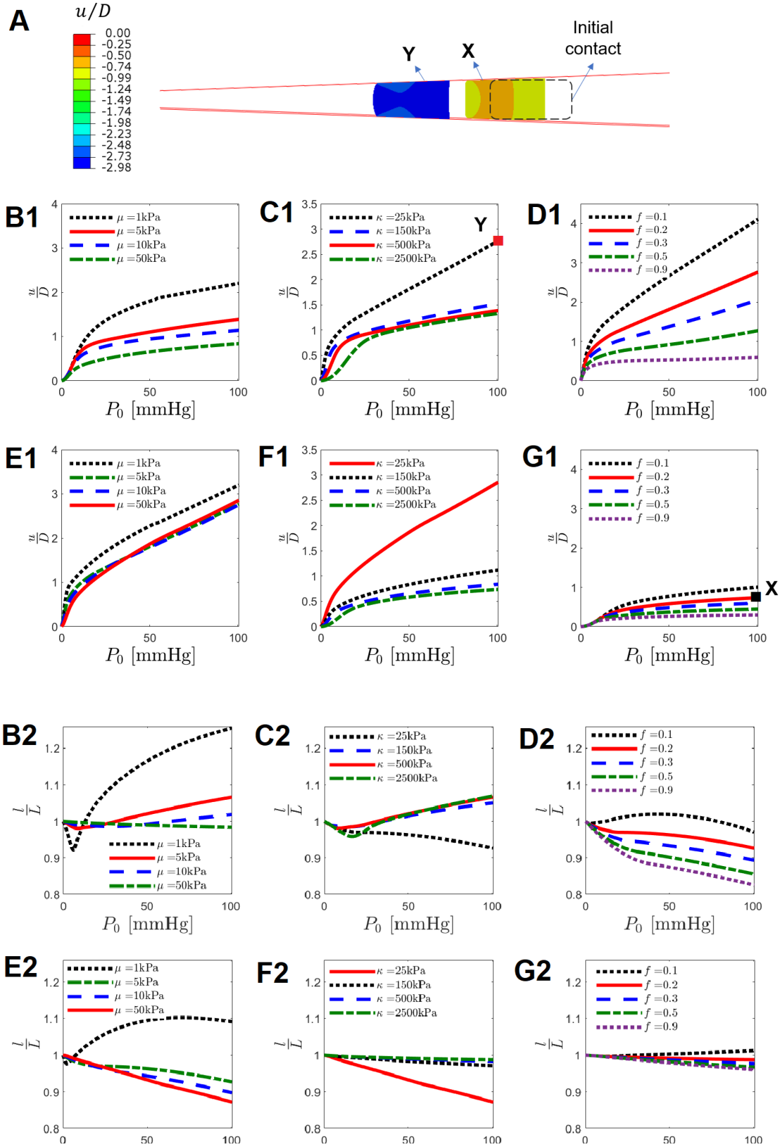
Fig.3: The effects of shear modulus ( \mu ), bulk modulus ( \kappa ), and friction coefficient ( f ) on the occlusion location u in a tapered vessel (B1-G1) and clot length l (B2-G2). The baseline parameters of L/D = 2, P_0 = 100 mmHg, E_1 = E_2 = 0.0844 kPa, D_1 = 0.03, D_2 = 0.08, f = 0.2 and \phi = 2^\circ are used. Also \kappa = 500 kPa, \kappa = 25 kPa have
