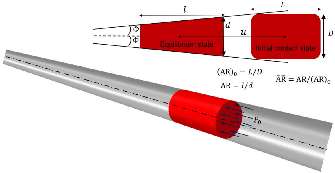
Fig.2: A schematic illustration of the occlusion of a cylindrical blood clot in a tapered vessel. Aspect ratio of clot at initial contact state ((AR)_0) and at equilibrium state (AR) as well as the normalized aspect ratio (\widehat{AR}) are defined.
