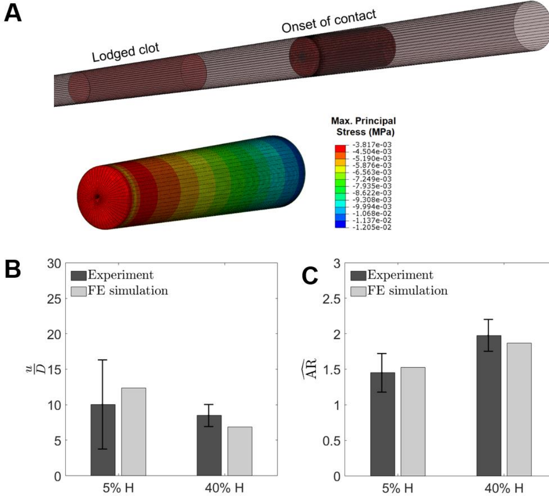
Fig.7: Comparison of in-vitro and FE results for occlusion of the platelet-contracted blood clot analogues in a silicon rubber vessel with taper angle of \Phi = 0.9854^\circ . (A) FE simulation results for the 40% H platelet-contracted clot analogues. (B) The location of clot lodgement ( u/D ) and (C) aspect ratio of clot ( \widehat{AR} ) for 5% H and 40% H clot. The material parameters from Table 1 have been employed. Experimental results reproduced from Johnson et al. (2020a).
