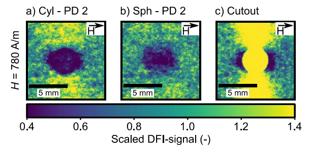
Fig. 4 Scaled DFI of a), Cyl - PD 2, and b), Sph - PD 2, with applied magnetic field strength H of 780 A/m.
