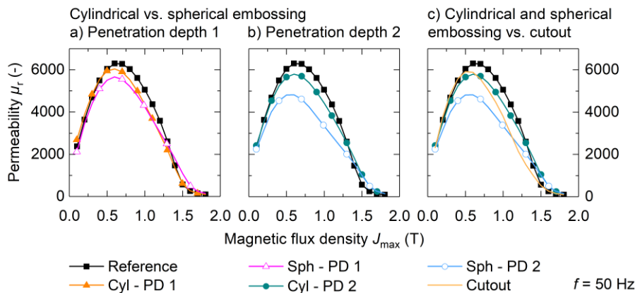
Fig. 8 Magnetic permeability \mu_r of cylindrically and spherically embossed specimen fabricated with a), penetration depth 1, and b), with penetration depth 2, compared to reference material and c), comparison of reference material, cylindrically embossed specimen with a penetration depth of 240 \mu\text{m} , spherically embossed specimen with a penetration depth of 230 \mu\text{m} and flux barrier manufactured as cutout.
