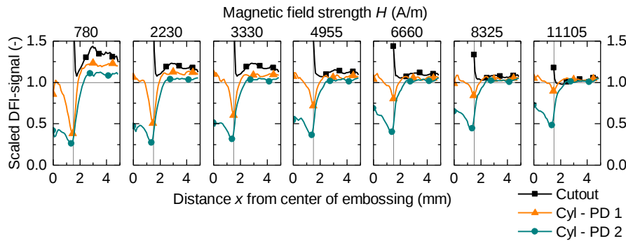
Fig. 5 Scaled DFI-signal of the cylindrically embossed specimens at two different penetration depths compared to a specimen with a cutout (diameter 3.00 mm) as flux barrier measured at different magnetic field strengths H .
