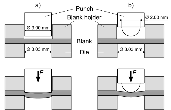
Fig. 2 Schematic illustration of the embossing tool and the embossing of the blank with a) cylindrical punch, and b) spherical punch.
