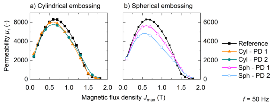
Fig. 7 Magnetic permeability \mu_r for a), cylindrically embossed, and b), spherically embossed specimen, fabricated with two different penetration depths compared to a reference material.
