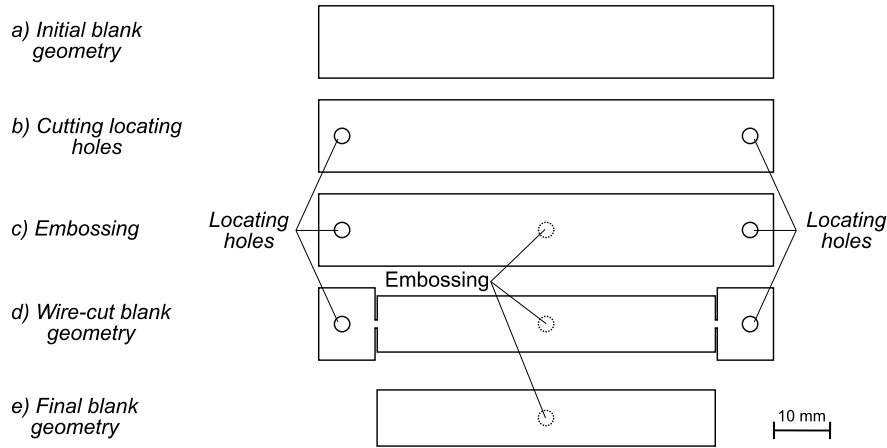
Fig. 1 Schematic illustration of specimen manufacturing: a) initial blank geometry, b) cutting of locating holes, c) embossing of flux barrier, d) wire-cutting and e) final blank geometry.
