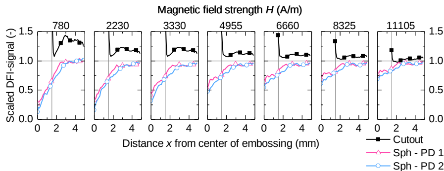
Fig. 6 Scaled DFI-signal of the spherically embossed specimens at two different penetration depths compared to a specimen with a cutout (diameter 3.00 mm) as flux barrier measured at different magnetic field strengths H .
