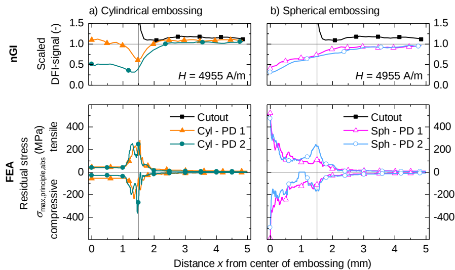
Fig. 9 Comparison of scaled DFI-signal at a magnetic field strength H of 4955 A/m and numerically analyzed residual stress distributions \sigma_{max,principle,abs} of a), cylindrical, and b), spherical embossings.
