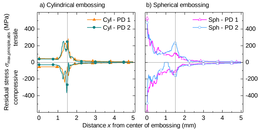
Fig. 3 Numerically analyzed distribution of tensile and compressive residual stress \sigma_{max,principle,abs} plotted to the distance x from center of embossing for a), the cylindrically embossed specimens, and b), the spherically embossed specimens.
