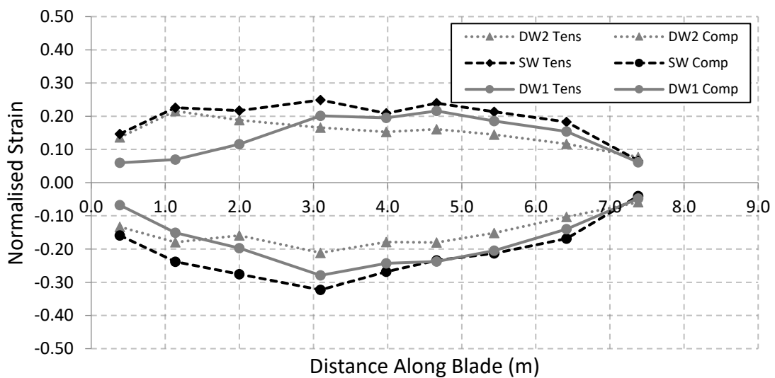
Fig. 5. The longitudinal strain along the blade in the highest loaded biaxial layer in the shear web(s) for both the Single and Double Web designs.
