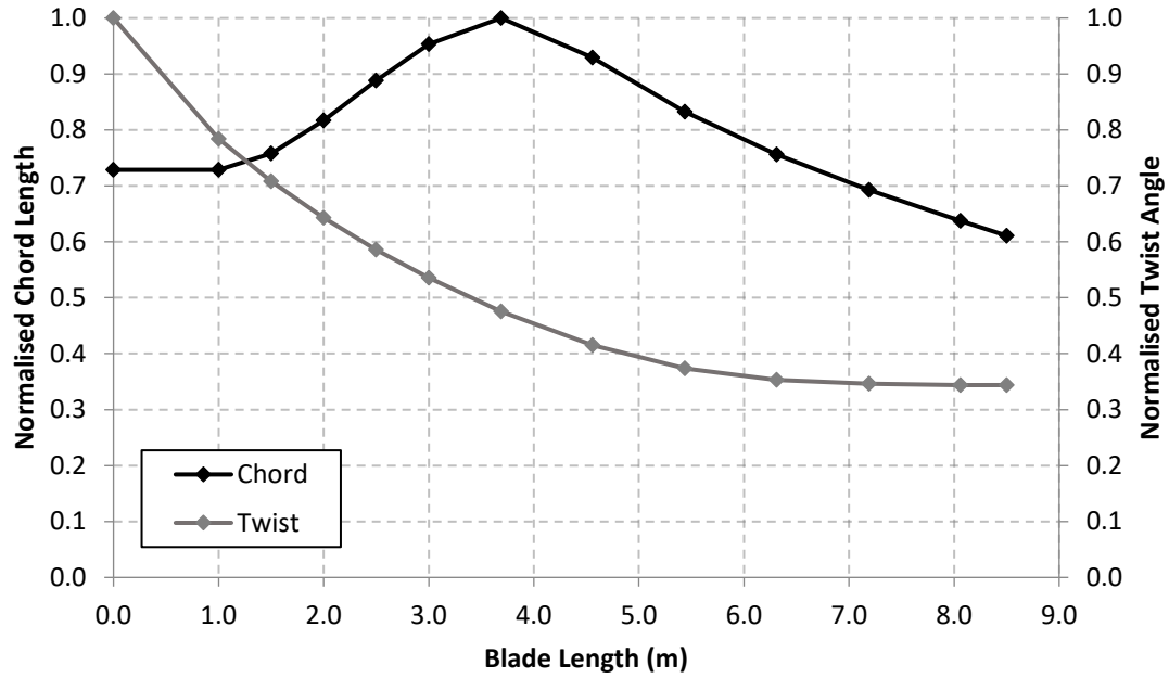
Fig. 1. Chord length and hydrodynamic twist angle distributions along the length of the blade, normalised by the maximum value of each variable.
