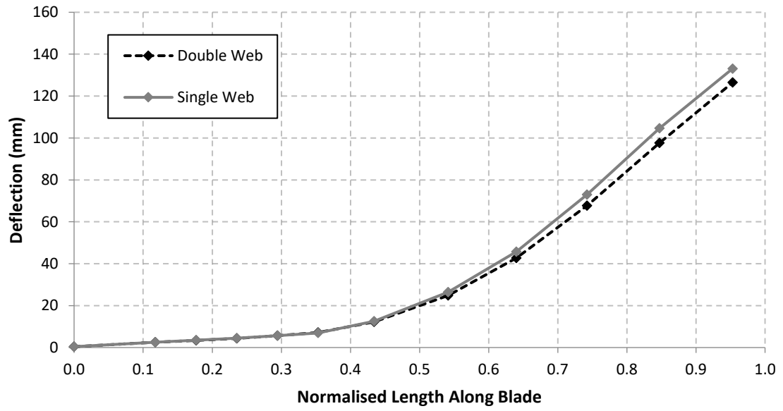
Fig. 6. The resultant deflection of both blade designs.
