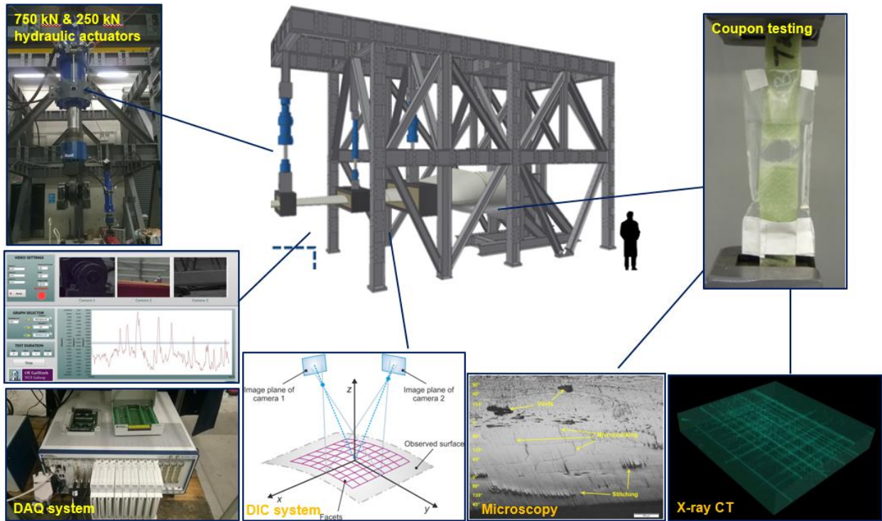
Fig. 8. Testing capabilities of the MaREI Centre's Large Structures Testing Laboratory at the National University of Ireland Galway.
