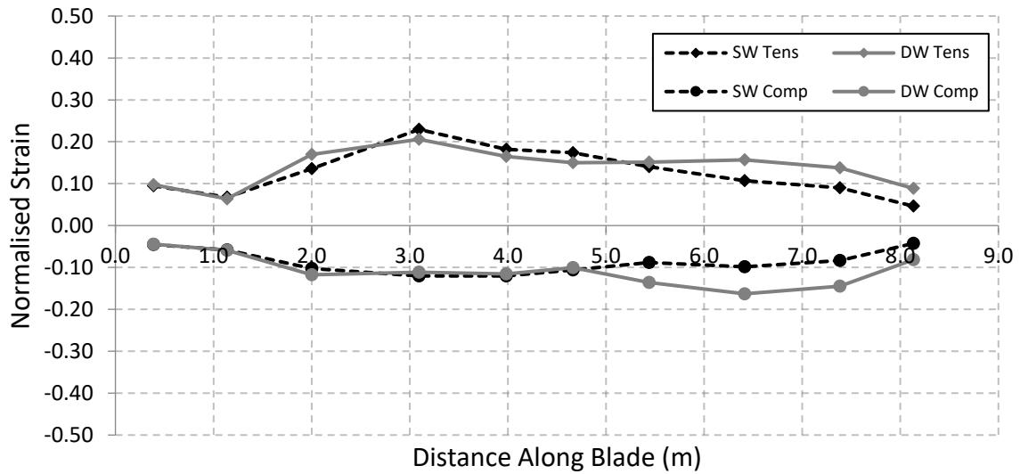
Fig. 4. The maximum longitudinal normalised strain along the blade for (a) the innermost biaxial layer on the pressure side spar cap, (b) the outermost unidirectional layer on the pressure side spar cap, (c) the outermost biaxial layer on the pressure side spar cap.
