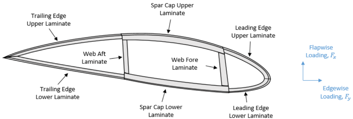
Fig. 3. Naming convention for each region in the blade cross-section.
