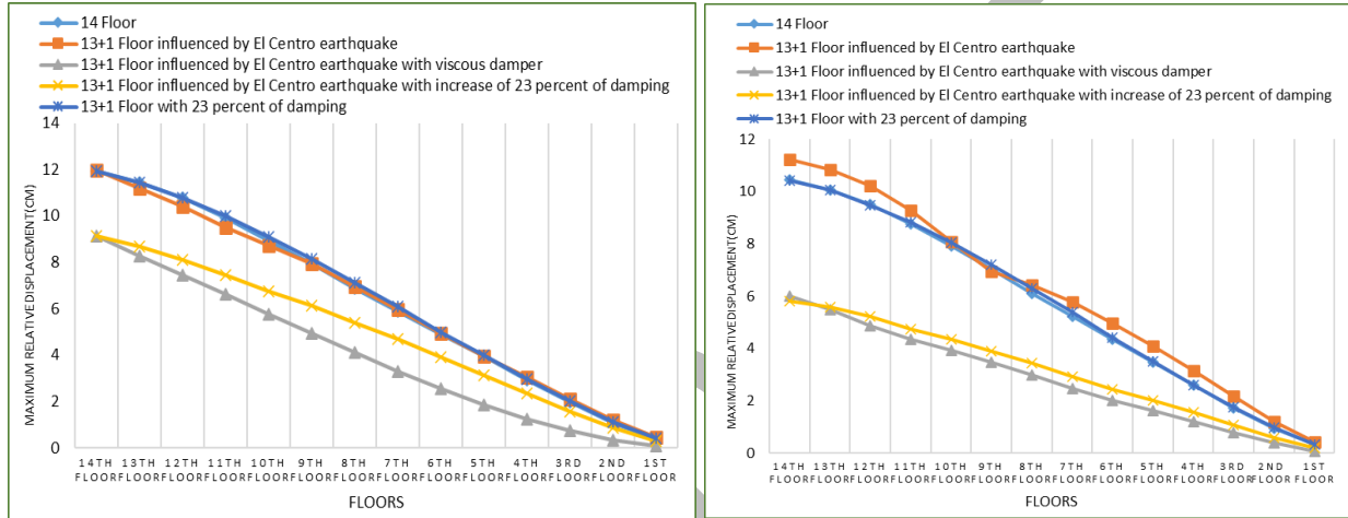
Figure 8. a) Diagram of the maximum displacement of floors in the x-direction, b) the maximum displacement of the floors in the y-direction in different cases in model number three
