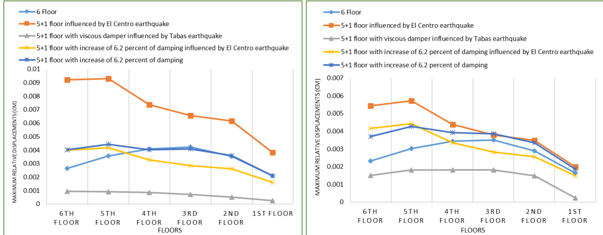
Figure 4. a) Diagram of the relative displacement of the floors in the x-direction, b) the relative displacements of the classes in the y-direction in different cases in different cases in model number 1
