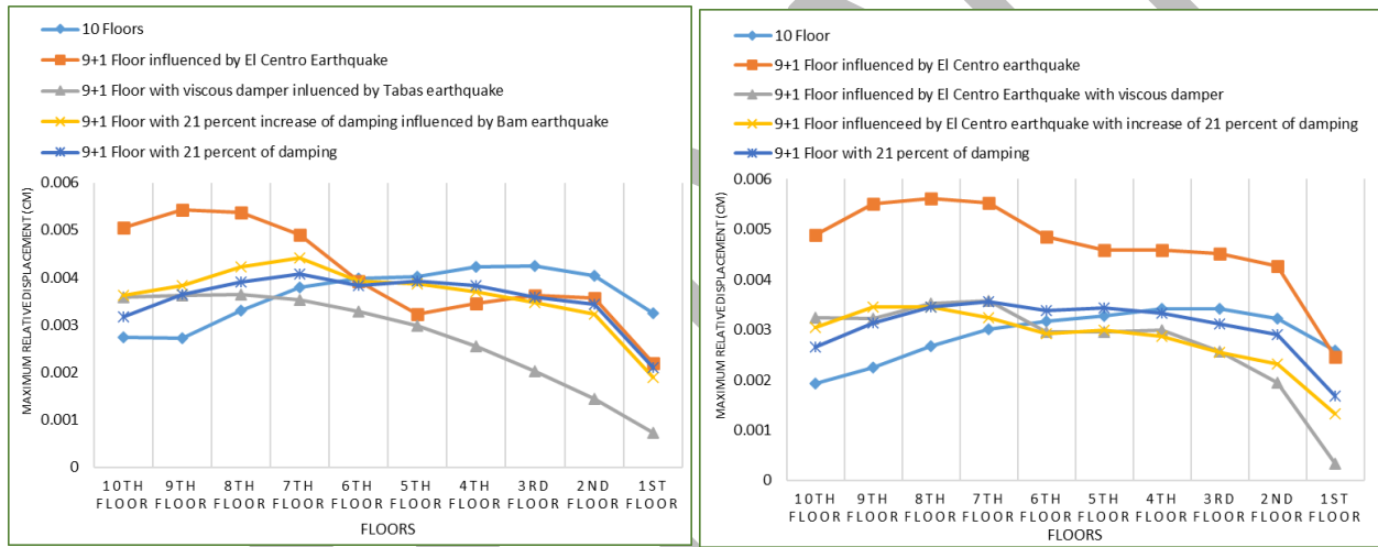
Figure 5. a) Diagram of relative displacement of classes in the x-direction, b) relative displacement of classes in the y-direction in different cases in model number two.
