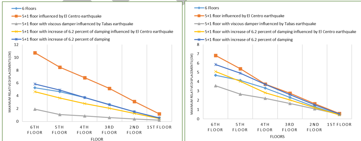
Figure 5. a) Diagram of the maximum displacement of floors in the x-direction, b) the maximum displacement of the floors in the y-direction in different cases in model number one
