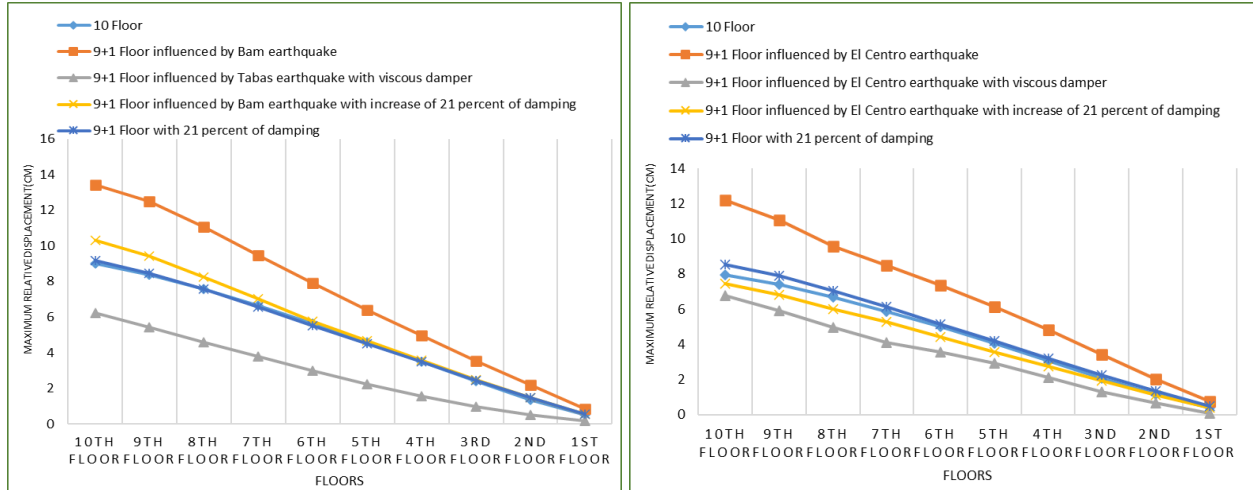
Figure 6. a) Diagram of the maximum displacement of floors in the x-direction, b) the maximum displacement of the floors in the y-direction in different cases in model number two
