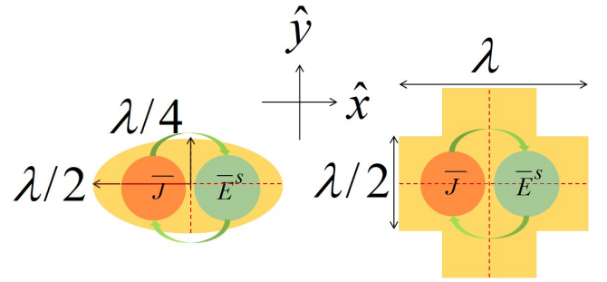
Fig. 1. Planar 2D structures under study: left) an ellipse antenna; and 2) a cross-shaped metasurface. Also shown is the Ping-Pong updating process of the surface current \bar{J} and the scattering electric field \bar{E}^s .
