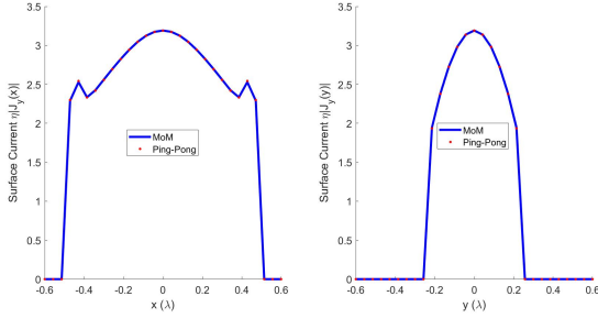
Fig. 4. Comparison of the ellipse antenna's surface current ( \hat{y} component \eta|J_y| ) between our Ping-Pong algorithm and those of the : left) along the \hat{x} direction; and right) along the and \hat{y} direction.
