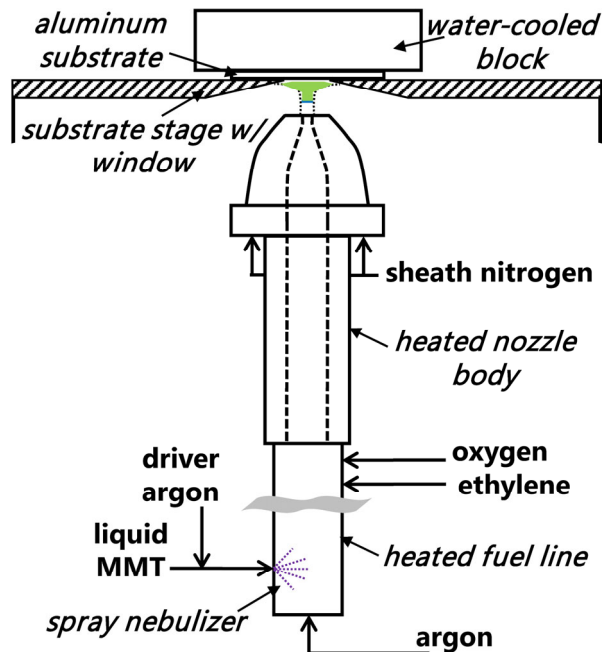
Figure 2 Experimental setup for the flame-assisted deposition process.
