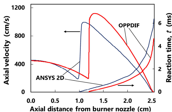
Figure 4 Comparison between typical velocity and reaction time profiles obtained from OPPDIF and ANSYS 2D computations.
