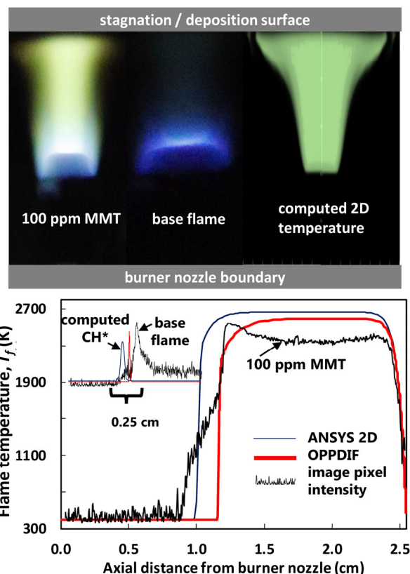
Figure 3 Comparison between measured and computed flame position in terms of flame images (top-left) and 2D temperature contour computed using ANSYS (top-right). Also shown is comparison between centerline temperature profiles (bottom) and CH^* concentration profiles (bottom-inset).
