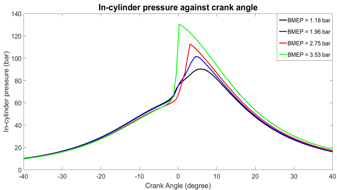
Figure 2. In-cylinder pressure against crank angle at different BMEPs with 2000 rpm engine speed and 300 K intake charge temperature.
