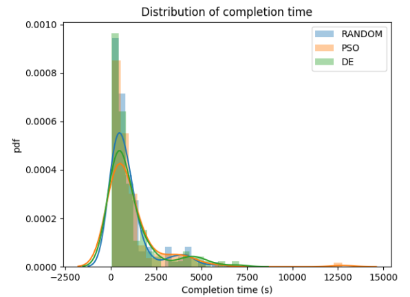
Fig. 5: Probability density functions of Random, DE and PSO
