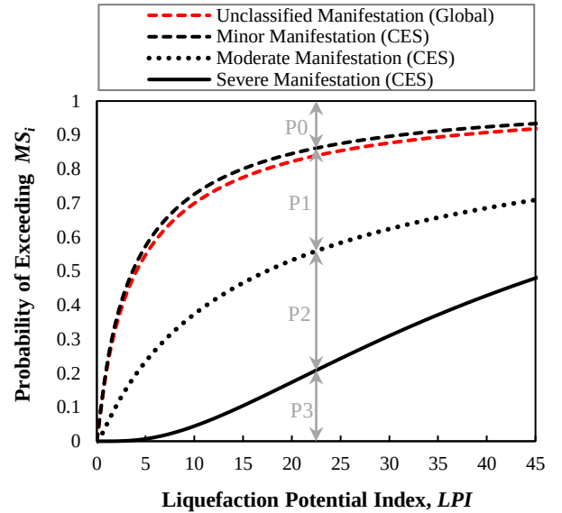
Figure 2. The probability of exceeding manifestation severity, MS_i , given an LPI value computed using the RW98 model. For the CES dataset, P_0 , P_1 , P_2 , and P_3 are the respective probabilities that manifestation severity is none, minor, moderate, and severe.
