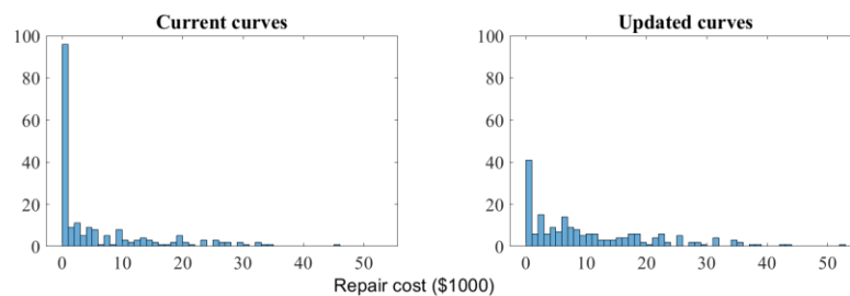
Figure 35. Histograms of repair cost for scenario 1 (CFS-HUD)
