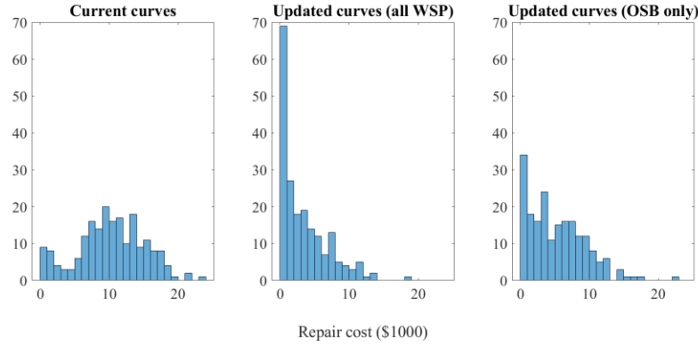
Figure 32. Histograms of repair cost for scenario 2 (CFS-NEES)
