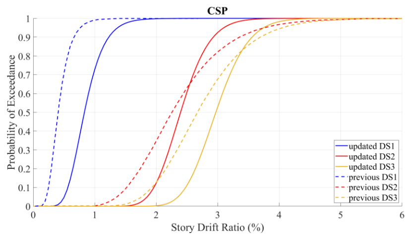
Figure 12. Updated fragility curves for CFS framed walls with CSP sheathing
