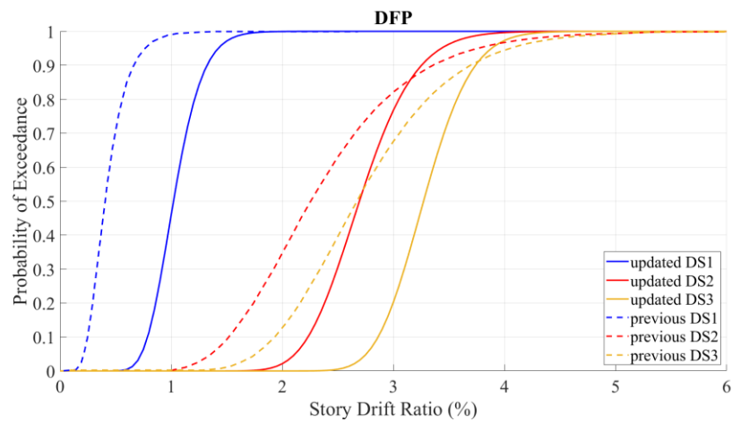
Figure 11. Updated fragility curves for CFS framed walls with DFP sheathing
