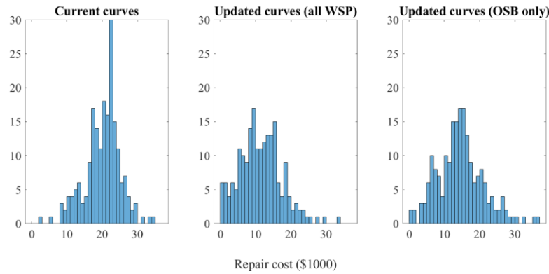
Figure 33. Histograms of repair cost for scenario 3 (CFS-NEES)
