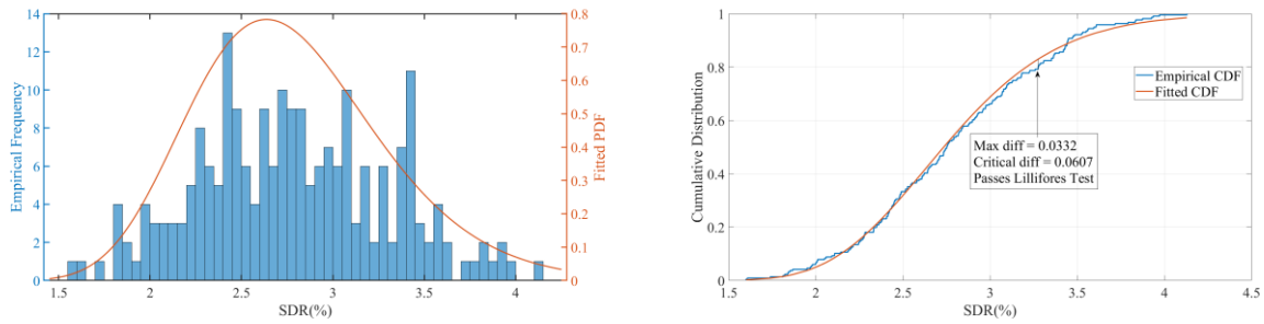
Figure 8. Probabilistic (left) and cumulative distribution (right) corresponding to DS3 for all WSP sheathed walls.
