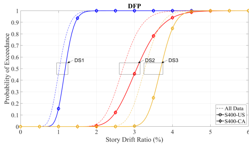
Figure 24. Updated fragility curves for CFS framed walls with DFP sheathing per AISI S400-15
