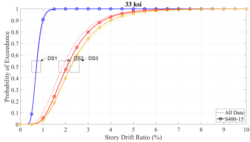
Figure 28. Updated fragility curves for CFS framed walls with X-bracing per AISI S400-15, steel grade: 230 MPa (33 ksi)
