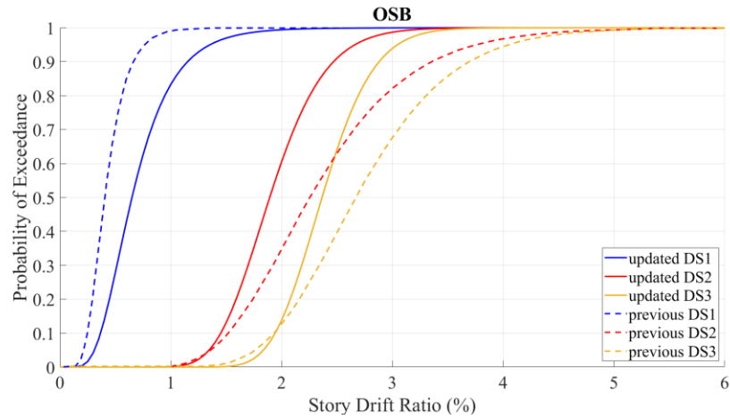
Figure 10. Updated fragility curves for CFS framed walls with OSB sheathing
