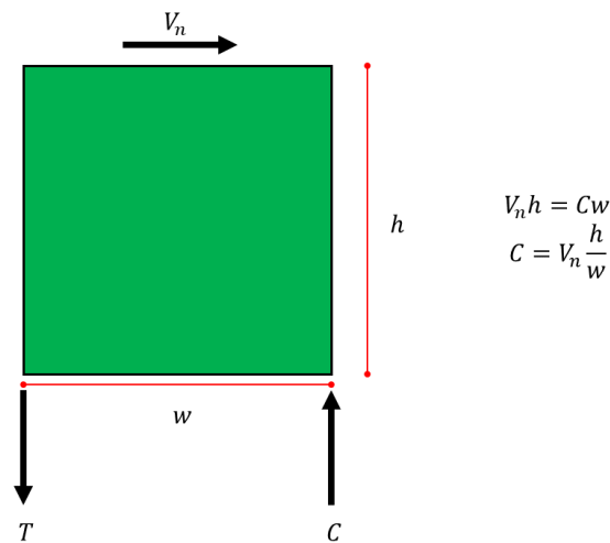
Figure 21. Force diagram of a CFS framed wall under seismic loading
