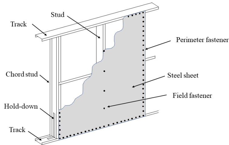
Figure 13. CFS framed shear wall with steel sheet sheathing
