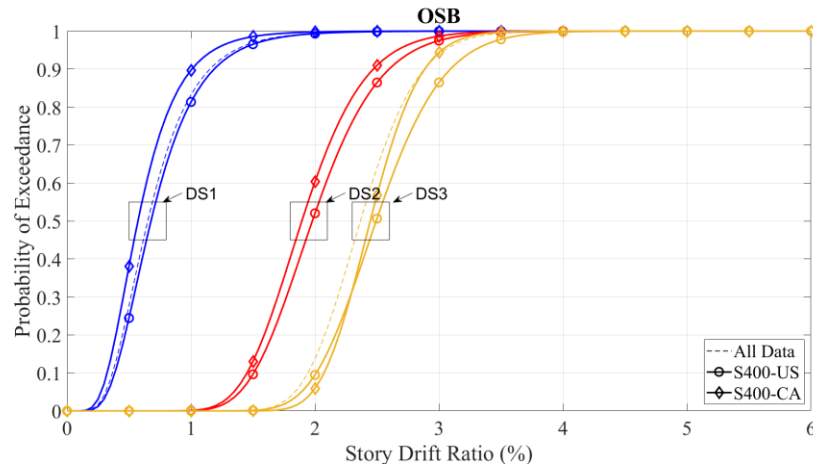
Figure 23. Updated fragility curves for CFS framed walls with OSB sheathing per AISI S400-15
