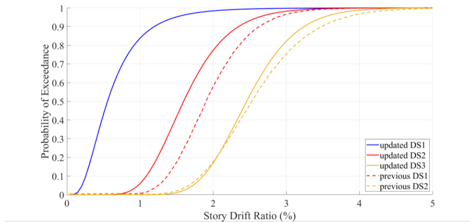
Figure 15. Updated fragility curves for CFS framed walls with steel sheet sheathing
