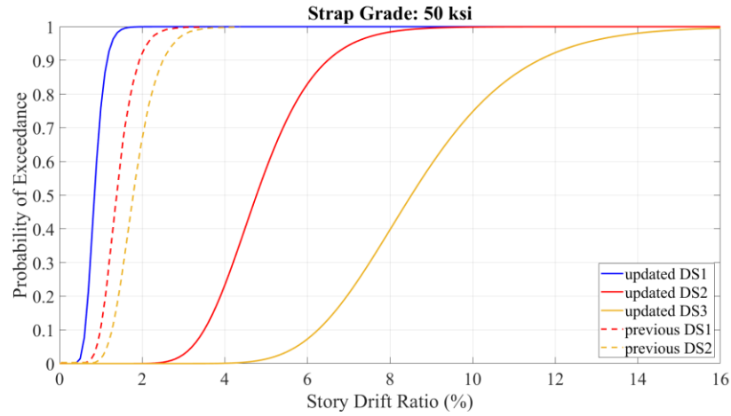
Figure 20. Updated fragility curves for CFS framed walls with X-bracing, steel grade: 345 MPa (50 ksi)
