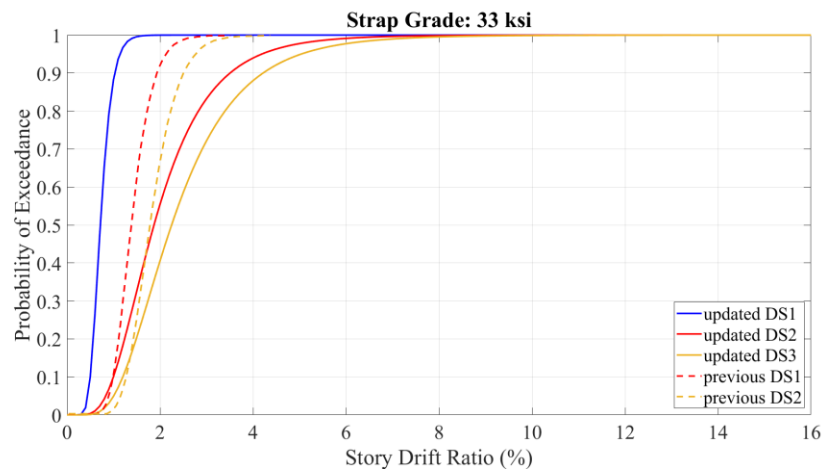
Figure 19. Updated fragility curves for CFS framed walls with X-bracing, steel grade: 230 MPa (33 ksi)
