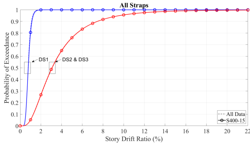
Figure 27. Updated fragility curves for CFS framed walls with flat strap X-bracing per AISI S400-15 (all steel grades inclusive)
