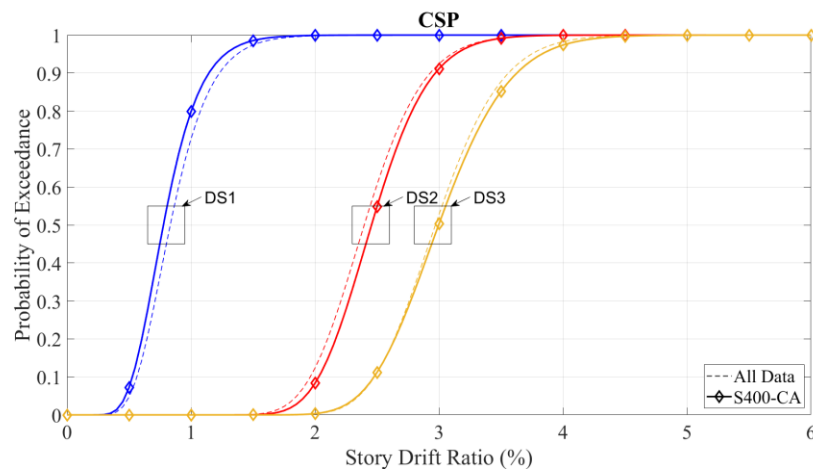
Figure 25. Updated fragility curves for CFS framed walls with CSP sheathing per AISI S400-15
