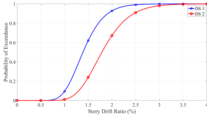
Figure 3. Current fragility curves for walls with flat strap X-bracing
