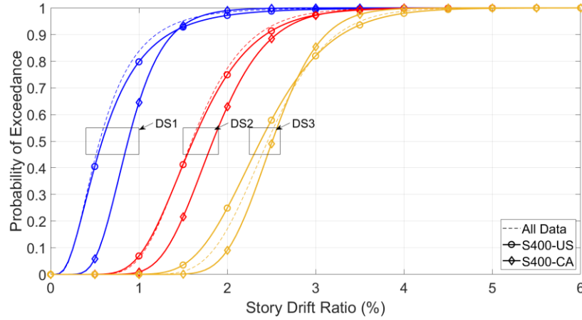
Figure 26. Updated fragility curves for CFS framed walls with steel sheet sheathing per AISI S400-15
