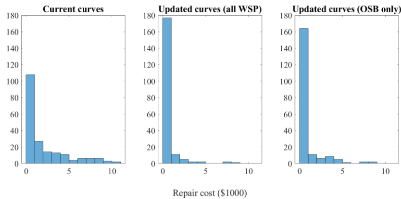
Figure 31. Histograms of repair cost for scenario 1 (CFS-NEES)
