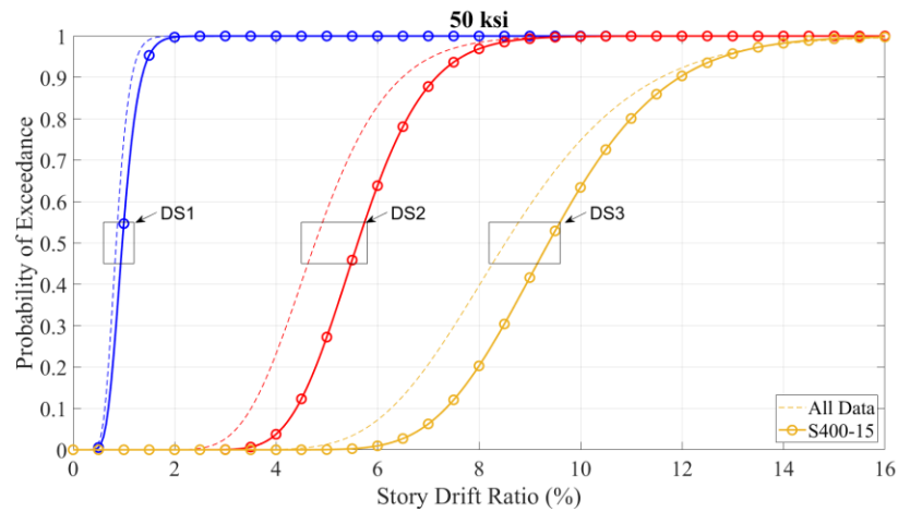
Figure 29. Updated fragility curves for CFS framed walls with X-bracing per AISI S400-15, steel grade: 345 MPa (50 ksi)
