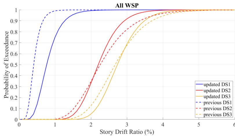
Figure 9. Updated fragility curves for CFS framed walls with all WSP sheathing
