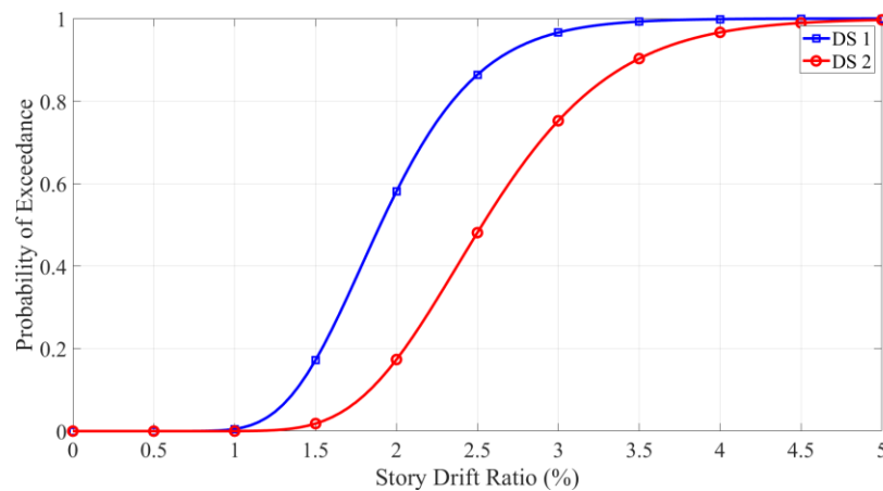
Figure 4. Current fragility curves for walls with steel sheet sheathing
