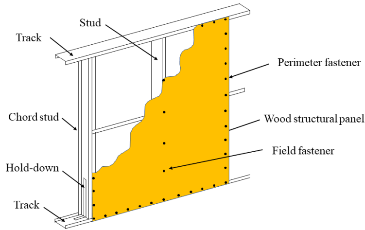
Figure 5. CFS shear wall with WSP sheathing
