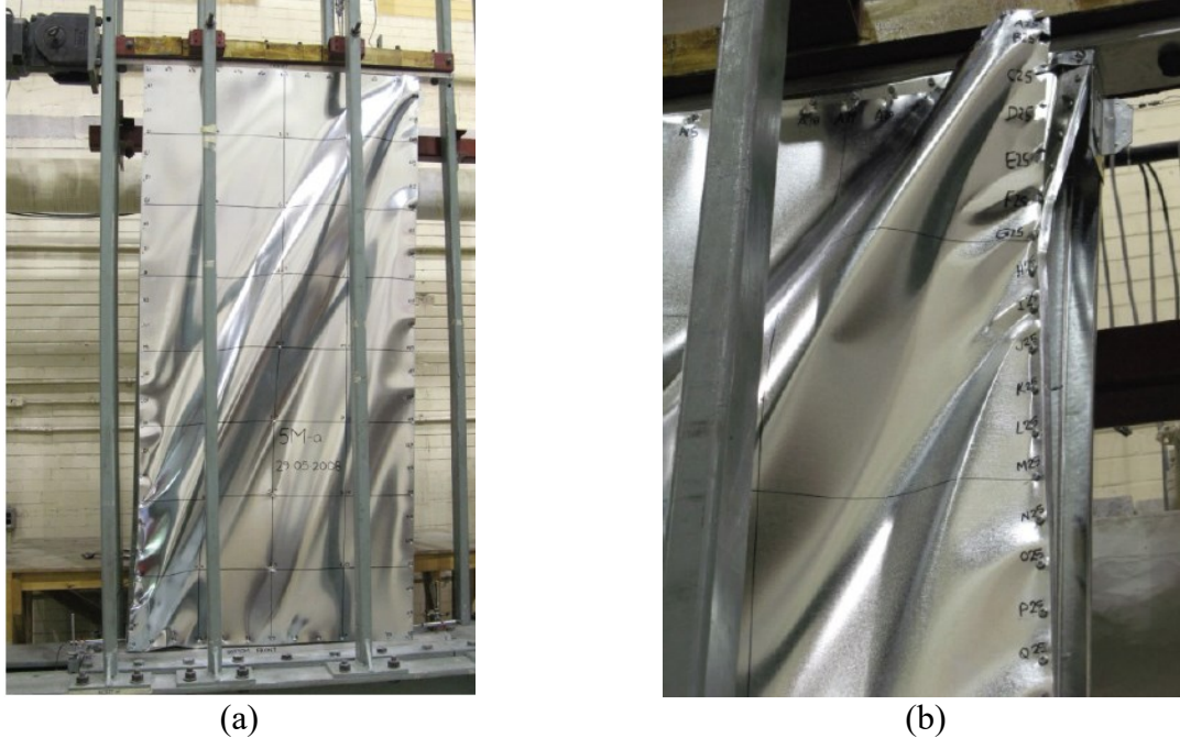
Figure 14. Examples of failure modes of walls with steel sheet sheathing: (a) buckling of steel sheet; (b) twisting of stud (image source: [11])
