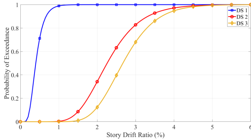
Figure 2. Current fragility curves for walls with WSP sheathing
