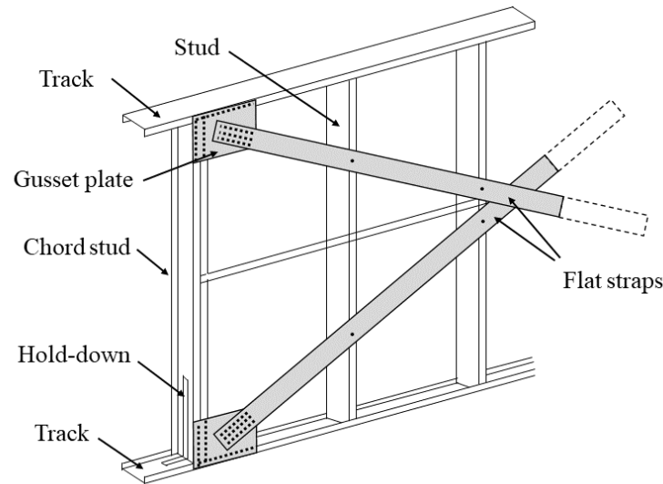
Figure 16. CFS framed shear wall with flat strap X-bracing (fastened detail shown, welded gusset plates and strap is also common)
