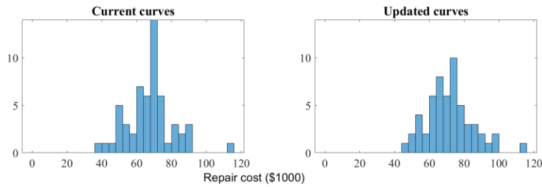
Figure 37. Histograms of repair cost for scenario 3, excluding collapse cases (CFS-HUD)
