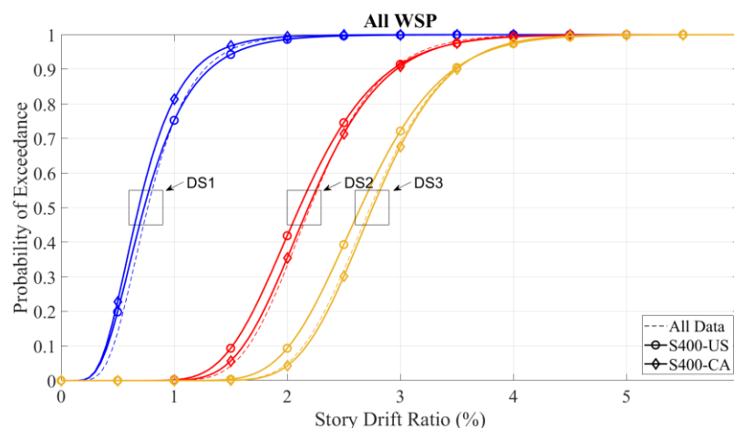
Figure 22. Updated fragility curves for CFS framed walls with all WSP sheathing per AISI S400-15
