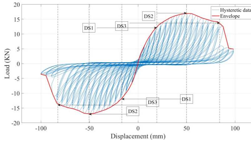
Figure 7. Example of damage states for a test specimen
