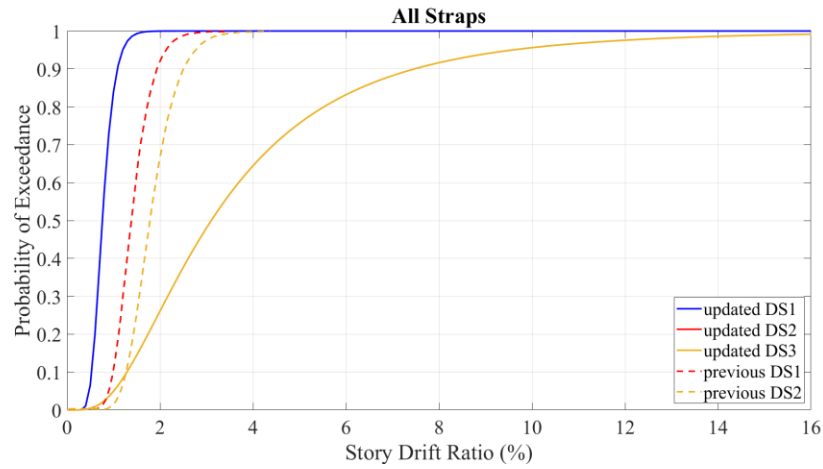
Figure 18. Updated fragility curves for CFS framed walls with X-bracing (all steel grades inclusive)
