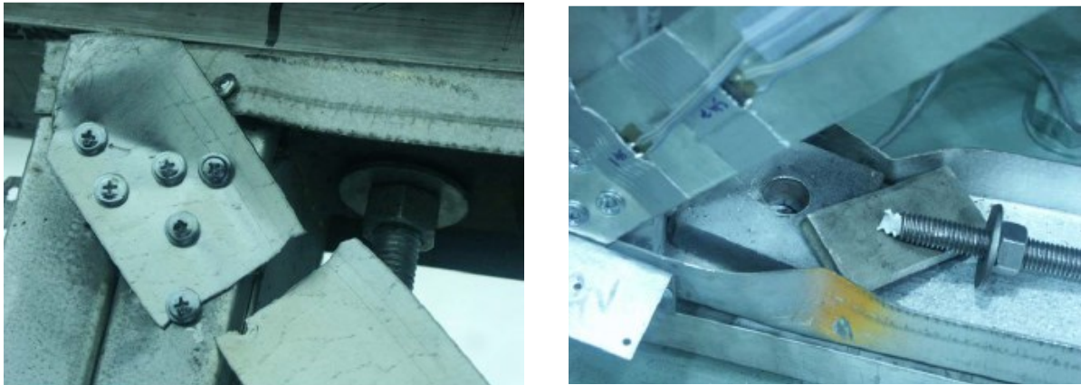
Figure 17. Potential undesirable failure modes in flat strapped shear walls: (a) improperly detailed connection leading to net section failure; (b) improperly sized rod leading to anchorage failure (image source: [23])
