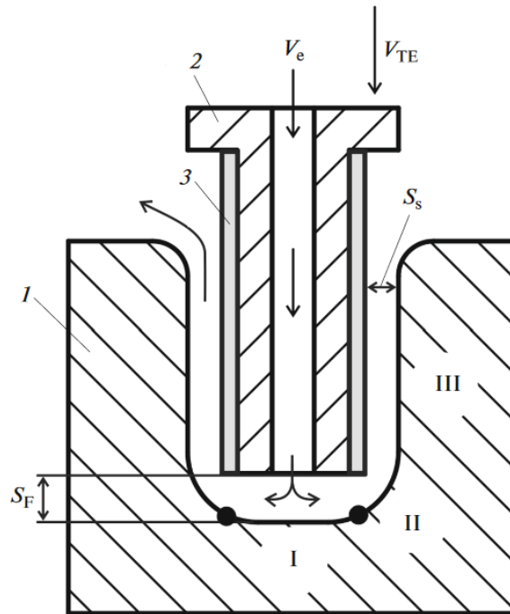
Figure 3: Scheme of ECM of workpiece (1) by tubular tool-electrode (2) with insulated side surface (3). The arrow at VTE shows the direction of TE feed, the arrows from Ve show the direction of electrolyte flow, SF is the end face inter electrode gap, Ss is the side inter electrode gap, I denotes the machining zone (working zone), II denotes area adjacent to the working zone, and III denotes the zone of passive titanium Davydov et al. (2017) .
