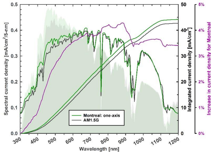
Fig. 4. Current densities for the silicon cell derived from its quantum efficiency combined with spectral irradiances for the standard spectrum (AM1.5G) and the annual global spectrum for single-axis tracking in Montreal. The purple line indicates the relative increase in integrated current density for Montreal with respect to AM1.5G. Spectral irradiances in the background are not shown to scale.
