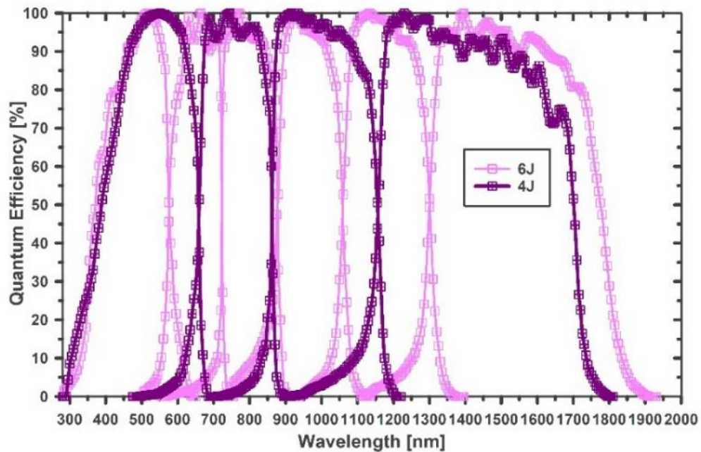
Fig. S3. Quantum efficiencies of the III-V four- and six-junction cells.
