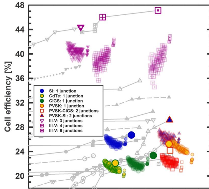
Fig. S4. Efficiencies under operating spectra and temperatures.
