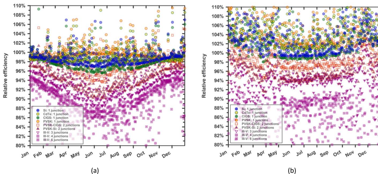
Fig. 7. Daily relative efficiencies at 25° C for Alamosa, USA (latitude-tilt) and Montreal, Canada (one-axis tracking). Results for other sites are in Supplemental Table S4.
