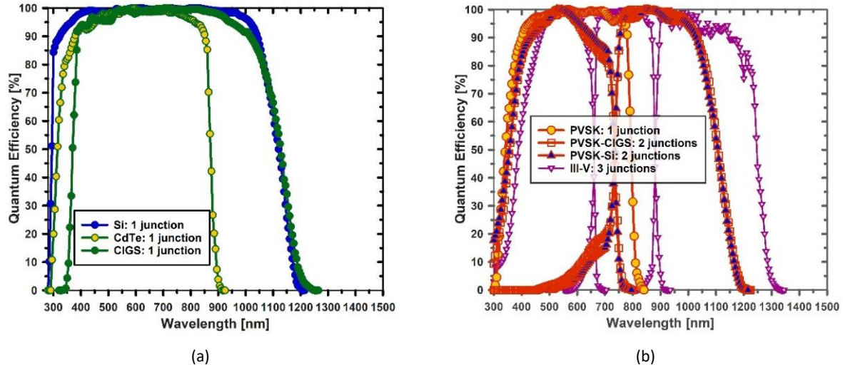
Fig. 3. Quantum efficiencies for seven of the nine cell types in this study, digitized at 5-nm intervals from figures in the Solar Cell Efficiency Tables : (a) silicon (Si) 37 , cadmium telluride (CdTe) 38 , and CIGS 39 ; (b) perovskite (PVSK) 40 , perovskite-CIGS tandem (PVSK-CIGS) 41 , perovskite-silicon tandem (PVSK-Si) 41 and a III-V three-junction cell 42 . The quantum efficiencies for the III-V four-junction and III-V six-junction cells are shown in Supplemental Fig. S3.
