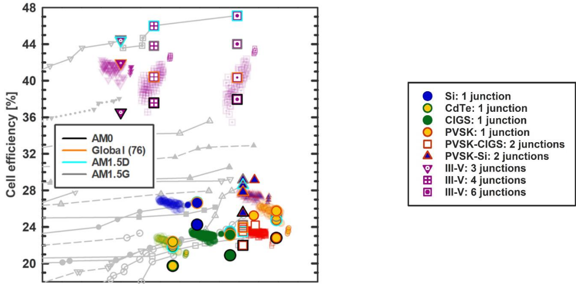
Fig. S5. Efficiencies under operating spectra (at 25° C), AM1.5G, AM1.5D, and AM0. Some lateral positions are adjusted to improve visibility.
