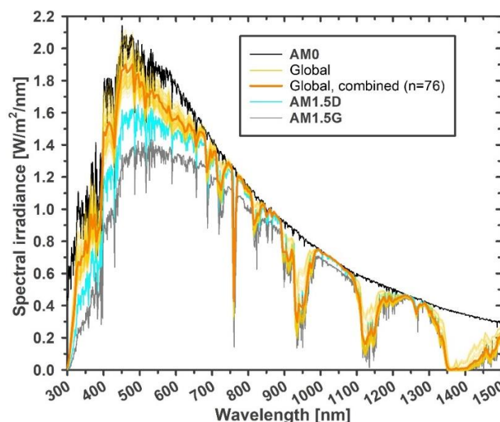
Fig. S1. Three standard spectra (AM0, AM1.5D, and AM1.5G) compared against seventy-six annual global spectra (one-axis and latitude-tilt) derived from the National Solar Radiation Database (NSRDB) hourly spectra, converted to 5-nm wavelength intervals. The NSRDB global spectra are normalized to the AM0 value at 1050 nm.
