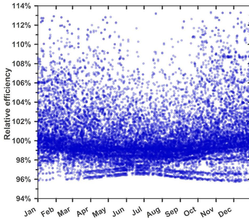
Fig. S7. Variation of a silicon cell under the global spectra compiled for sites in Table S4 (25° C).
