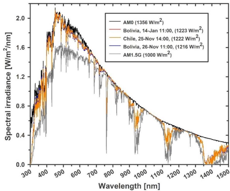
Fig. S8. The three highest hourly irradiances in the data, obtained for Uyuni, Bolivia and Putre, Chile. Amplitudes are normalized to AM0 at 1050 nm.
