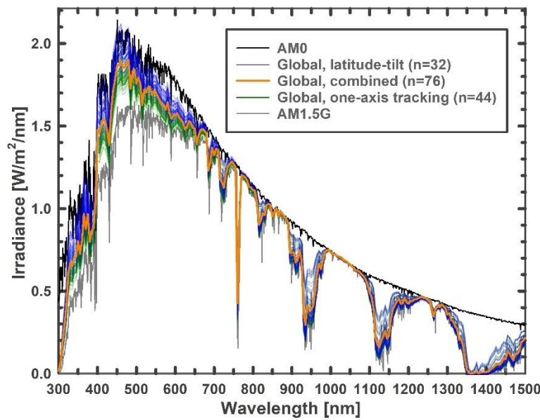
Fig. 2. Annual summations of seventy-six hourly global spectra from forty-five locations for NSRDB spectrum year 2018. For comparison with AM1.5G (gray) and the extraterrestrial standard (AM0, black), the global spectra amplitudes have been normalized to that of AM0 at 1050 nm.
