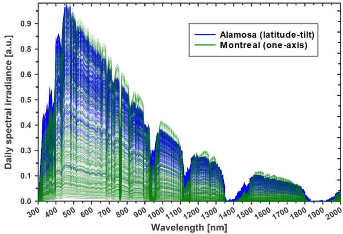
Fig. S2. Daily spectral irradiances for Alamosa (latitude-tilt) and Montreal (one-axis tracking). Amplitudes are normalized to the peak at each respective location.
