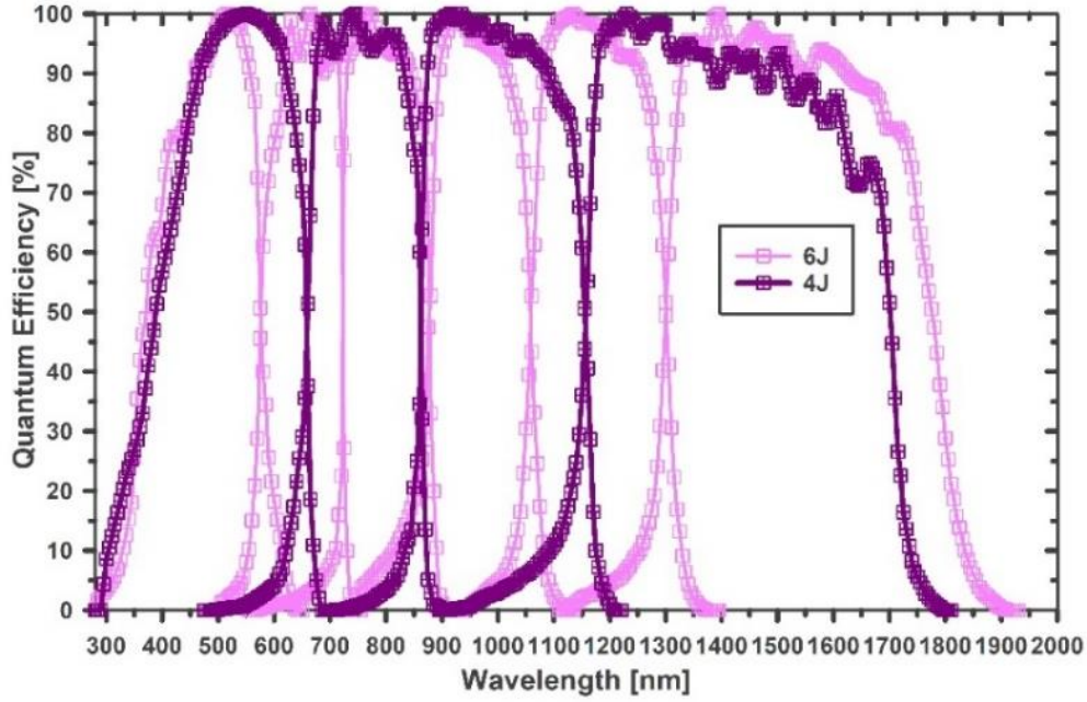
Fig. S3. Quantum efficiencies of the III-V four- 38 and six-junction 39 cells.
