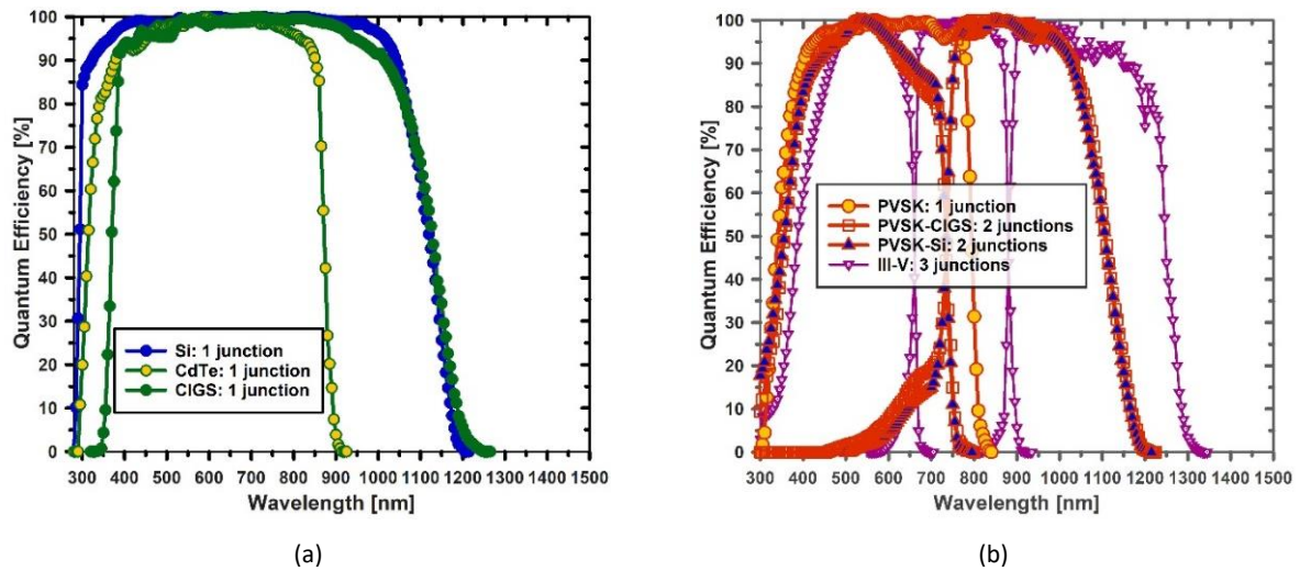
Fig. 3. Quantum efficiencies for seven of the nine cell types in this study, digitized at 5-nm intervals from figures in the Solar Cell Efficiency Tables : (a) silicon (Si) 37 , cadmium telluride (CdTe) 38 , and CIGS 39 ; (b) perovskite (PVSK) 40 , perovskite-CIGS tandem (PVSK-CIGS) 41 , perovskite-silicon tandem (PVSK-Si) 41 and a III-V three-junction cell 42 . The quantum efficiencies for the III-V four-junction and III-V six-junction cells are shown in Supplemental Fig. S3.
