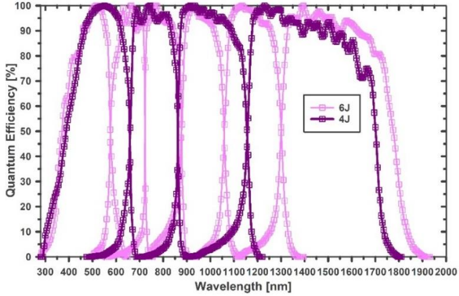
Fig. S3. Quantum efficiencies of the III-V four 39 and six-junction 40 cells.
