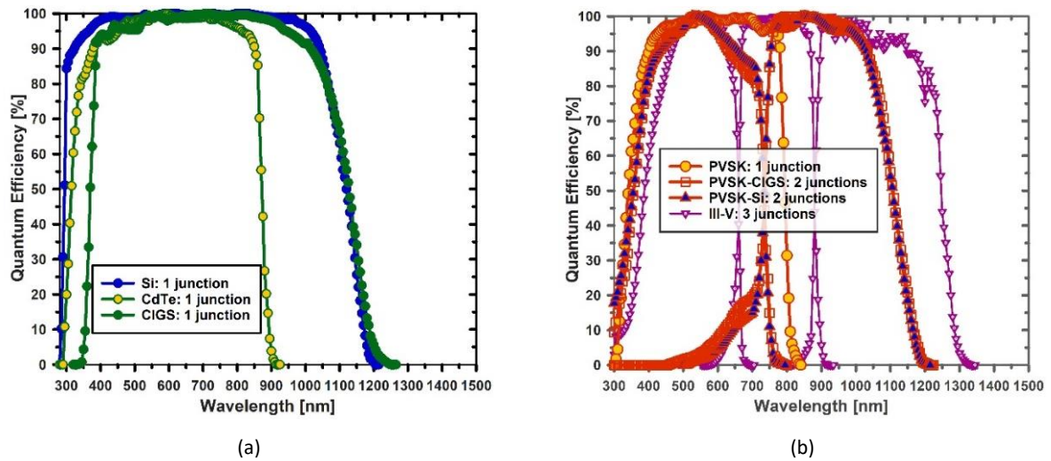
Fig. 3. Quantum efficiencies for seven of the nine cell types in this study, digitized at 5-nm intervals from figures in the Solar Cell Efficiency Tables : (a) silicon (Si) 38 , cadmium telluride (CdTe) 39 , and CIGS 40 ; (b) perovskite (PVSK) 41 , perovskite-CIGS tandem (PVSK-CIGS) 42 , perovskite-silicon tandem (PVSK-Si) 42 and a III-V three-junction cell 43 . The quantum efficiencies for the III-V four-junction and III-V six-junction cells are shown in Supplemental Fig. S3.
