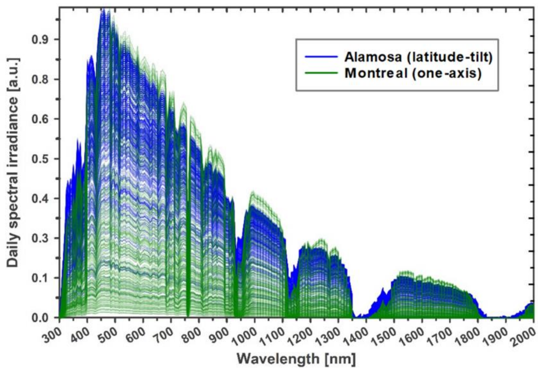
Fig. S2-1. Daily spectral irradiances for Alamosa (latitude-tilt) and Montreal (one-axis tracking). Amplitudes are normalized to the peak at each respective location.
