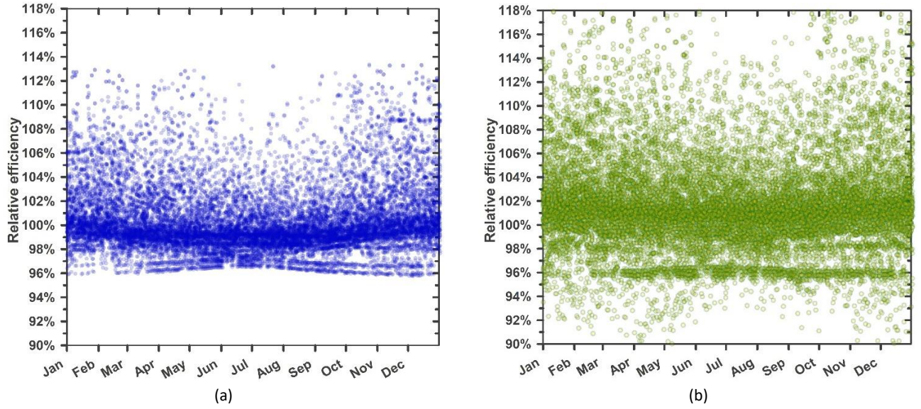
Fig. S7. Daily relative efficiencies of (a) silicon and (b) cadmium telluride cells under global operating spectra (25° C) for the sites in Table S4.
