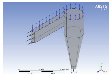
Fig. 12. Boundary conditions for flow simulation without runner
