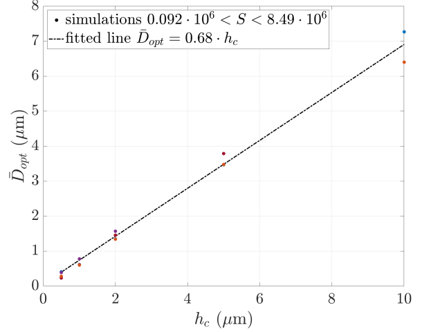
Figure 14: Average dimple depth as function of the gap height. Each point represent a different combinations of velocity and viscosity so that the following range of Sommerfeld number is swept: 0.092 \cdot 10^6 < S < 8.49 \cdot 10^6 . The simulations are carried out at constant gap height.
