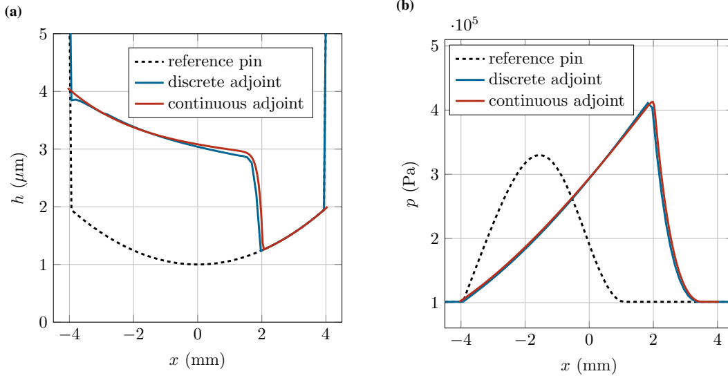
Figure 6: Validation of the discrete and continuous adjoint implementations with the geometry of the parabolic pin in presence of cavitation. a, Comparison between the continuous and the discrete adjoint methods for pin with parabolic shape. The parabola is 1 \mu\text{m} high as well as the gap height at the center. b, Comparison of the pressure profile in the centerline of the pin. The comparison is carried out with the following operating parameters for both figures: U = 0.1 \text{ m/s} , \mu = 0.0028 \text{ Pa}\cdot\text{s} , P_{\text{cav}} = P_{\text{in}} = 101325 \text{ Pa} .
