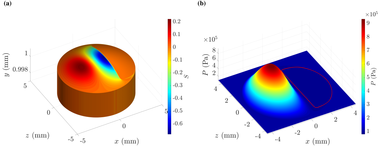
Figure 7: Analysis of the reference untextured pin. a, Sensitivity over the pin geometry at the first optimization step. A positive sensitivity implies that the gap height should be increased in order to achieve a higher load carrying capacity. The vertical y axis is 1000 magnified in comparison to the other two ones. b, Pressure distribution of the parabolic pin. The cavitation region is delimited by a red line. The lubricant fluid flows from left to right in the x direction.
