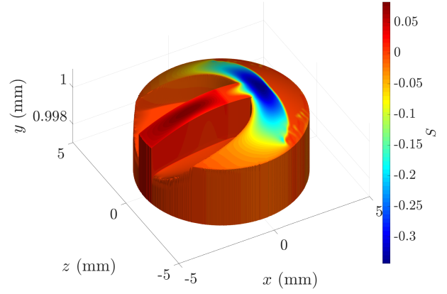
Figure 10: Sensitivity over the optimized pin geometry with the additional constraint which eases the effective texturation on a real pin-on-disc tribometer. The central stripe has a width of 30% of the pin radius. The vertical y axis is 1000 magnified in comparison to the other two ones.
