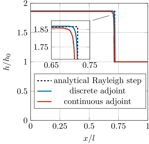
Figure 3: Validation of the adjoint implementation with analytical and direct methods. Comparison between the analytical solution of the 1D Rayleigh step and the solution of the discrete and continuous adjoint method. The curves are non dimensionalized. The inlet pressure is set equal to the outlet one.
