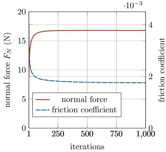
Figure 9: Convergence of the normal force and of the friction coefficient during the optimization iterations. The simulations are stopped as soon as the residual on the gap height variation \bar{h} drops below 10^{-5} .
