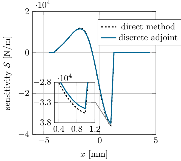
Figure 5: Validation of the adjoint implementation with analytical and direct methods. Sensitivity in the centerline at the first iteration step for the a pin with parabolic shape. The sensitivity is shown with its dimensional value [N/m] since it relates the variation of the normal force (object function) to a variation in the geometry.
