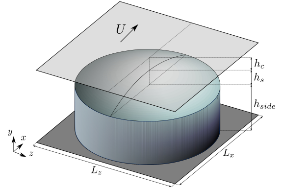
Figure 4: Schematic representation of the pin geometry in a pin-on-disc tribometer. The pin has a parabolic profile whose height at the center is h_s , while the minimum gap height at the center of the geometry is h_c . The side of the pin h_{side} is 1 mm high. The domain is size is L_x and L_z in the x - and z -direction respectively.
