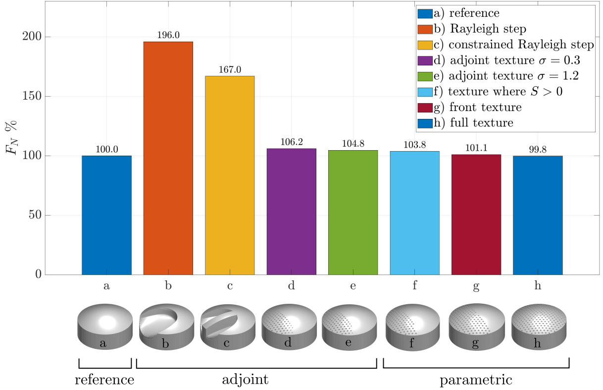
Figure 13: Performance of the adjoint optimization for different constraints. The figure shows also the comparison with parametric studies for textured surfaces done in this work. The normal force is displayed as percentage of the untextured case a. The operating parameters of this comparison are reported in Table 1.
