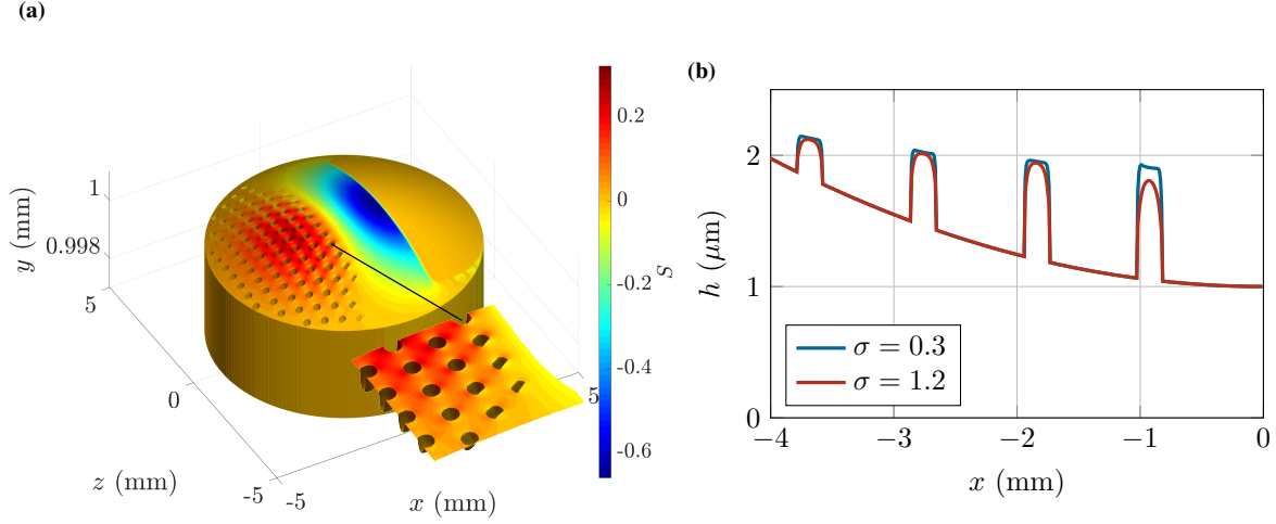
Figure 12: Analysis of the impact of the smoothing amplitude \sigma . a, Sensitivity over the pin geometry. With high smoothing amplitude \sigma = 1.2 . The vertical y axis is 1000 magnified in comparison to the other two ones. b, Comparison of the centerline gap height for different values of smoothing amplitude \sigma . The gap height is 1000 magnified in comparison to length of the pin.
