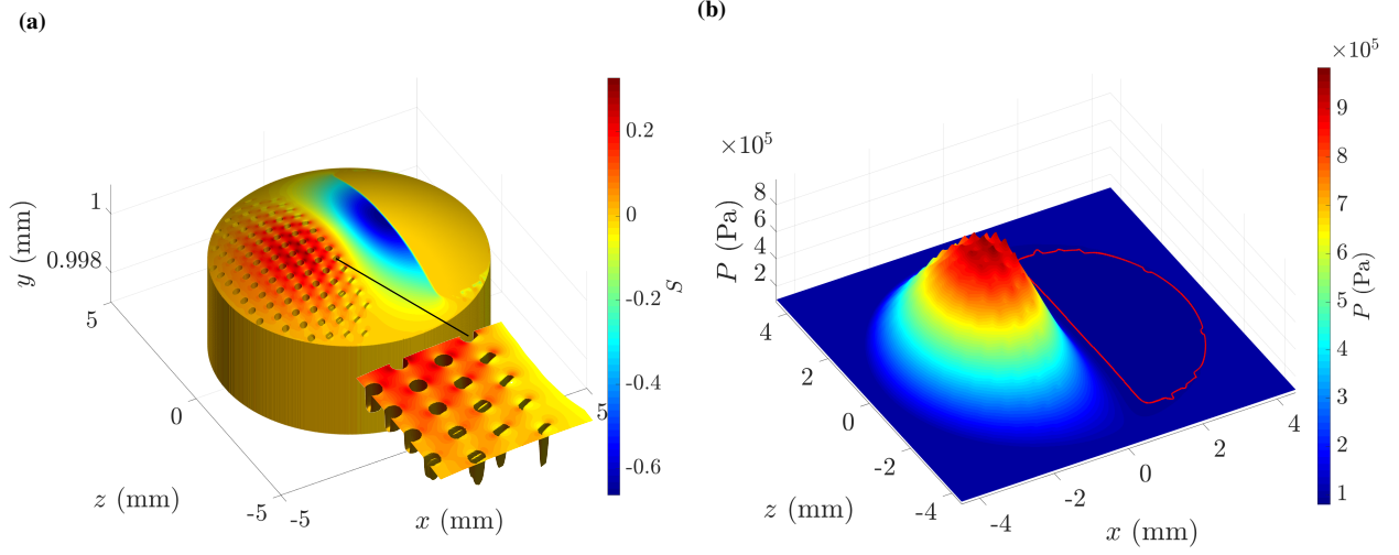
Figure 11: Optimization of texture on the pin surface. The texture has a pseudo-hexagonal pattern and the dimples are constrained to have a maximal diameter D = 200 \mu\text{m} . a, Sensitivity over the textured pin surface with low smoothing amplitude \sigma = 0.3 . The vertical y axis is 1000 magnified in comparison to the other two ones. b, Pressure distribution. The cavitation region is delimited by a red line.
