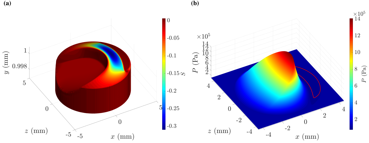
Figure 8: Optimized pin geometry and pressure distribution with the 2D Rayleigh step. The optimization has the only constraint that the gap height cannot be reduced as stated in equation 21. a, Geometry of the optimized 2D Rayleigh step. The sensitivity is plotted over the surface of the pin. The vertical y axis is 1000 magnified in comparison to the other two ones. b, Pressure distribution over the optimized 2D Rayleigh step. The cavitation region is delimited by a red line. The lubricant fluid flows from left to right in the x direction
