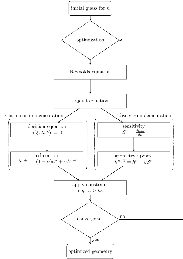
Figure 2: Flowchart of the optimization process. The computation of the sensitivity and of the update of the gap height are presented for both the continuous as well as the discrete implementation.
