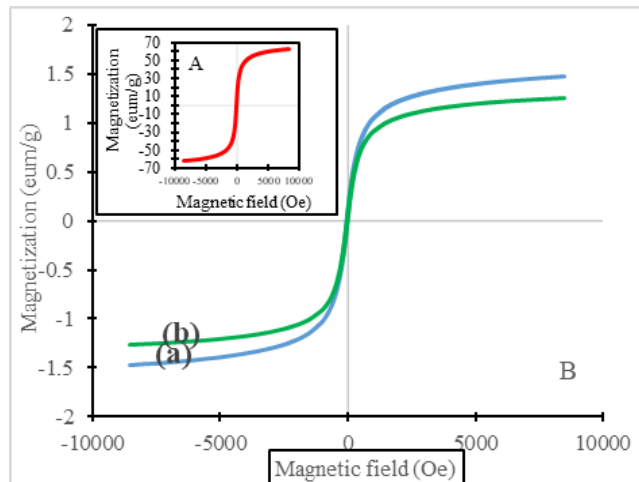
FIGURE 7. Comparison of hysteresis curves of A) \text{Fe}_3\text{O}_4 and B) (a) \text{Fe}_3\text{O}_4/\text{TiO}_2 and (b) \text{Fe}_3\text{O}_4/\text{TiO}_2/\text{Ag}
