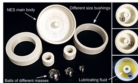
Exploded view for NES part
