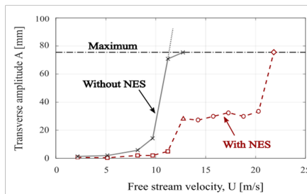
Prism response with and without the NES
