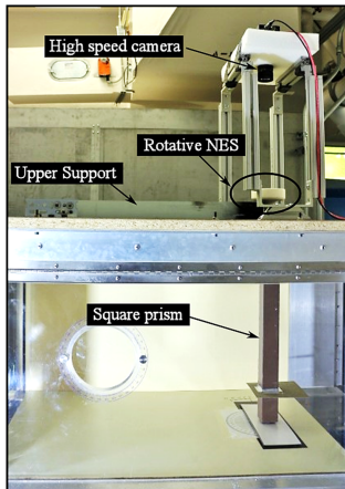
Experimental Setup
