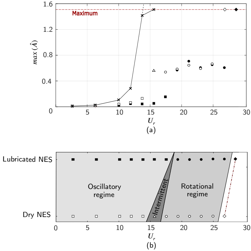
Figure 10: (a) Prism responses without \times and with a dry (white marks) and lubricated (black marks) NESs with the same mass and radius ratios \hat{m} = 0.08 , \hat{r} = 0.6 , (b) NES regimes mapping presenting oscillatory \square , Intermittent \triangle , and Rotational \circ regimes, and the points that reach the maximum allowed amplitude \diamond .
