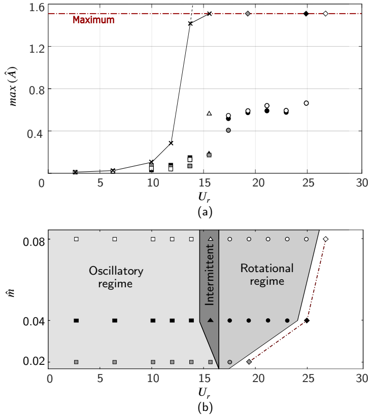
Figure 8: (a) Prism responses without \times and with a NES of mass ratio \hat{m} = 0.02 (grey marks), \hat{m} = 0.04 (black marks), and \hat{m} = 0.08 (white marks) at a constant \hat{r} = 0.6 , (b) NES regimes mapping presenting oscillatory \square , Intermittent \triangle , and Rotational \circ regimes, and the points that reach the maximum allowed amplitude \diamond .
