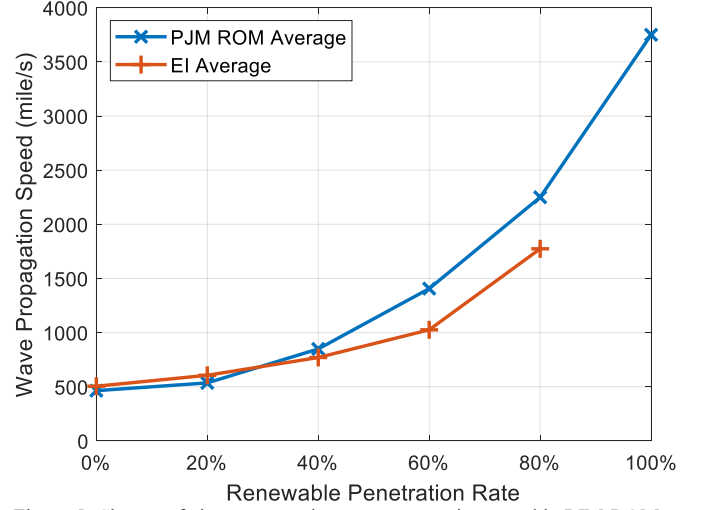
Figure 5. Change of electromagnetic wave propagation speed in PJM-ROM and the EI
