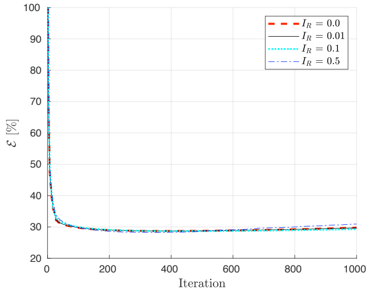
(b) Error, \mathcal{E} , versus iterations
