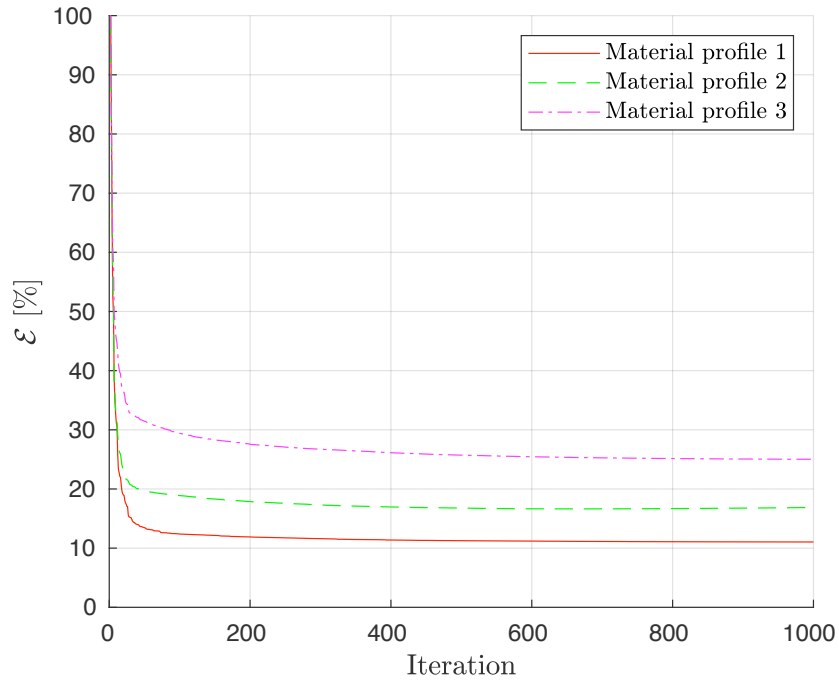
Figure 8: Example 1 - Error, \mathcal{E} , versus iterations with respect to the material profiles.
