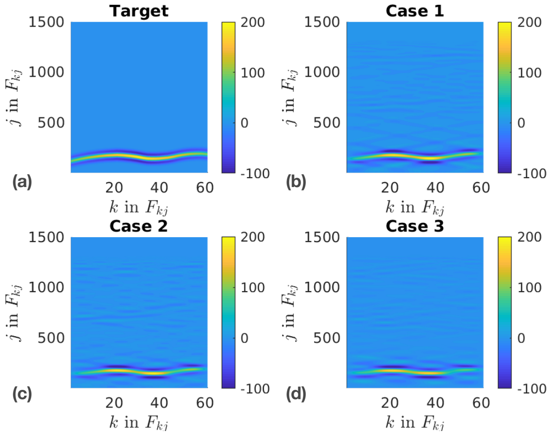
Figure 6: (a) Target and (b-d) Reconstructed F_1(x, t) for Cases 1-3 at the 1000th iteration. Horizontal and vertical axis in the contour plot represent, respectively, the numbering of the discretized points over space ( x ) and time ( t ) of the distribution of F_1(x, t) .
