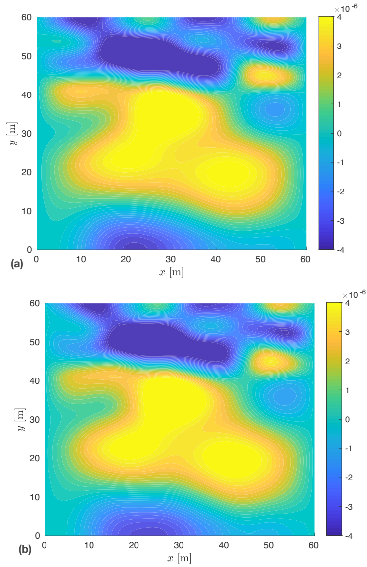
Figure 10: Wave responses, u(x, y, t) , at 1.5 seconds due to (a) target traction and (b) reconstructed traction in Case 3.
