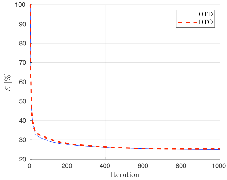
(b) Error, \mathcal{E} , versus iterations
