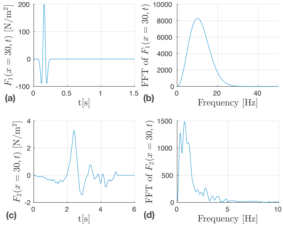
Figure 3: (a) The time signal of F_1(x = 30, t) ; (b) the amplitude of Fourier Transform of F_1(x = 30, t) ; (c) the time signal of F_2(x = 30, t) ; and (d) the FFT of F_2(x = 30, t) .
