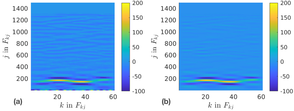
Figure 16: Example 4 - Estimated traction F_1(x, t) for (a) Case 8, where I_R = 1.0 , and (b) Case 11, where I_R = 0.0
