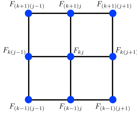
Figure 2: F_{kj} is surrounded by four elements in the space in terms of x and t : the horizontal and vertical axes represent, respectively, the x coordinate and time t .
