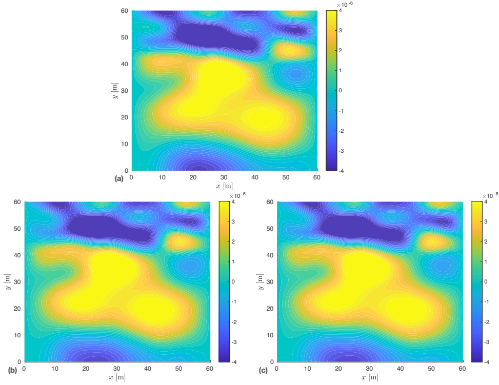
Figure 11: (a) Targeted F_1(x, t) and (b,c) Reconstructed F_1(x, t) for the OTD and DTO approaches, respectively, at the 1000th iteration.
