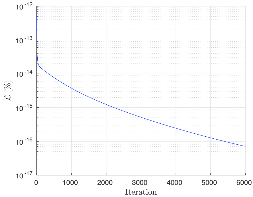
Figure 20: Example 6 - Objective function, \mathcal{L} , versus iterations.
