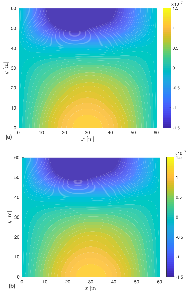
Figure 22: Wave responses, u(x, y, t) , at 6.0 seconds due to (a) target load and (b) reconstructed load in Case 18.
