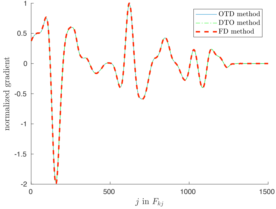
Figure 5: Comparison between the gradients generated by the OTD approach, DTO approach and the FD approximation.
