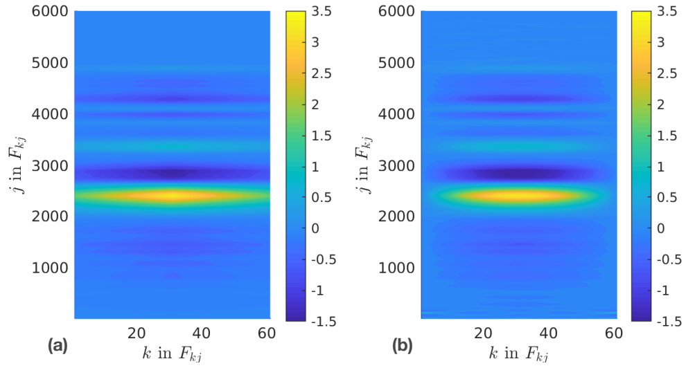
Figure 19: Example 6 - (a) Target and (b) Reconstructed F_2(x, t) for Case 18 at the 6000-th iteration.
