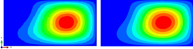
Figure 26: Discrete (left) and smeared (right) thickness, 1st eigenmode of case 3.
