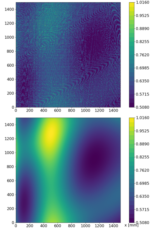
Figure 18: Discrete (top) and smeared (bottom) thickness profile of case 1.
