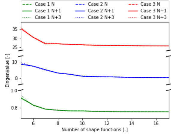
Figure 21: Semi-analytical model convergence of the smeared thickness approach for N , N+1 and N+3 integration points.
