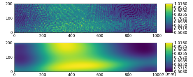
Figure 19: Discrete (top) and smeared (bottom) thickness profile of case 2.
