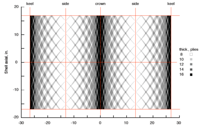
Figure 3: Discretised laminate thickness [39].
