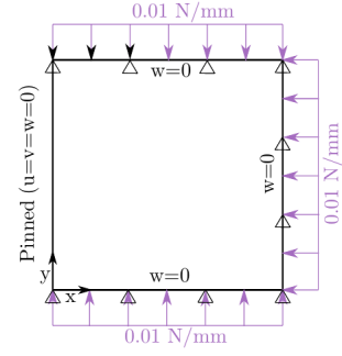
Figure 14: Definition of test case 1.
