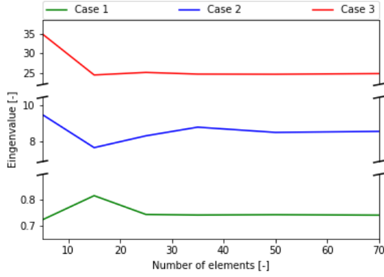
Figure 23: FE convergence using the discrete thickness approach.
