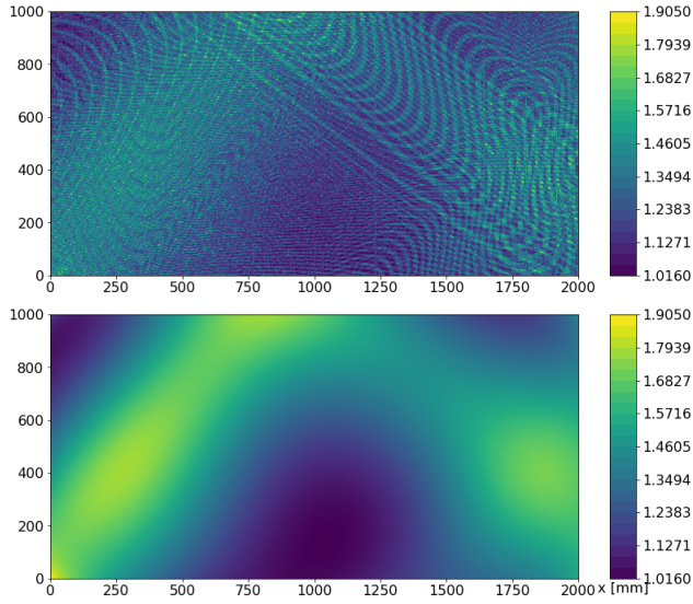
Figure 20: Discrete (top) and smeared (bottom) thickness profile of case 3.
