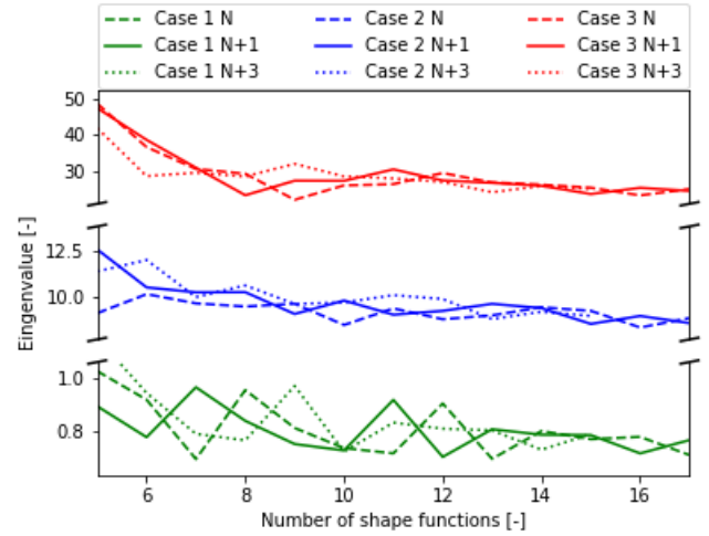
Figure 22: Semi-analytical model convergence of the discrete thickness approach for N , N+1 and N+3 integration points; where N is the order of the Legendre polynomials used as shape functions.
