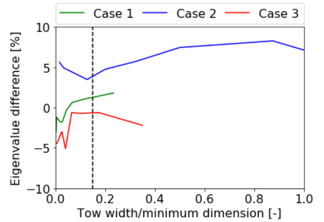
Figure 27: First linear buckling eigenvalue error, of the smeared relative to the discrete thickness approach, for different tow widths per minimum dimension ratios.
