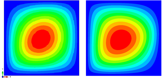
Figure 24: Discrete (left) and smeared (right) thickness, 1st eigenmode of case 1.
