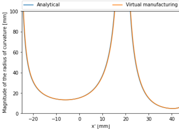
Figure 17: Tow path radius comparison between the virtual manufacturing and the analytical expression of Equation 19.
