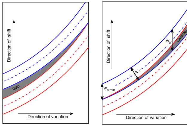
(a) Gap between two courses (b) Overlapping courses
