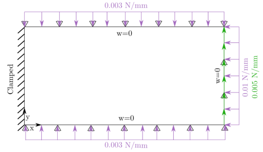
Figure 16: Definition of test case 3.
