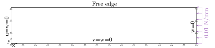
Figure 15: Definition of test case 2.
