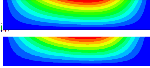
Figure 25: Discrete (top) and smeared (bottom) thickness, 1st eigenmode of case 2.
