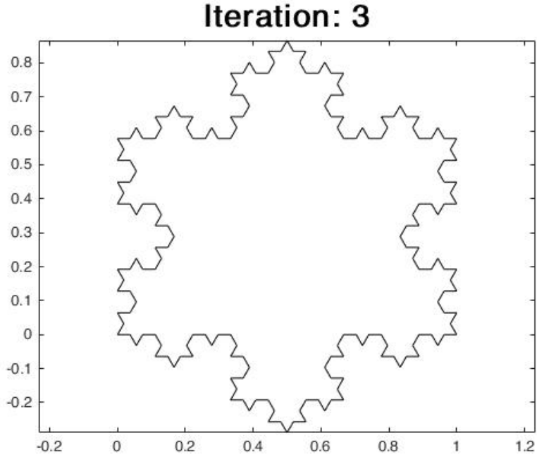
Figure 1: Koch Snowflake Curve (for n=3 )
