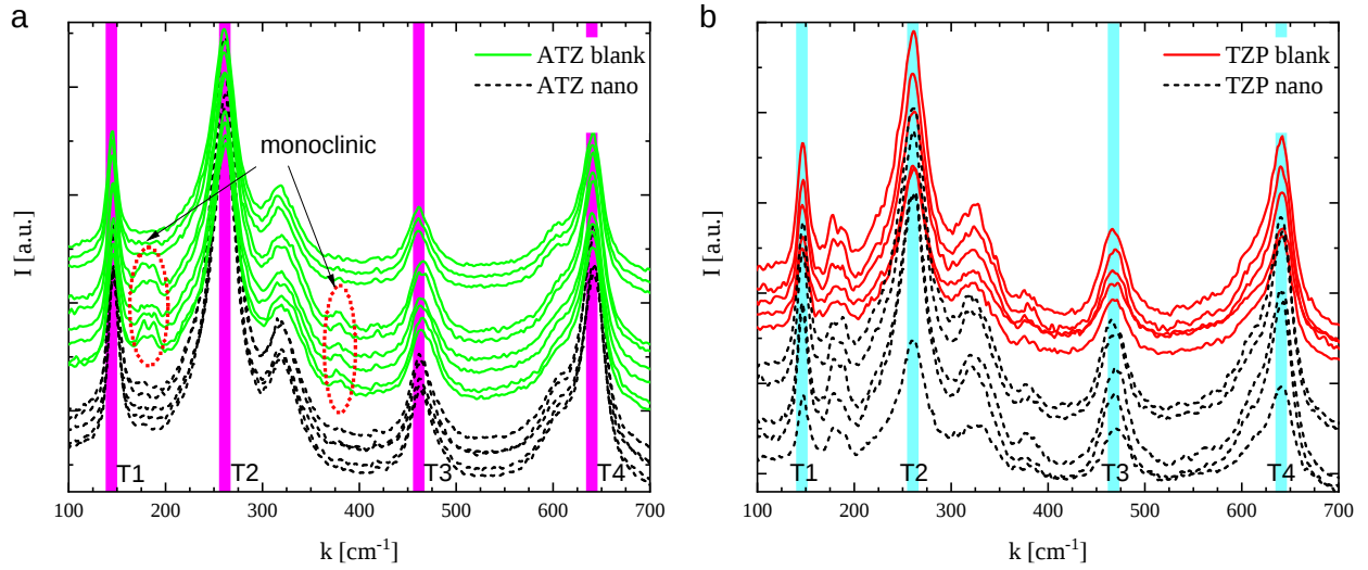
Figure 7: Raman measurements of the blank, nano ATZ (a) and TZP (b) composite revealing the persistence of the tetragonal phase with an offset for clarity. The spectra for the blank (solid) and nano (dashed) point to a negligible impact of USP ablation reducing the monoclinic phase for ATZ.
