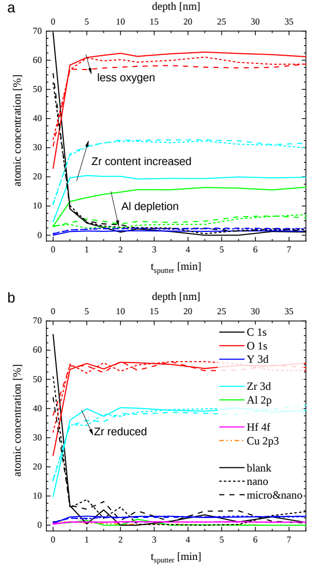
Figure 10: XPS depth profiles following the main constituents of the ATZ (a) and TZP (b) specimen revealing a clear change in chemistry for ATZ correlated with the laser machining for the nano surface structures. For TZP Zr is reduced in the first 10 nm.
