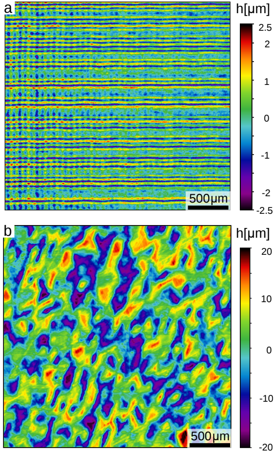
Figure 5: Surface design and confocal measurement of the ATZ ceramic. (a) The rough surfaces is laser-structured by cross-hatching and (b) the superposition with microstructures and random height with spacing of 50\text{ }\mu\text{m} and peak to valley height of 40\text{ }\mu\text{m} .
