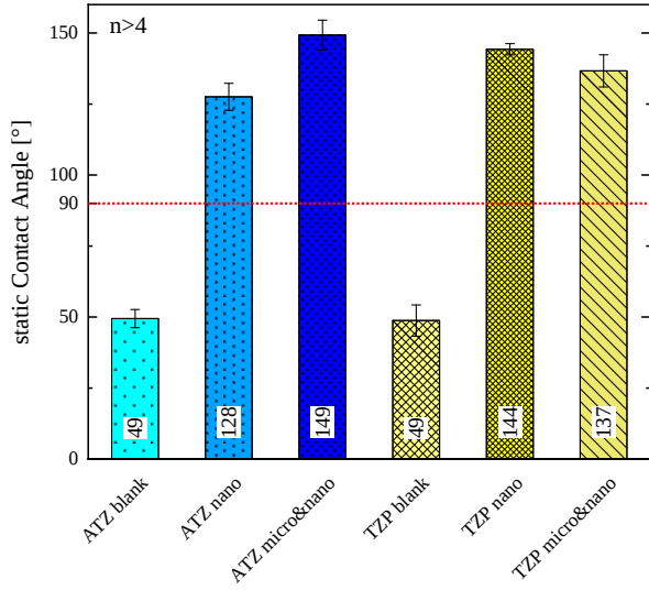
Figure 9: Static contact angle of two samples per surface at more than two locations. For both ceramics laser machining induces a transition from hydrophilic to -phobic wettability.
