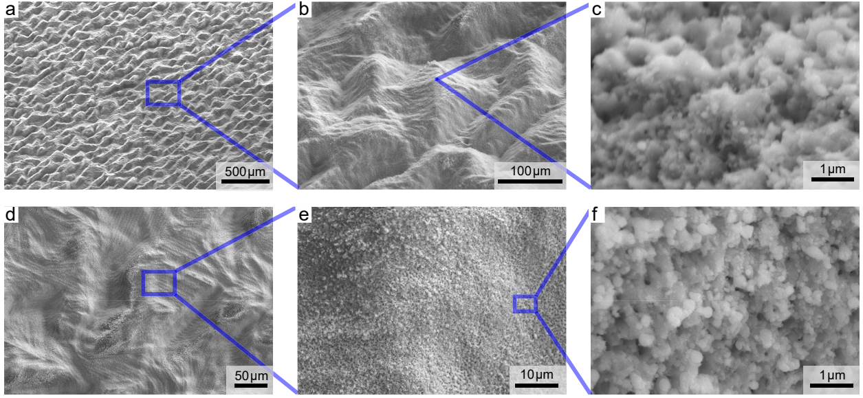
Figure 6: SEM graphs of the micro&nano hierarchical structures on ATZ (a-c) in the upper row tilted by 40 deg and TZP (d-f) at the bottom. The rational designed micro features (a,b,d,e) are superimposed by the designed nano-roughness (c,f). The quality of the structures on both materials is comparable shown with higher magnification in (c) and (f).
