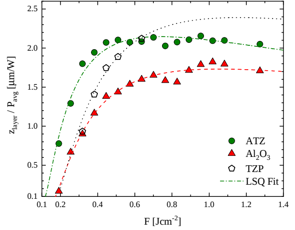
Figure 3: Specific material removal rate given by the ablation layer depth z_{\text{layer}} scaled by the average power P_{\text{avg}} . To determine the multi-pulse threshold and optimal efficient fluence a least square curve fitting following (1) and (2) is applied.
