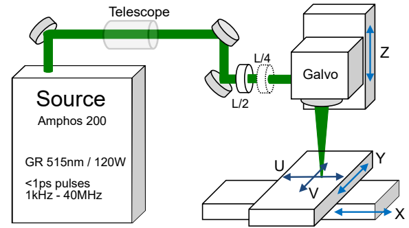
Figure 2: Experimental laser test bed constituted by a source, beam guidance, optical (U, V), and mechanical (X, Y, Z) axes for fast beam steering plus positioning.
