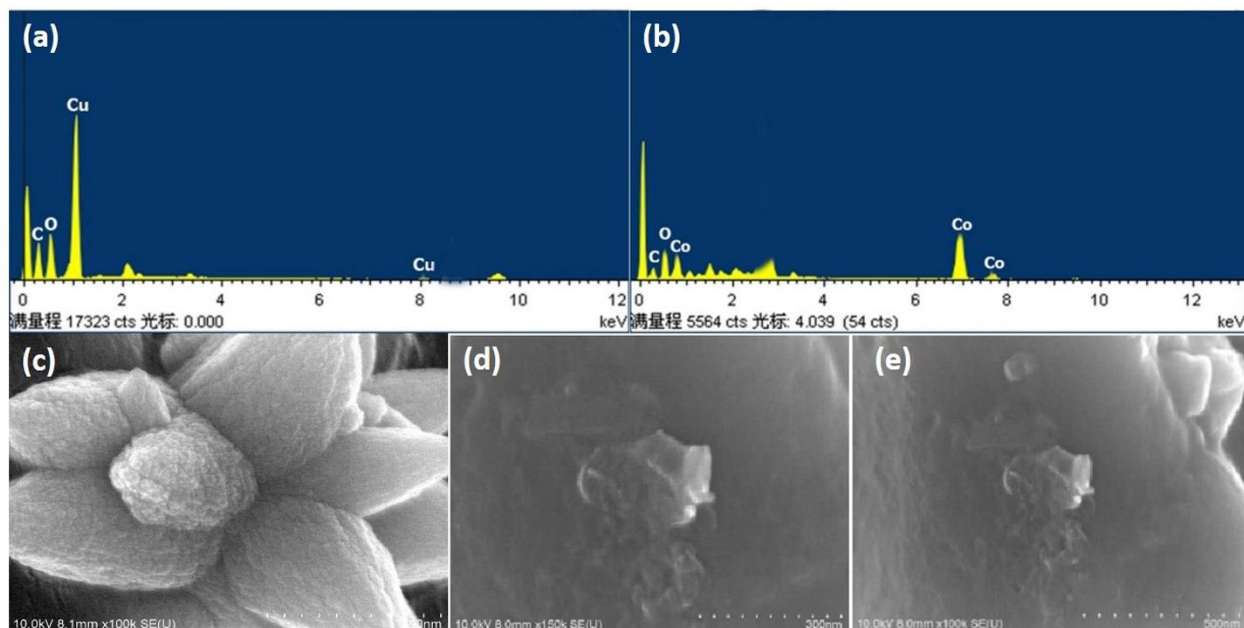
Figure 5 (a, b) EDX images of copper oxide nanoparticles and cobalt oxide nanoparticles. (c, d, e) SEM images of copper oxide nanoparticles and cobalt oxide nanoparticles
