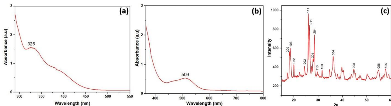
Figure 4 (a, b) UV-Vis spectroscopy of copper oxide nanoparticles and cobalt oxide nanoparticles, (c) XRD graph of copper oxide nanoparticles
