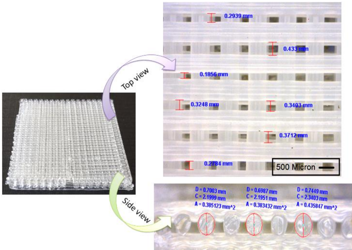
Figure 6. The microscopic view of the fabricated scaffold
