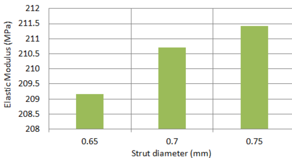
Figure 11. Investigation of the effect of struts' diameter on the elastic modulus of bone scaffold
