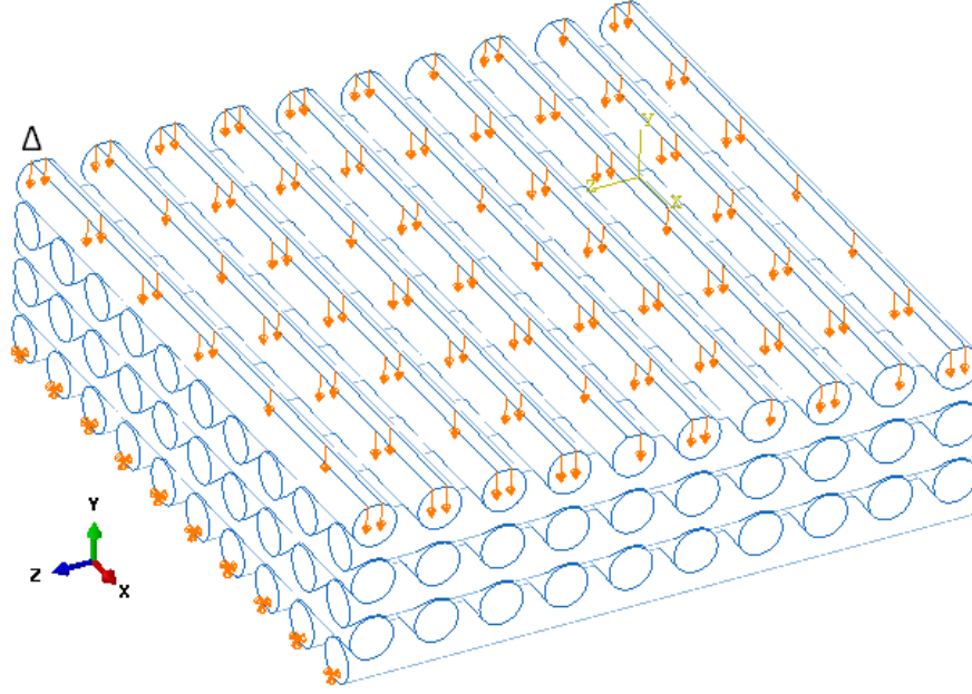
Figure 5. Schematic of the applied boundary conditions to the bone scaffold
