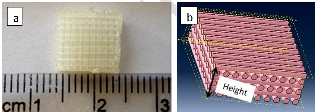
Figure 2. a) Front view of the fabricated bone scaffold via FDM technique, b) three dimensional view of the designed scaffold
