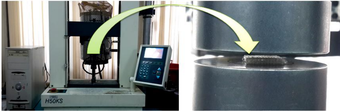
Figure 3. View of the performed compression tests setup
