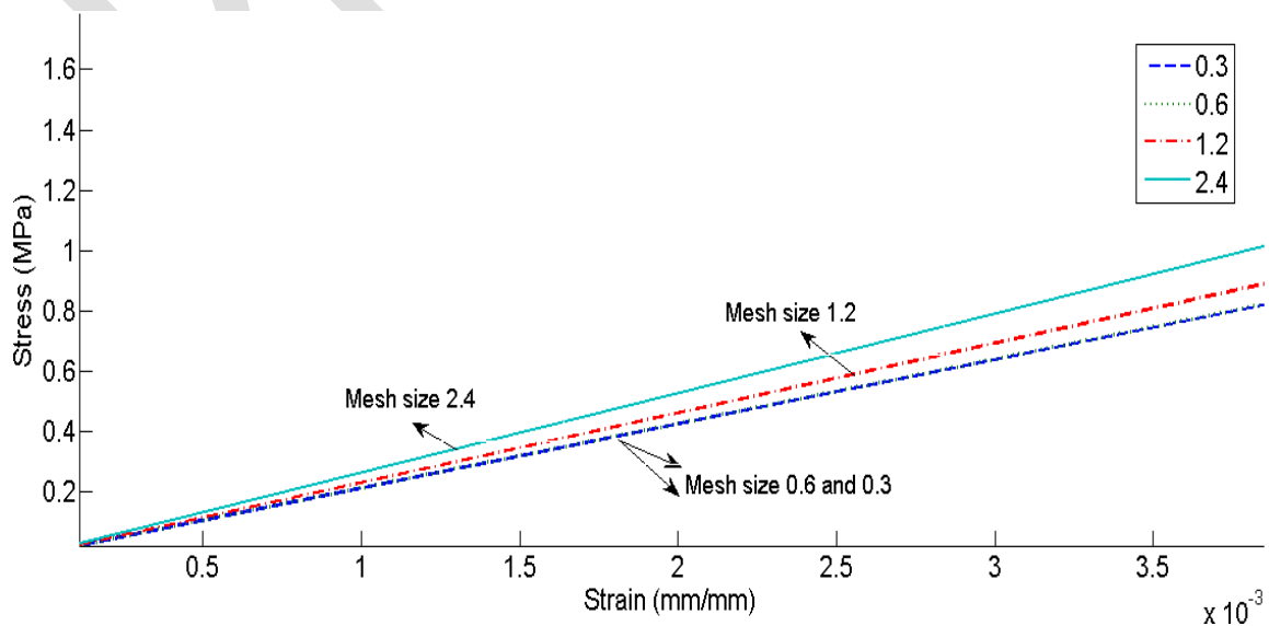
Figure 10. The results of mesh sensitivity analysis
