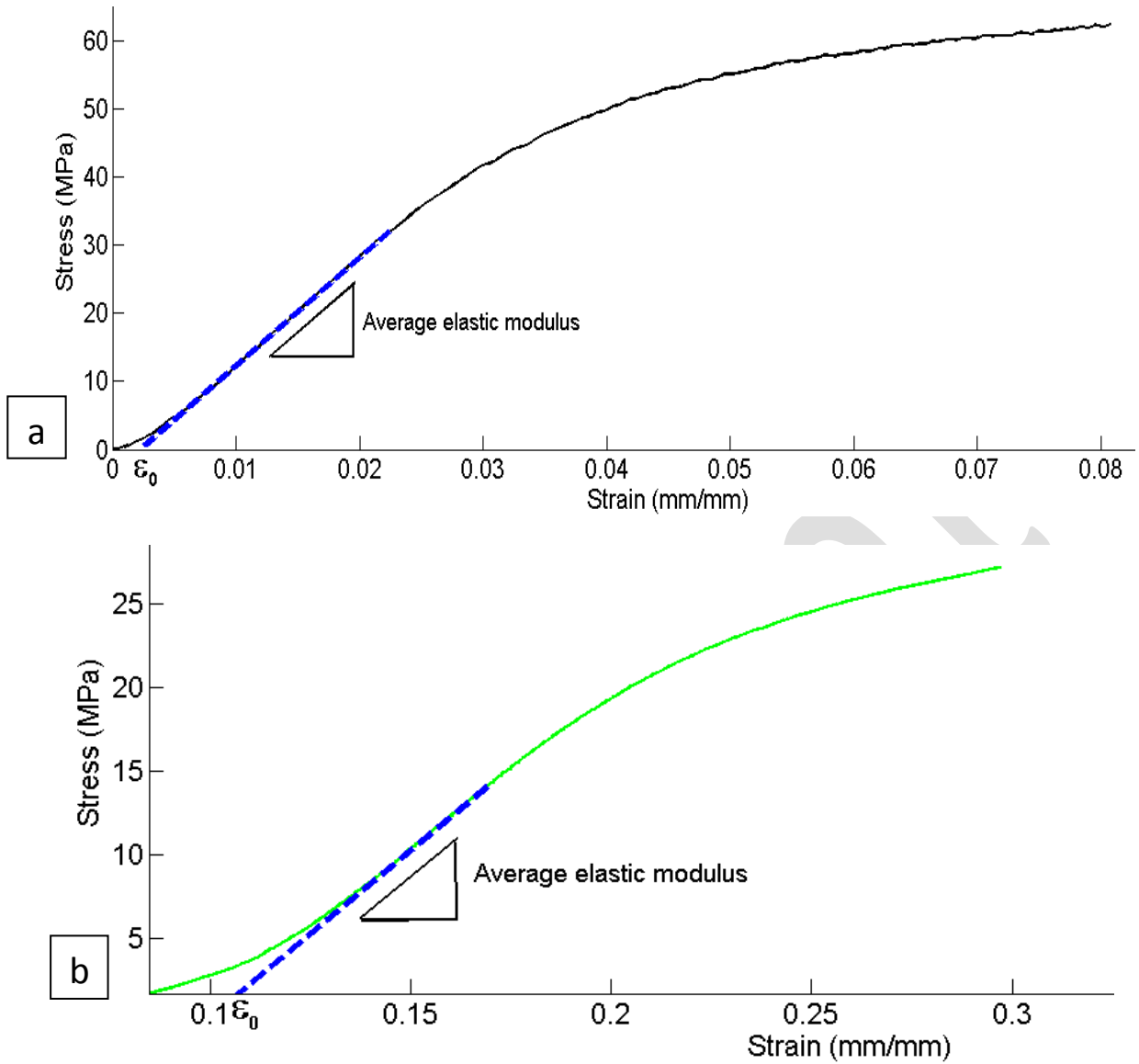
Figure 8. Experimental and corrected stress–strain curve of a) the bulk material and b) the bone scaffold specimen
