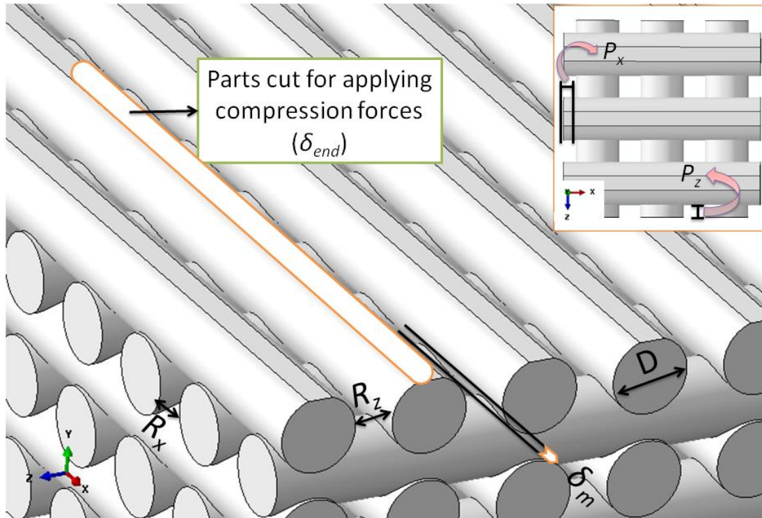
Figure 4. Schematic of the internal structure and parameters of the designed scaffold in finite element model
