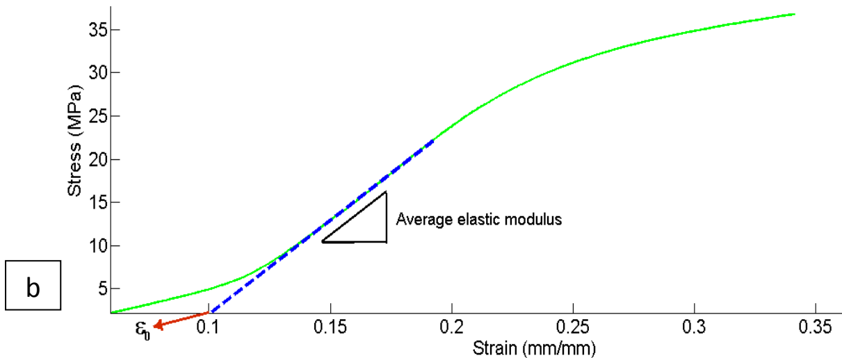
Figure 14. Experimental and corrected stress–strain curve of a) the bulk post-heated and b) post-heated bone scaffold specimen
