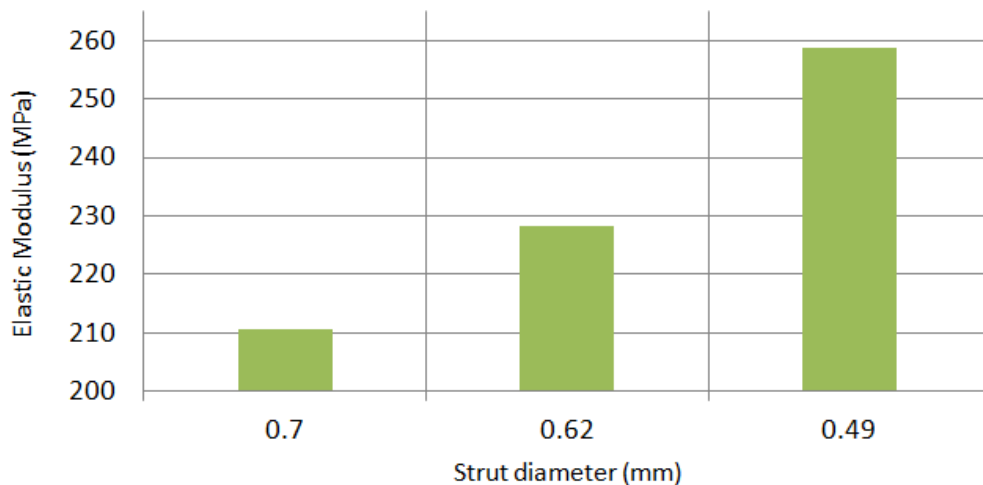
Figure 12. Investigation of the effect of struts' diameter on mechanical properties in fix porosity
