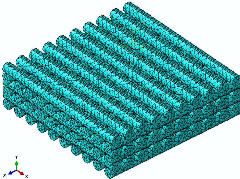
Figure 9. A schematic of the meshed bone scaffold
