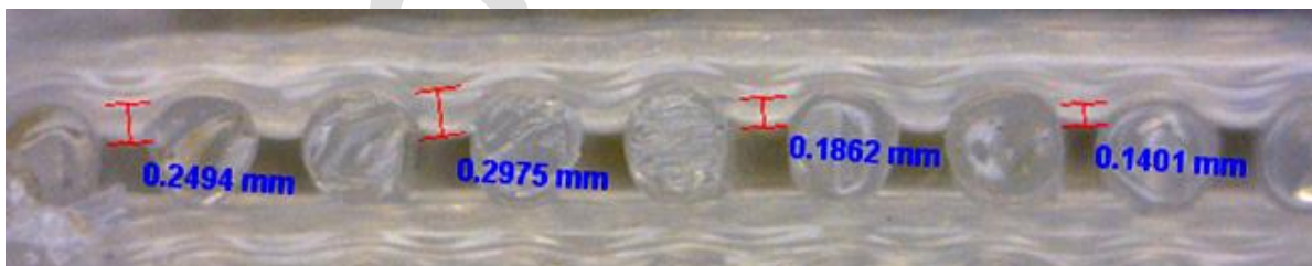
Figure 7. The amount of layer adhesion between additive manufactured bone scaffold layers
