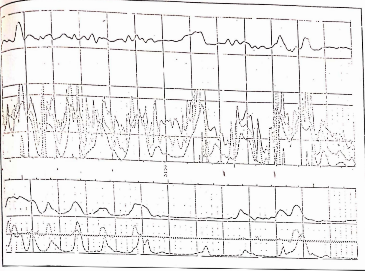
Fig. (B-6) MSFL/SFL/ILD/DT/SP/RWA for Well No. (EB-79)
