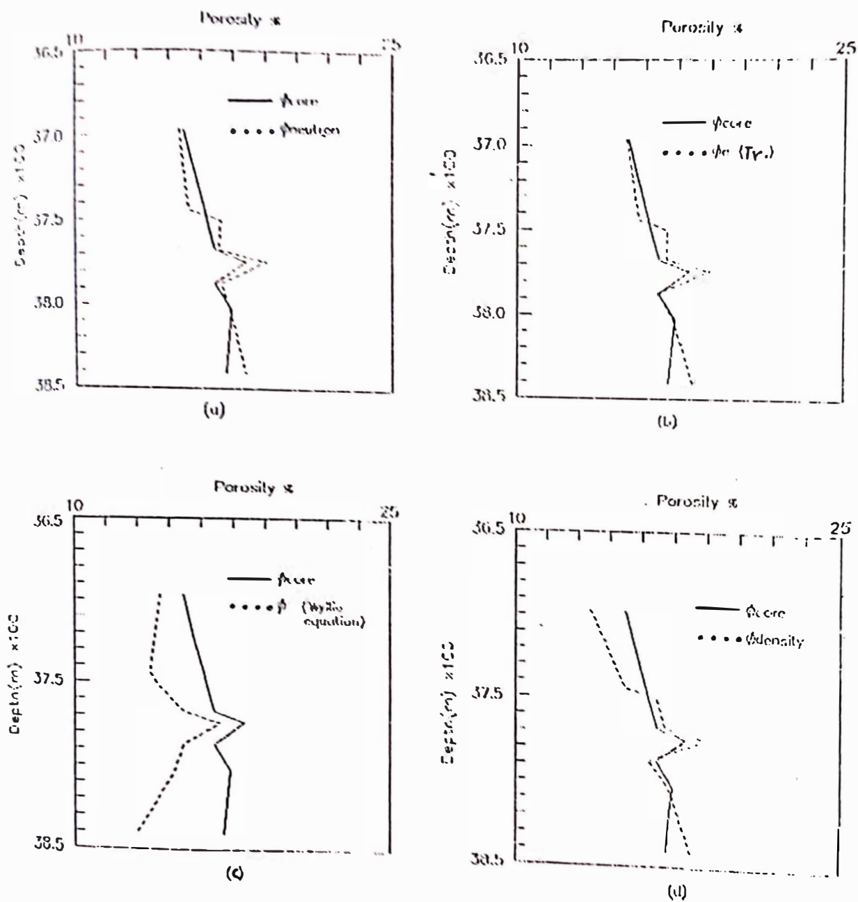
Fig.(4-24) \phi_{core} - \phi_{log} comparisons for Well No.(EB-18).
