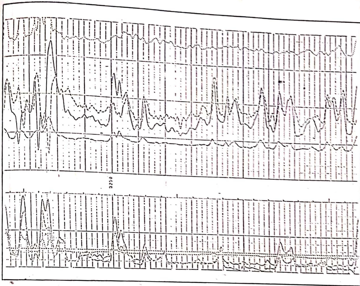
Fig.(B-1) FDC/CNL/CAL/GR Logs for Well No.(EB-55)
