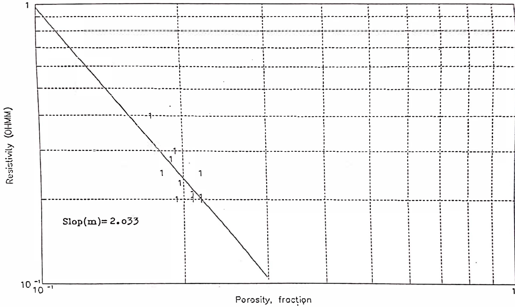
Fig.( 5 - 4 ) Resistivity - Porosity cross plot for Well No.(EB-79) .
