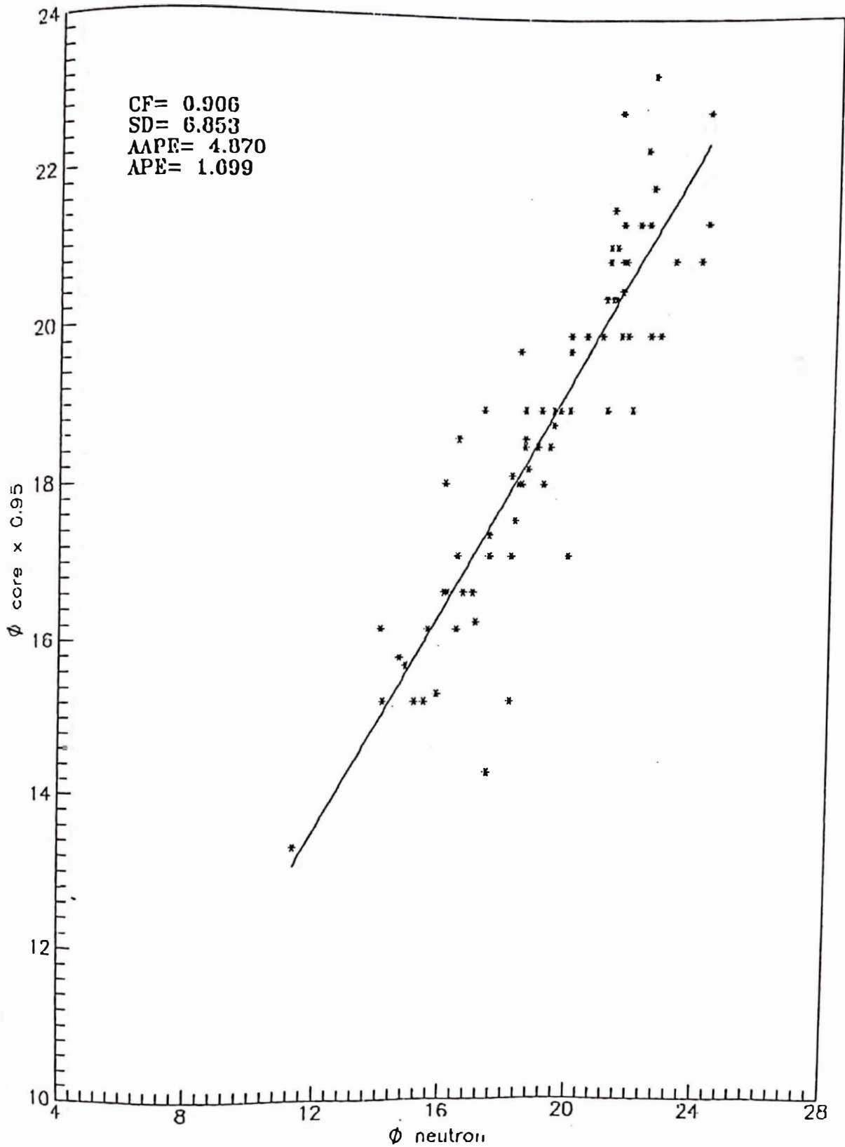
Fig.(4-16) Plot of \phi core vs. \phi neutron for the Wells of Zubair formation-East Baghdad field.
