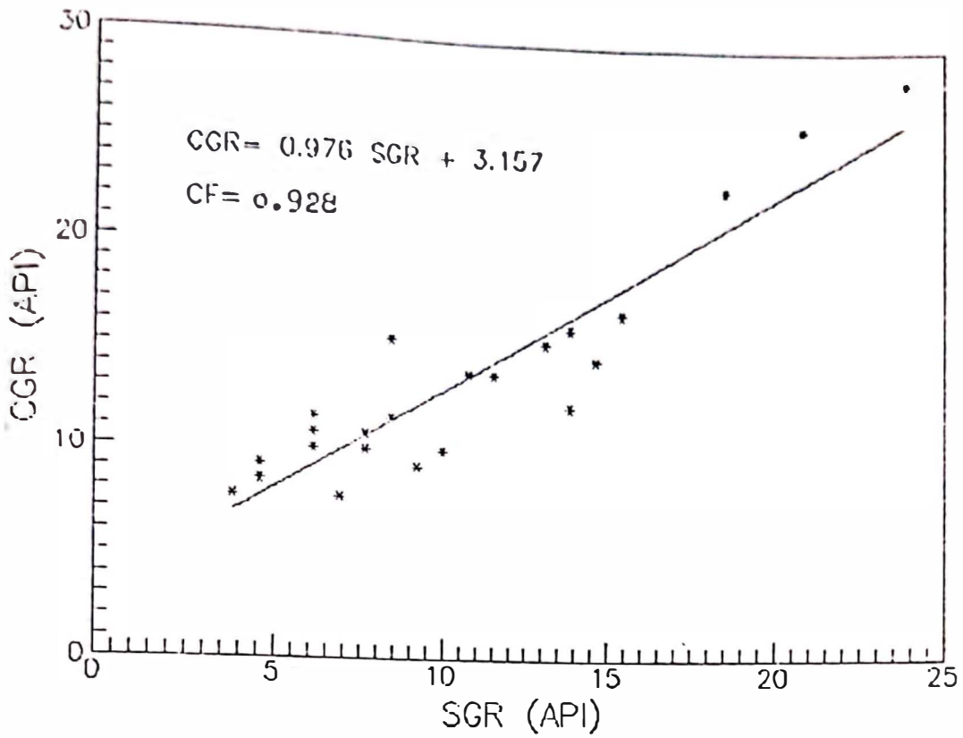
Fig.(4 - 5 ) Corrected gamma ray-Standard gamma ray relationship for sand body No. 5 .
