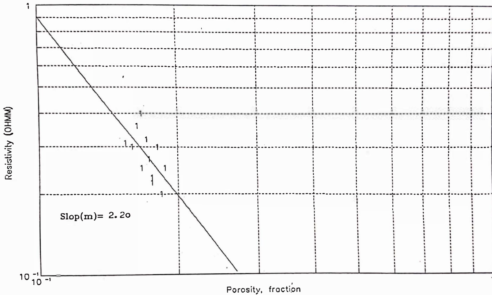
Fig.( 5 - 6 ) Resistivity - Porosity cross plot for Well No.(EB-15) .
