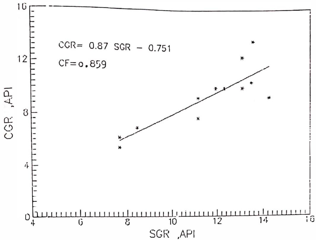
Fig.(4 - 1 ) Corrected gamma ray-Standard gamma ray relationship for sand body No. 1 .
