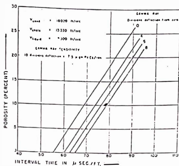
Fig.( 2-1) Theoretical plot of porosity vs transit time with increasing shale as indicated by Gamma Ray deflection
