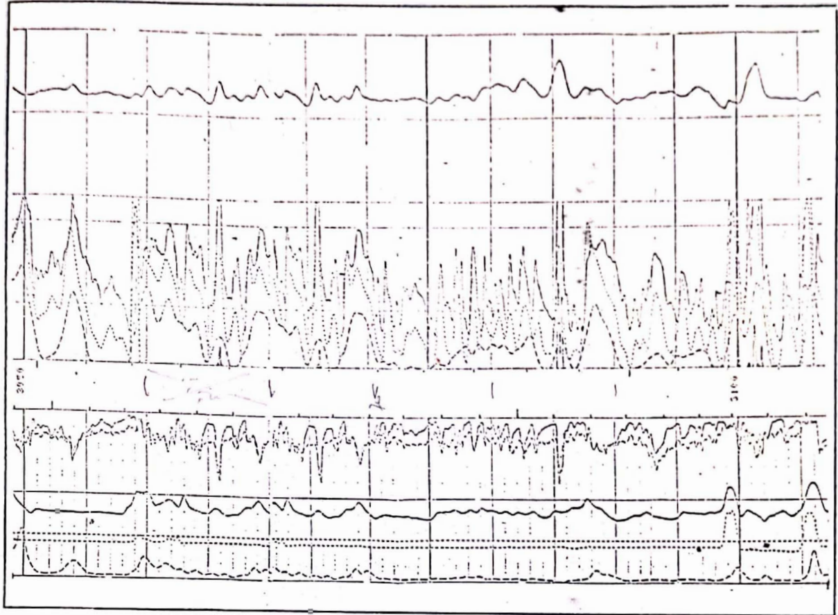
FIG. (B-8) MSFL/SFL/ILD/DT/SP/Rwa for Well No. (EB-77)
