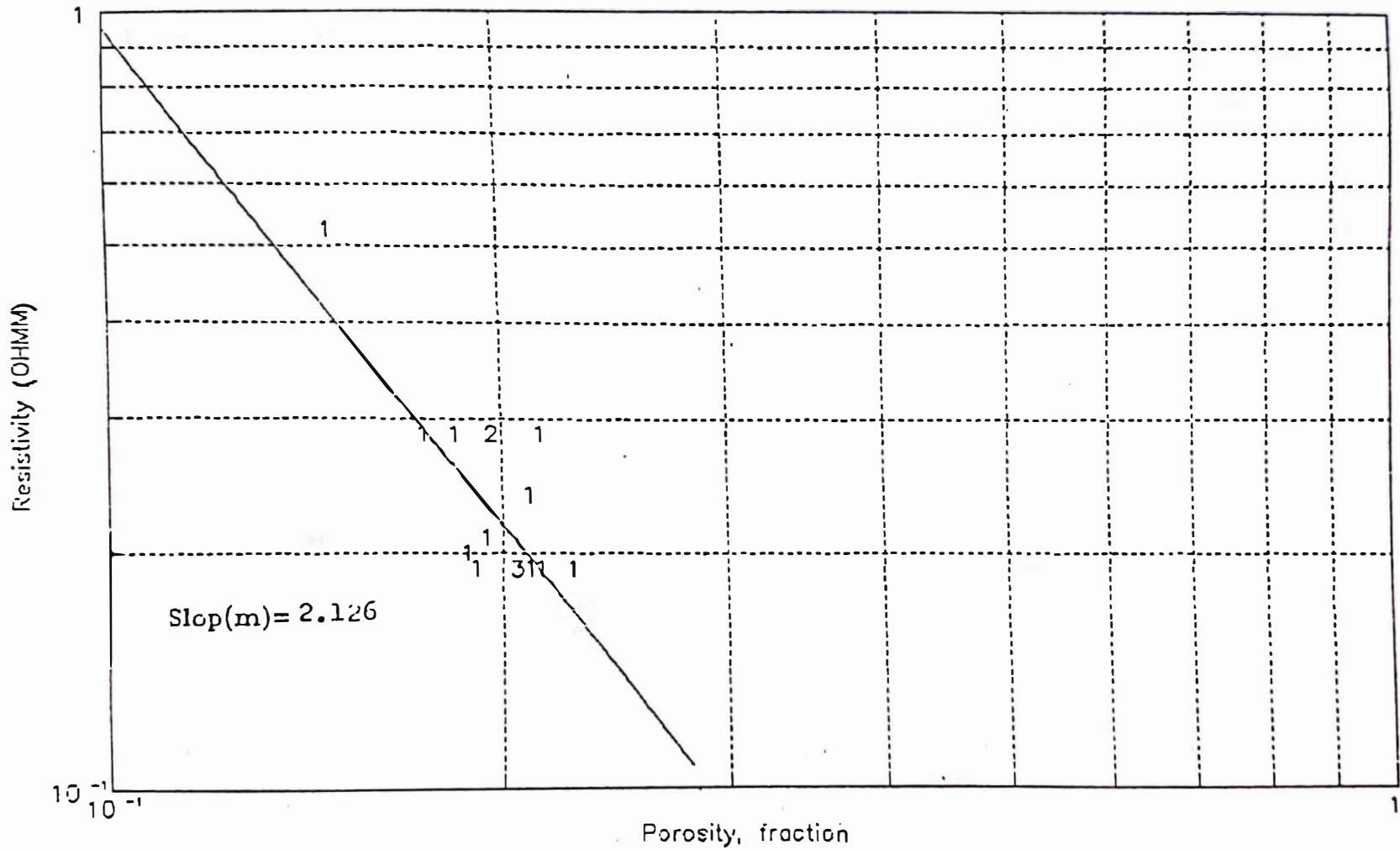
Fig.( 5 - 2 ) Resistivity - Porosity cross plot for Well No.(EB-55) .
