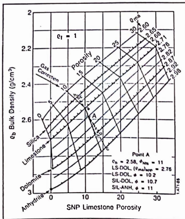
Fig. 2. 4 —Neutron-density crossplot scaled with interpolated c_{ma} lines.
