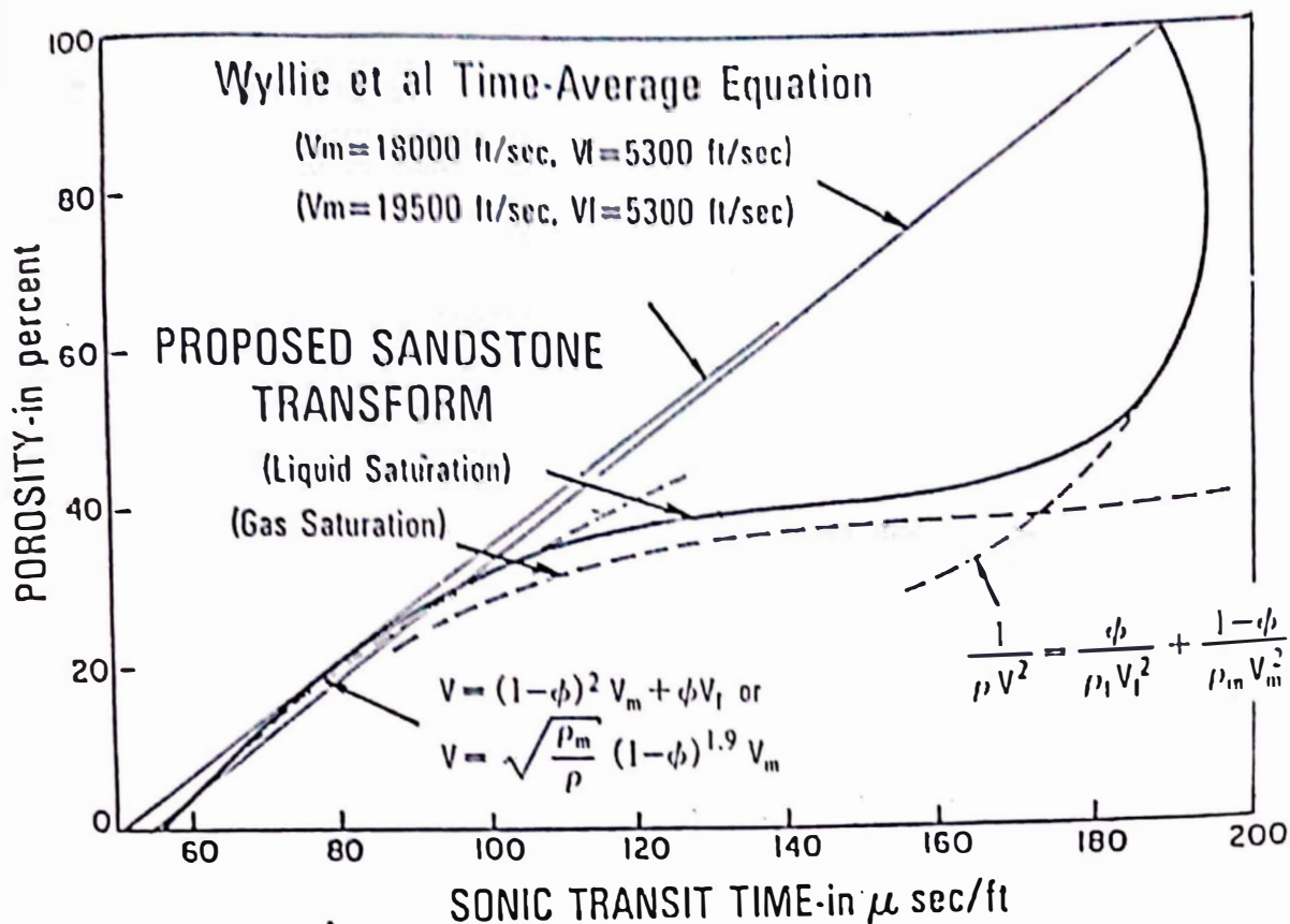
Fig.(2-3) The proposed sonic transit time-to porosity transform, showing comparison to Wyllie time-average equation (1956) and to suggested algorithms by Raymer et al. (1980).
