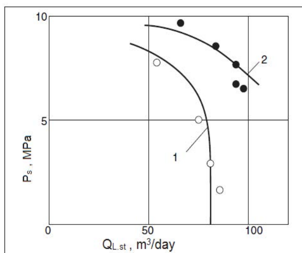
Figure 2: Comparison of the calculated and actual characteristics of the ESP5-130-1200 : 1 - the calculated P_s - Q_{L.st} curve for a pump without a gas separator at P_{in} = 5.18 MPa, d_c = 35 mm, water cut 0.051 and \beta_{in} = 0.38 ; \circ - actual operating modes of the pump without a gas separator at P_{in} = 5.12-5.22 MPa, water cut 0.017–0.100, \beta_{in} = 0.37 - 40 ; 2 - calculated curve P_s - Q_{L.st} for a pump with a gas separator at P_{in} = 3.1 MPa, d_c = 35 mm, zero water cut, \beta_{in} = 0.61 and Sc = 0.85 ; \bullet - actual operating modes of the pump with a gas separator at P_{in} = 2.9-3.45 MPa, zero water cut, \beta_{in} = 0.57-0.63 and Sc = 0.75-1.0 .
