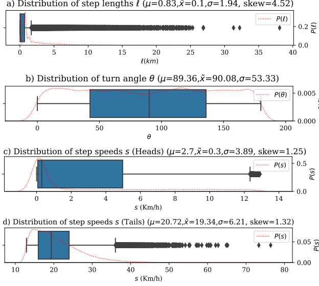
Figure 3: Summary distributions for all minibus taxis' step lengths, turning angles and steps speeds (speeds were calculated for distances where heads \leq 0.676 km, tails > 0.676 km).
