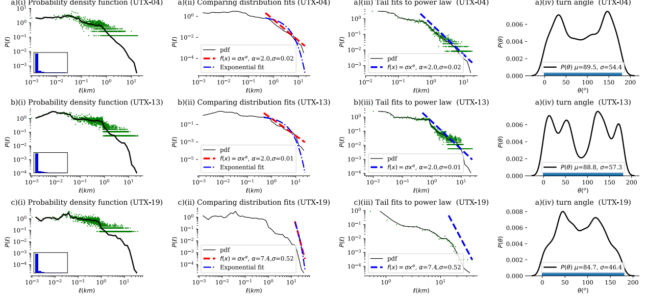
Figure 5: Power-law analysis of Lévy walk steps.
