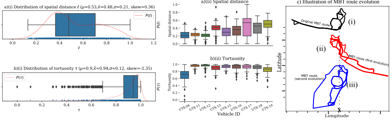
Figure 4: (a) distribution of normalized spatial distance (b) distribution of normalized tortuosity, (c) illustration of minibus taxi route evolution over time.
