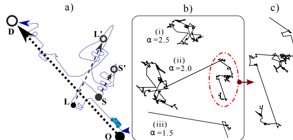
Figure 1: The concepts of Lévy walk (LW), and minibus taxi movement behavior: a) minibus taxi passenger search behavior from origin (O) to destination (D); b) Lévy walks with different values of Lévy exponent \alpha ; c) scale-invariant and fractal properties of a Lévy walk.
