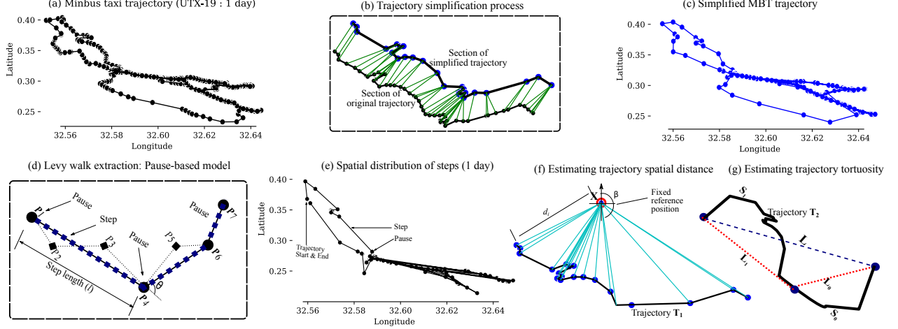
Figure 2: a) Minibus taxi (MBT) trajectory sample for one day; b) trajectory simplification process; c) simplified trajectory, d) pause-based model to extract steps from a section of the minibus taxi trajectory in a, (e) spatial distribution steps and pauses extracted from the simplified trajectory in (c); f) trajectory spatial distance estimation; and g) trajectory tortuosity estimation.
