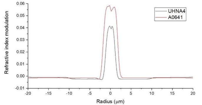
Figure 1: Refractive index profiles of two high germanium content optical fibers under test.
