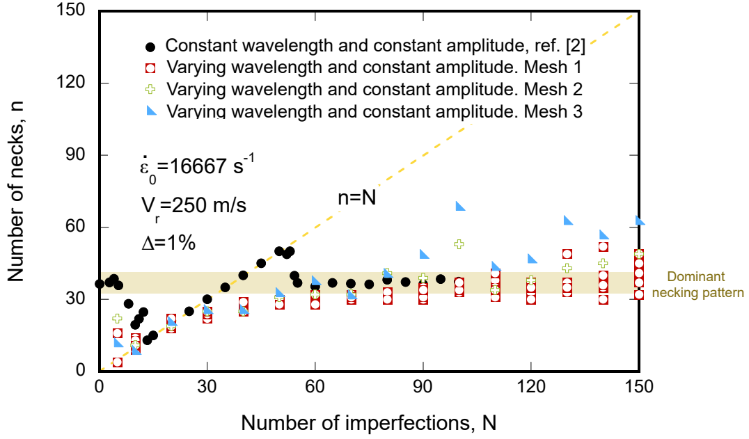
Figure A.16: Number of necks n as a function of the number of imperfections N for an imposed initial strain rate of \dot{\epsilon}_0 = 16667 \text{ s}^{-1} (which corresponds to V_r = 250 \text{ m/s} ). The results are obtained for three different meshes: Mesh 1 with \approx 100000 elements, Mesh 2 with \approx 150000 elements and Mesh 3 with \approx 200000 elements. The results for Mesh 1 are obtained for five random distributions of imperfection wavelengths (RDIW _i with i = 1, \dots, 5 ), and the results for Mesh 2 and Mesh 3 are obtained with an additional random distribution of imperfection wavelengths RDIW _6 . A comparison is performed with the finite element calculations performed by Rodríguez-Martínez et al. [33] for rings with constant wavelength imperfections. The amplitude of the imperfections is \Delta = 1\% .
