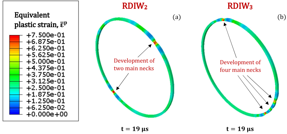
Figure 7: Contours of equivalent plastic strain \bar{\epsilon}^P . Imposed initial strain rate of \dot{\epsilon}_0 = 16667 \text{ s}^{-1} (which corresponds to V_r = 250 \text{ m/s} ). Number of imperfections N = 10 . The amplitude of the imperfections is \Delta = 1\% . Loading time t = 19 \mu\text{s} (a) Random distribution of imperfection wavelengths \text{RDIW}_2 . (b) Random distribution of imperfection wavelengths \text{RDIW}_3 .
