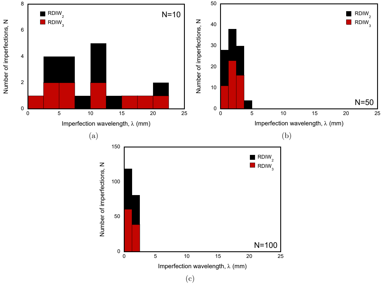
Figure 2: Histograms showing the number of imperfections N as a function of the imperfection wavelength \lambda . Results are presented for two different random distributions of imperfection wavelengths: RDIW_2 (black blocks) and RDIW_3 (red blocks). The height of a colored block within a bar of the histogram marks the number of imperfections within a fixed \lambda interval for a given distribution of imperfection wavelengths. Results are shown for different number of imperfections: (a) N = 10 , (b) N = 50 and (c) N = 100 . For interpretation of the references to color in the text, the reader is referred to the web version of this article.
