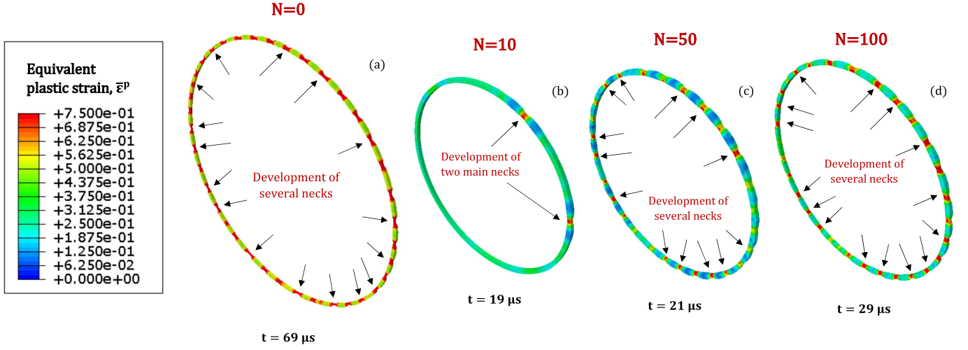
Figure 4: Contours of equivalent plastic strain \bar{\epsilon}^p . Imposed initial strain rate of \dot{\epsilon}_0 = 16667 \text{ s}^{-1} (which corresponds to V_r = 250 \text{ m/s} ). (a) Number of imperfections N = 0 . Loading time t = 69 \mu\text{s} . (b) Number of imperfections N = 10 . Loading time t = 19 \mu\text{s} . (c) Number of imperfections N = 50 . Loading time t = 21 \mu\text{s} . (d) Number of imperfections N = 100 . Loading time t = 29 \mu\text{s} . For N = 10, 50 and 100 the amplitude of the imperfections is \Delta = 1\% and the random distribution of imperfection wavelengths is \text{RDIW}_1 . All the isocontours have the same colour coding such that equivalent plastic strains ranging from 0 to 0.75 correlate with a colour scale that goes from blue to red. If the value of the equivalent plastic strain is above 0.75, it remains red.
