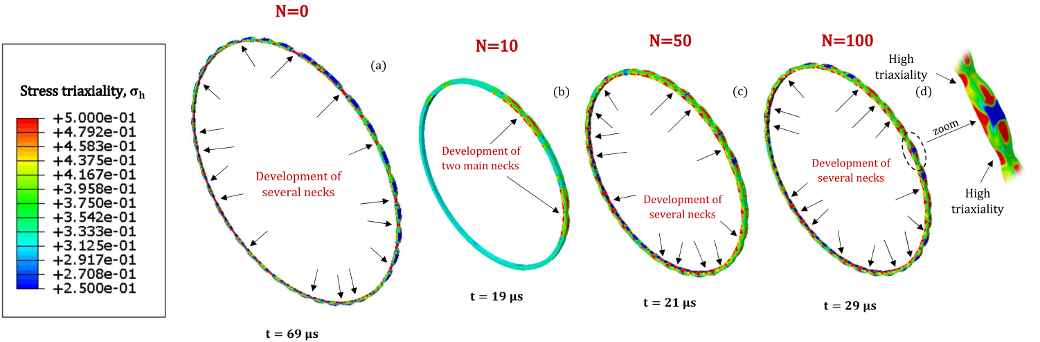
Figure 5: Contours of stress triaxiality \sigma_h . Imposed initial strain rate of \dot{\epsilon}_0 = 16667 \text{ s}^{-1} (which corresponds to V_r = 250 \text{ m/s} ). (a) Number of imperfections N = 0 . Loading time t = 69 \mu\text{s} . (b) Number of imperfections N = 10 . Loading time t = 19 \mu\text{s} . (c) Number of imperfections N = 50 . Loading time t = 21 \mu\text{s} . (d) Number of imperfections N = 100 . Loading time t = 29 \mu\text{s} . For N = 10, 50 and 100 the amplitude of the imperfections is \Delta = 1\% and the random distribution of imperfection wavelengths is \text{RDIW}_1 . All the isocontours have the same colour coding such that stress triaxialities ranging from 0.25 to 0.5 correlate with a colour scale that goes from blue to red. If the value of stress triaxiality is below 0.25, it remains blue, and if it is above 0.75, it remains red.
