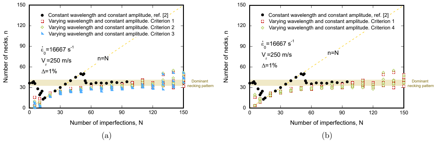
Figure B.17: Number of necks n as a function of the number of imperfections N for an imposed initial strain rate of \dot{\epsilon}_0 = 16667 \text{ s}^{-1} (which corresponds to V_r = 250 \text{ m/s} ). The results obtained for five random distributions of imperfection wavelengths (RDIW _i with i = 1, \dots, 5 ) are compared with the finite element calculations performed by Rodríguez-Martínez et al. [33] for rings with constant wavelength imperfections. The amplitude of the imperfections is \Delta = 1\% . The results corresponding to the random distributions of imperfection wavelengths are obtained using: (a) criteria 1, 2 and 3, (b) criteria 1 and 4. For interpretation of the references to color in this figure, the reader is referred to the web version of this article.
