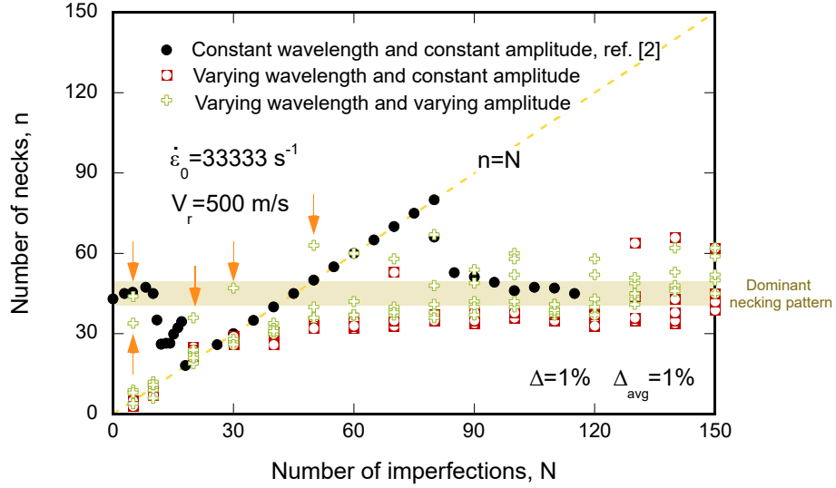
Figure 13: Number of necks n as a function of the number of imperfections N for an imposed initial strain rate of \dot{\epsilon}_0 = 33333 \text{ s}^{-1} (which corresponds to V_r = 500 \text{ m/s} ). The results obtained for five random distributions of wavelengths (RDIW _i with i = 1, \dots, 5 ) with imperfections of constant and varying amplitude are compared with the finite element calculations performed by Rodríguez-Martínez et al. [33] for rings with imperfections of constant wavelength and amplitude (i.e. the black and red markers correspond to results already shown in Fig. 9(a)). For the constant amplitude imperfections \Delta = 1\% . For the varying amplitude imperfections, the random distribution of imperfection amplitudes is bounded between 0.5% and 1.5%, with the mean of the distribution being \Delta_{\text{avg}} = 1\% . For interpretation of the references to color in this figure, the reader is referred to the web version of this article.
