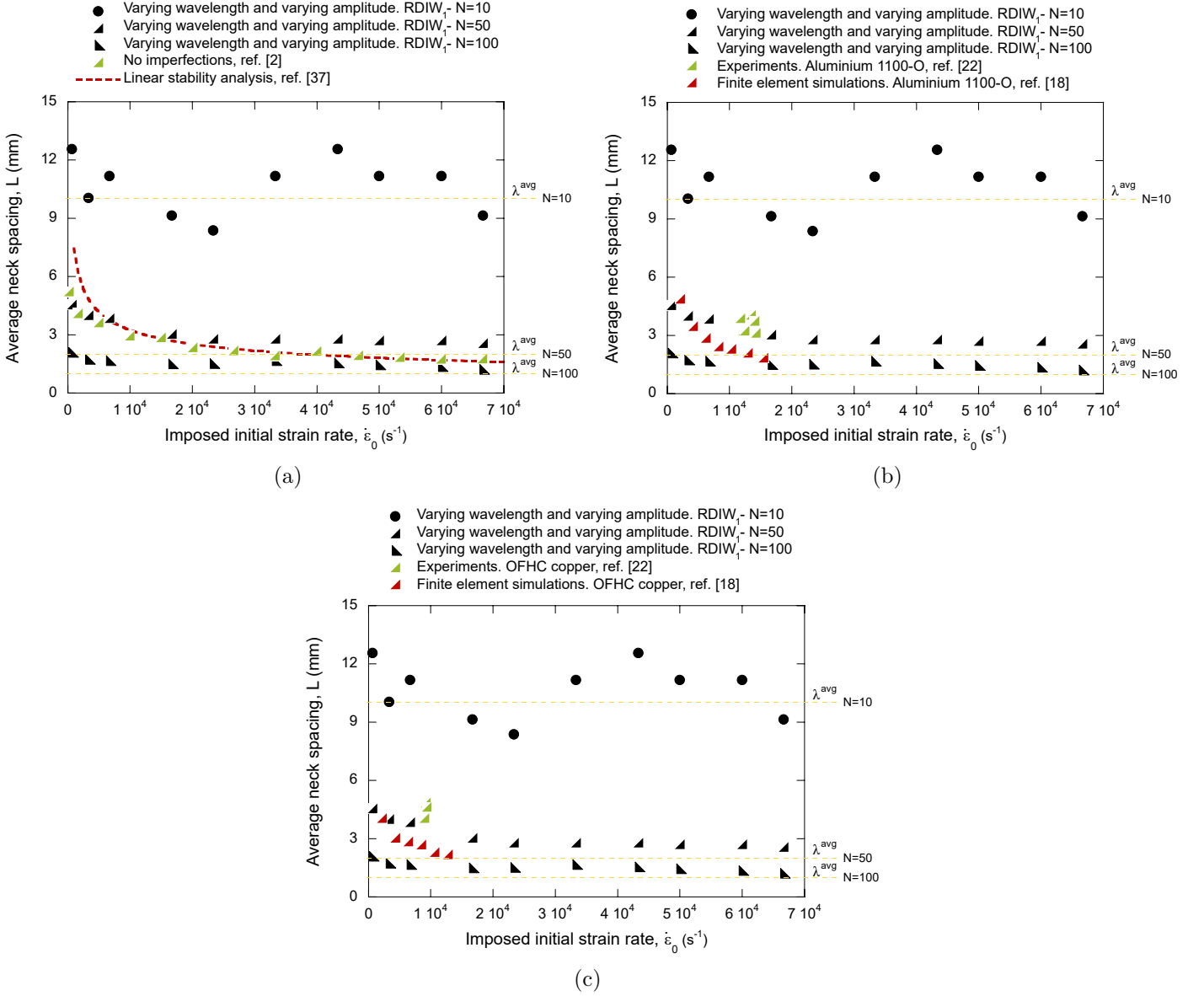
Figure 15: Average neck spacing L versus imposed initial strain rate \dot{\epsilon}_0 . Finite element results corresponding to imperfections of varying wavelength and amplitude for N = 10, 50 and 100 . The random distribution of imperfection wavelengths is \text{RDIW}_1 . The random distribution of imperfection amplitudes is bounded between 0.5\% and 1.5\% , with the mean of the distribution being \Delta_{\text{avg}} = 1\% . (a) Comparison with the finite element results for N = 0 reported by Rodríguez-Martínez et al. [33] and the linear stability analysis predictions reported by N'souglo et al. [30]. (b) Comparison with the experiments performed by Grady and Benson [9] and the finite element results reported by Guduru and Freund [12] for Aluminium 1100-O specimens. (c) Comparison with the experiments performed by Grady and Benson [9] and the finite element results reported by Guduru and Freund [12] for OFHC copper specimens. The horizontal yellow dashed lines correspond to the average imperfection wavelengths for N = 10, 50 and 100 . For interpretation of the references to color in this figure, the reader is referred to the web version of this article.
