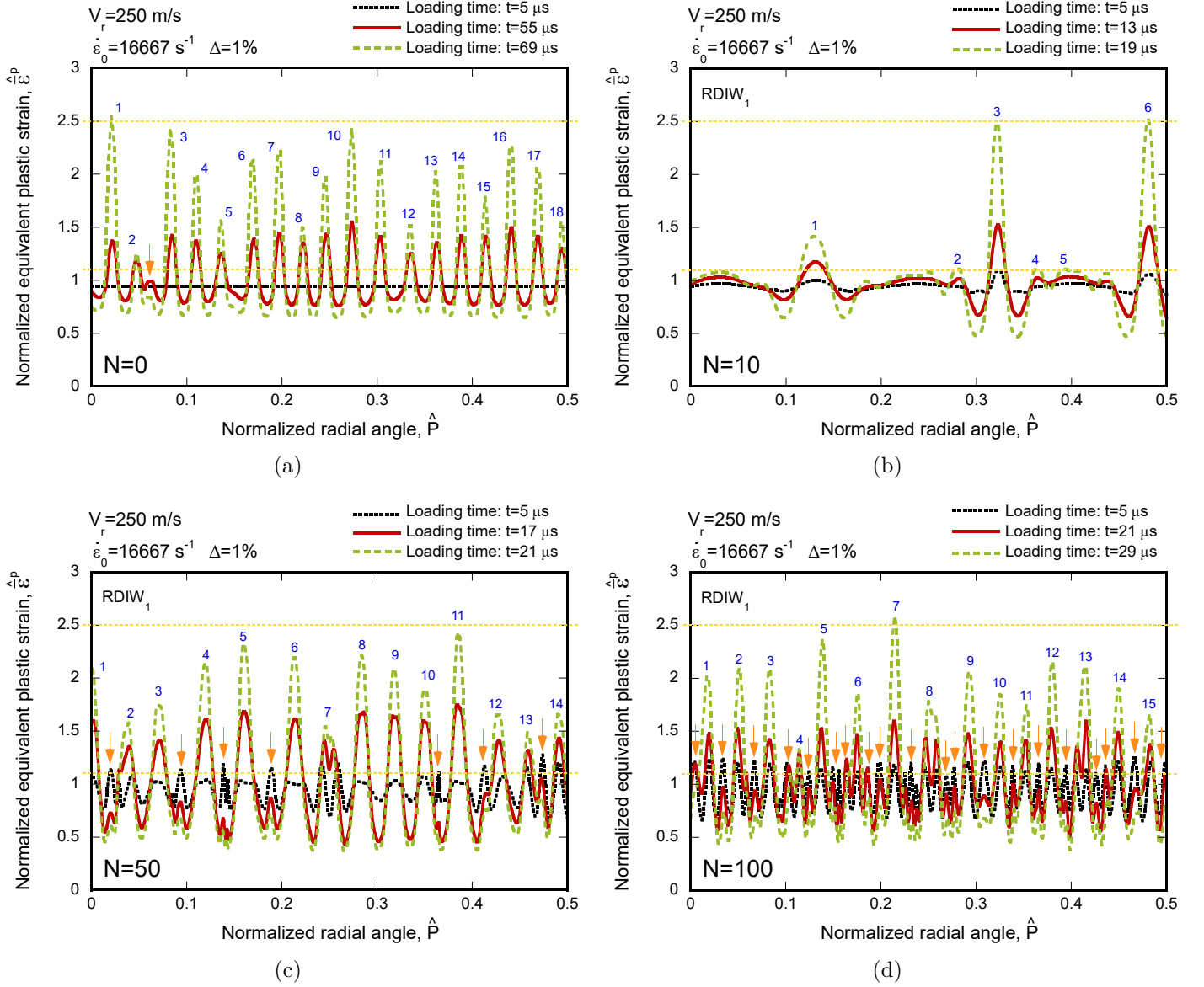
Figure 3: Normalized equivalent plastic strain \hat{\varepsilon}^p versus normalized outer perimeter of the ring \hat{P} . Imposed initial strain rate of \dot{\varepsilon}_0 = 16667 \text{ s}^{-1} (which corresponds to V_r = 250 \text{ m/s} ). (a) Number of imperfections N = 0 . Three loading times t are considered: 5 \mu s , 55 \mu s and 69 \mu s . (b) Number of imperfections N = 10 . Three loading times t are considered: 5 \mu s , 13 \mu s and 19 \mu s . (c) Number of imperfections N = 50 . Three loading times t are considered: 5 \mu s , 17 \mu s and 21 \mu s . (d) Number of imperfections N = 100 . Three loading times t are considered: 5 \mu s , 21 \mu s and 29 \mu s . For N = 10, 50 and 100 the amplitude of the imperfections is \Delta = 1\% and the random distribution of imperfection wavelengths is RDIW_1 . The horizontal yellow dashed lines correspond to the conditions \hat{\varepsilon}^p = 1.1 and \hat{\varepsilon}^p = 2.5 . For interpretation of the references to color in this figure, the reader is referred to the web version of this article.
