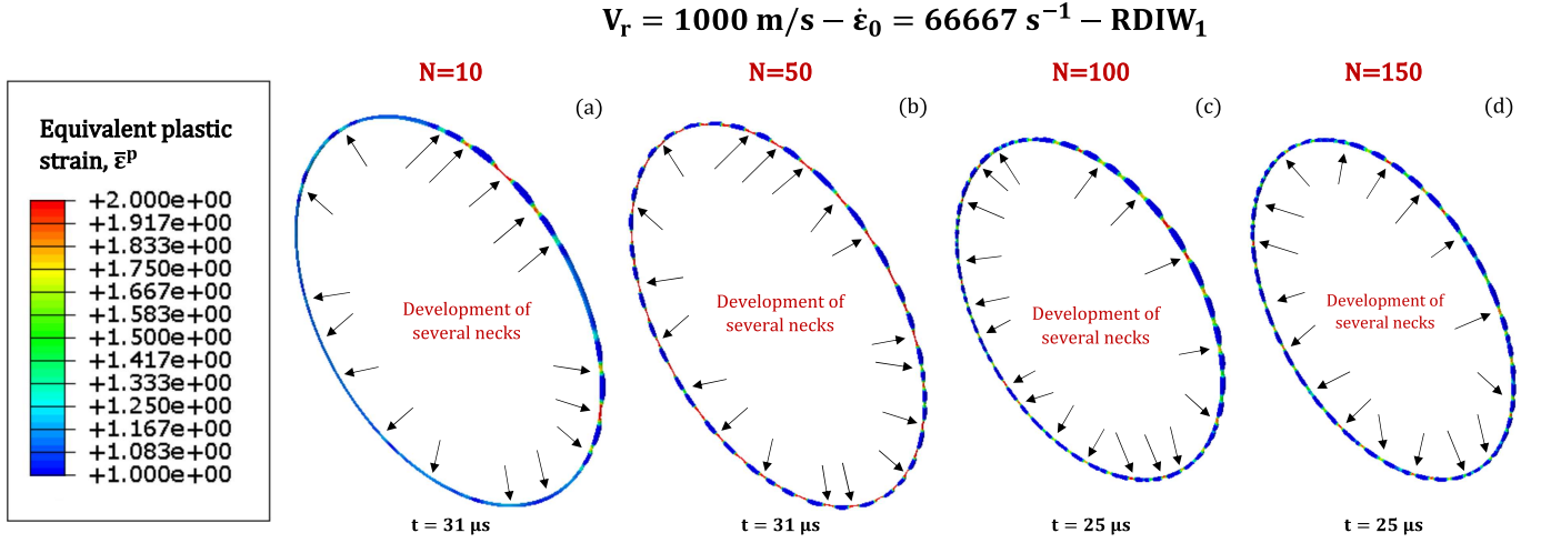
Figure 11: Contours of equivalent plastic strain \bar{\epsilon}^p . Imposed initial strain rate of \dot{\epsilon}_0 = 66667 \text{ s}^{-1} (which corresponds to V_r = 1000 \text{ m/s} ). (a) Number of imperfections N = 10 . Loading time t = 31 \mu\text{s} . (b) Number of imperfections N = 50 . Loading time t = 31 \mu\text{s} . (c) Number of imperfections N = 100 . Loading time t = 25 \mu\text{s} . (d) Number of imperfections N = 150 . Loading time t = 25 \mu\text{s} . The amplitude of the imperfections is \Delta = 1\% and the random distribution of imperfection wavelengths is \text{RDIW}_1 .
