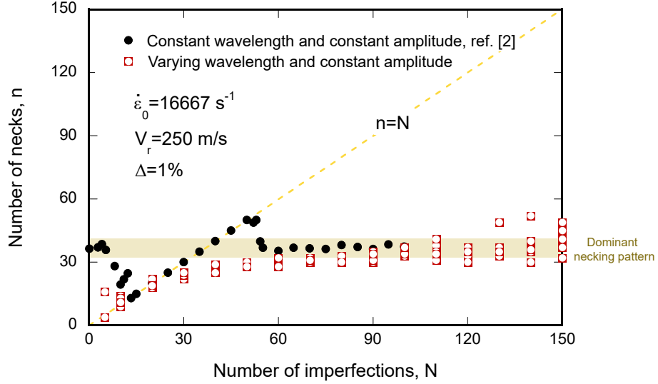
Figure 8: Number of necks n as a function of the number of imperfections N for an imposed initial strain rate of \dot{\epsilon}_0 = 16667 \text{ s}^{-1} (which corresponds to V_r = 250 \text{ m/s} ). The results obtained for five random distributions of imperfection wavelengths (RDIW _i with i = 1, \dots, 5 ) are compared with the finite element calculations performed by Rodríguez-Martínez et al. [33] for rings with constant wavelength imperfections. The amplitude of the imperfections is \Delta = 1\% .
