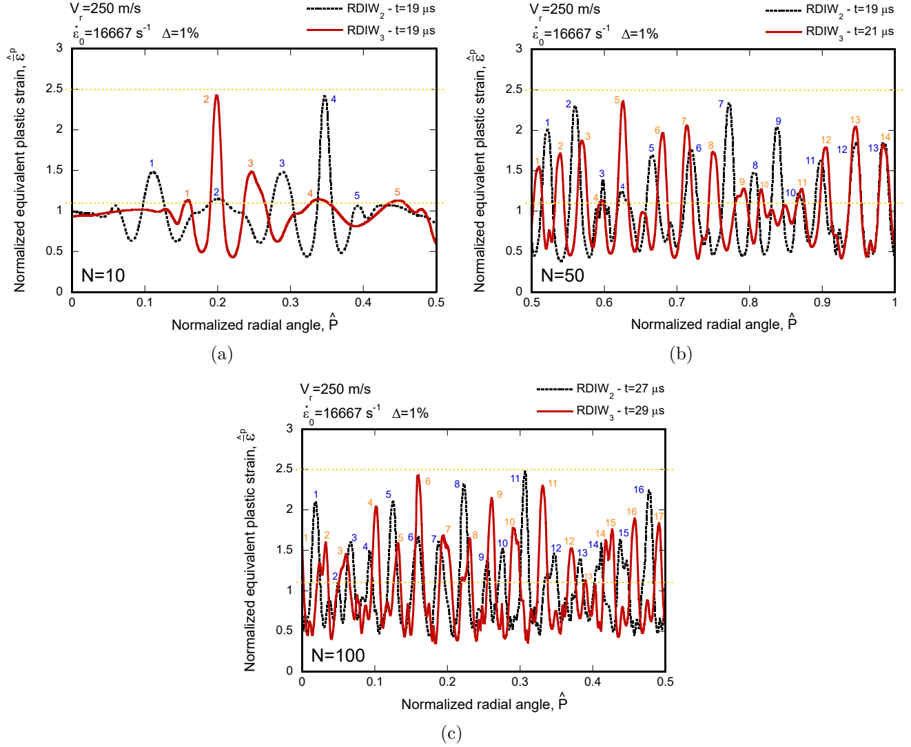
Figure 6: Normalized equivalent plastic strain \hat{\epsilon}^p versus normalized outer perimeter of the ring \hat{P} . Imposed initial strain rate of \dot{\epsilon}_0 = 16667 \text{ s}^{-1} (which corresponds to V_r = 250 \text{ m/s} ). Results are shown for two random distributions of imperfection wavelengths: \text{RDIW}_2 and \text{RDIW}_3 . The amplitude of the imperfections is \Delta = 1\% . (a) Number of imperfections N = 10 . The loading time for both \text{RDIW}_2 and \text{RDIW}_3 is t = 19 \mu\text{s} . (b) Number of imperfections N = 50 . The loading times for \text{RDIW}_2 and \text{RDIW}_3 are t = 19 \mu\text{s} and t = 21 \mu\text{s} , respectively. (c) Number of imperfections N = 100 . The loading times for \text{RDIW}_2 and \text{RDIW}_3 are t = 27 \mu\text{s} and t = 29 \mu\text{s} , respectively. The horizontal yellow dashed lines correspond to the conditions \hat{\epsilon}^p = 1.1 and \hat{\epsilon}^p = 2.5 . For interpretation of the references to color in this figure, the reader is referred to the web version of this article.
