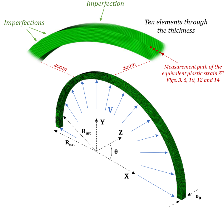
Figure 1: Finite element model. Mesh, geometry and boundary conditions. Note that, due to the symmetry of the specimen, only half of the ring is shown. The number of imperfections is N = 40 and the amplitude of the imperfections is \delta = 0.01 \text{ mm} .
