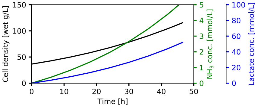
FIGURE 4.2: Fed-batch simulation in an O 2 -sparged 20 m 3 bioreactor with 80% max working volume and the stoichiometry of Reaction 2.11.
