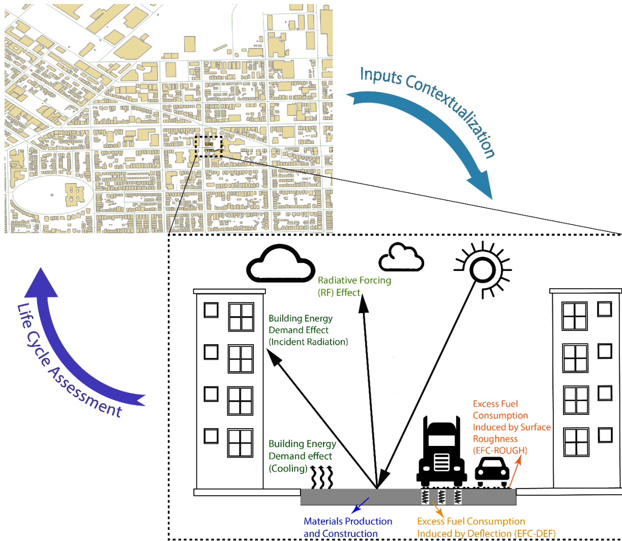
Figure 1. Overview of the methodology and life cycle components of pavements in urban areas. Considering the interconnection among the elements of the built environment, a top-down approach was developed to capture the effect of cool pavement strategies on the GHG balance of cities.
