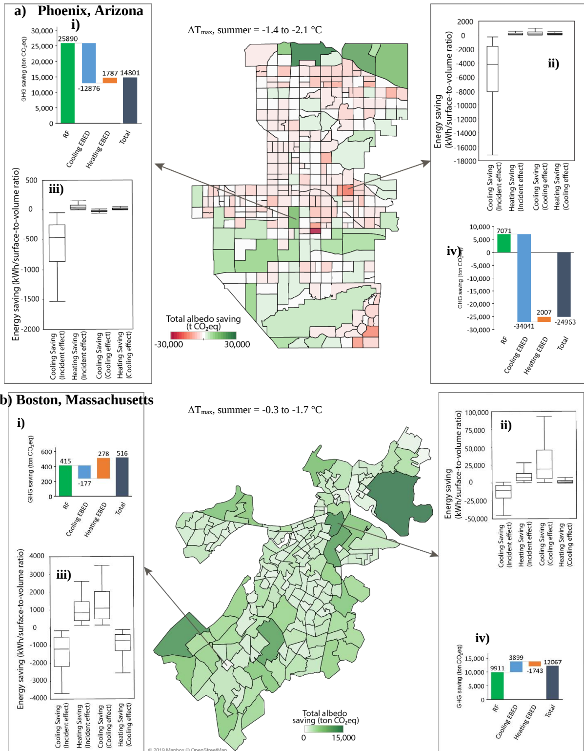
Figure 2. Albedo-induced GHG savings from increasing albedo by shifting from flexible (existing) to rigid (higher albedo) pavement in the city of a) Phoenix and b) Boston is shown as a heatmap (negative values imply a burden). Temperature decreases across the cities due to the shift in pavement type are shown above each map. The waterfall charts (i and iv) represent the disaggregation of the albedo effect in two different neighborhoods within each city and the box plots (ii and iii) show the contribution of the incident and cooling effect to the total building energy demand in the corresponding census tracts. Note: the scale of the values in the box plots depends on the number of buildings and building stories.
