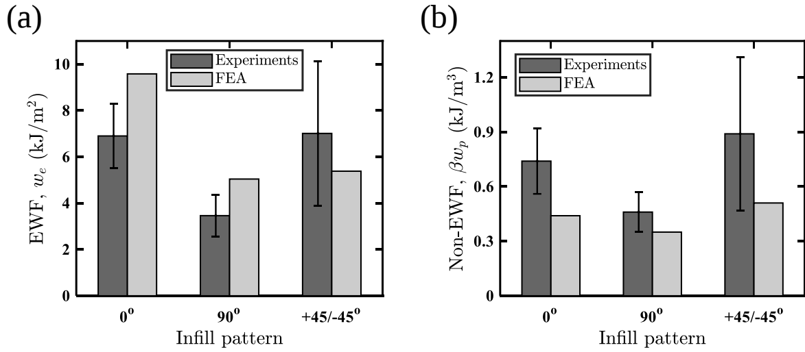
Fig. 6 Predicted and measured EWF (a) and non-EWF (b) for different raster angles.
