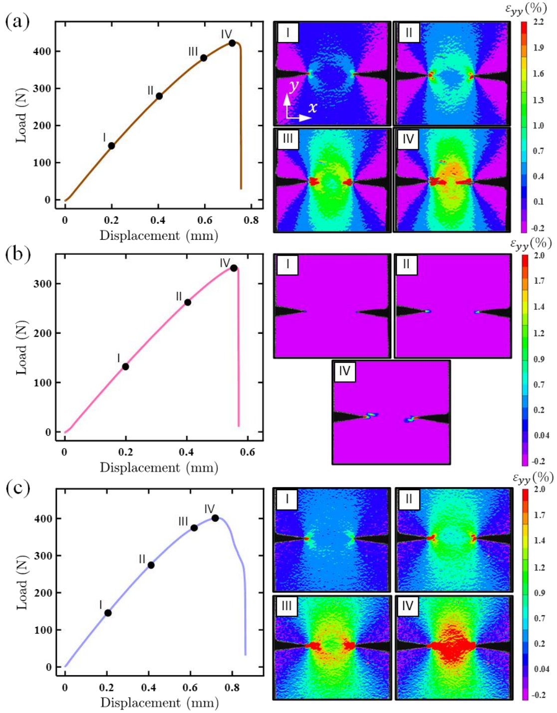
Fig. 3 Load versus displacement curves and contour plots of longitudinal strain in the vicinity of the notch measured via DIC for different raster angles ( L = 12 mm): (a) 0^\circ , (b) 90^\circ and (c) +45/-45^\circ .
