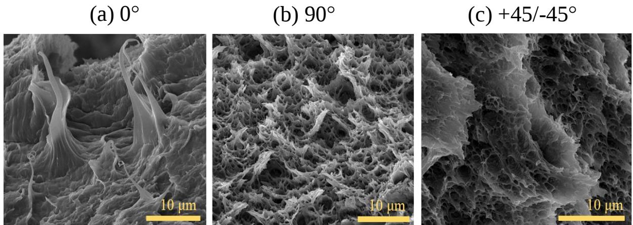
Fig. 7 SEM scans of fracture surfaces for different raster angles.
