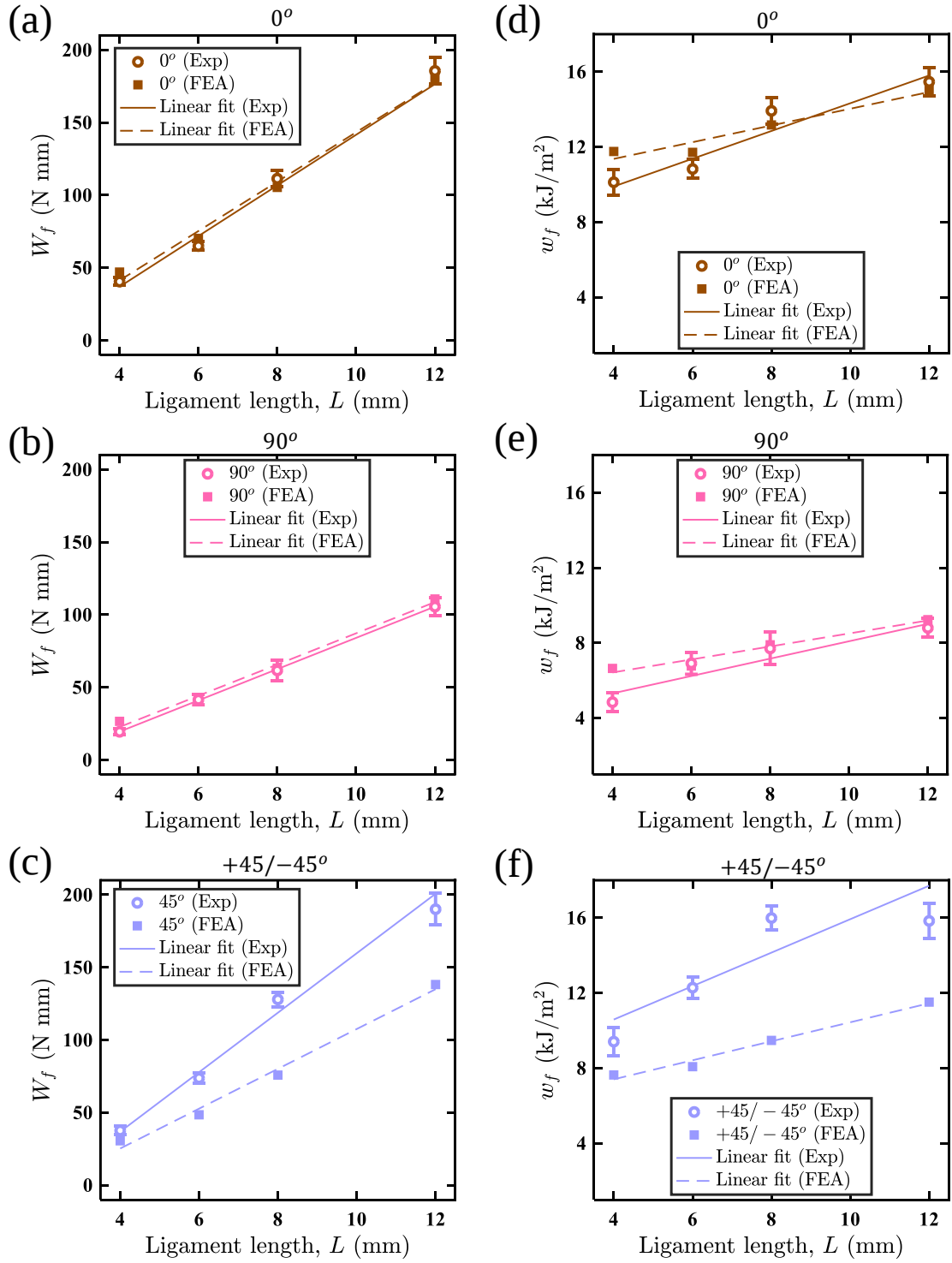
Fig. 5 Measured and predicted work of fracture (a-c) and specific work of fracture (d-f) for different raster angles
