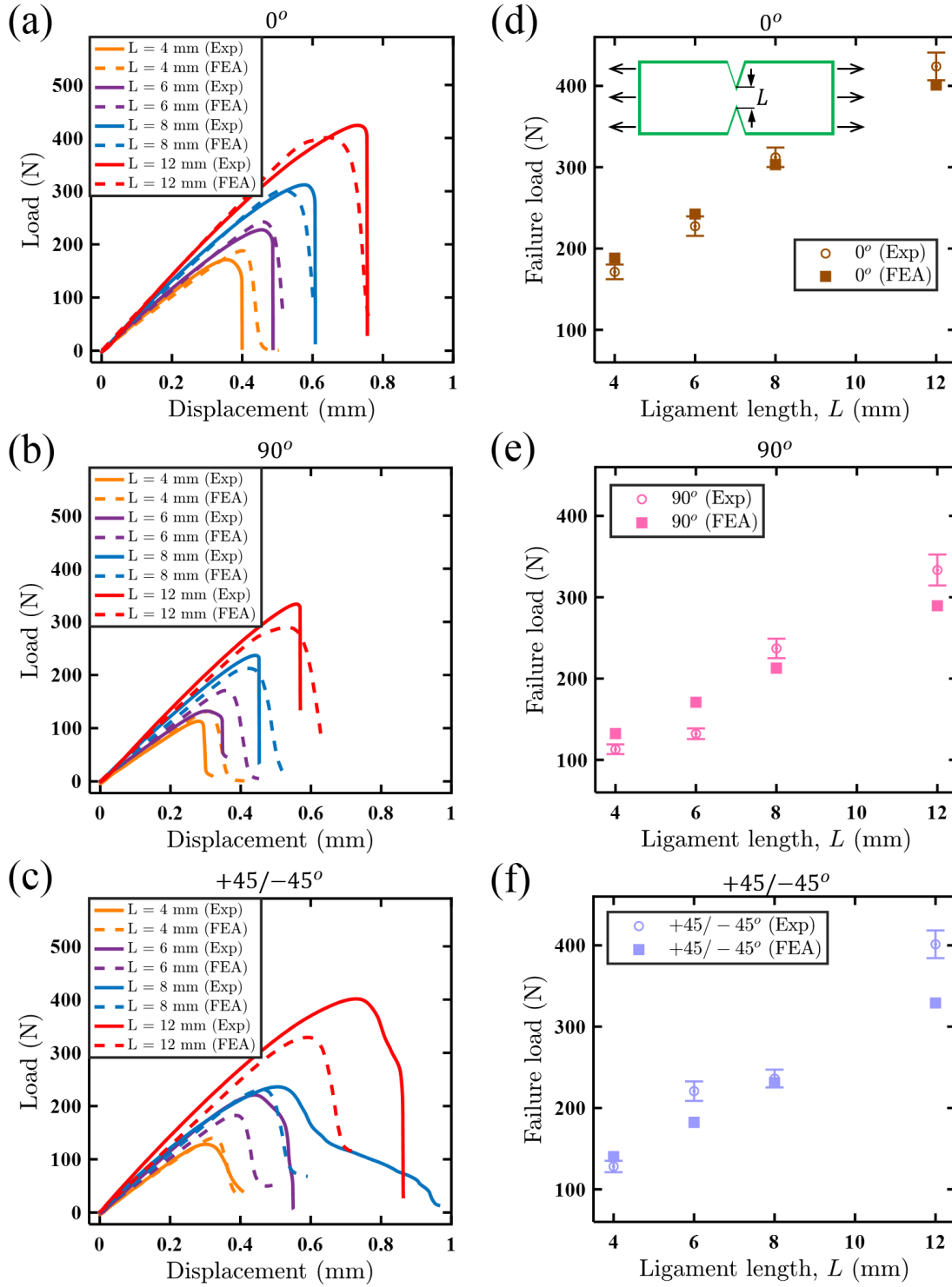
Fig. 2 (a)-(c): Measured and predicted load vs. displacement curves for different raster angles and ligament lengths L ; (d)-(f): ultimate load plotted as a function of ligament length.
