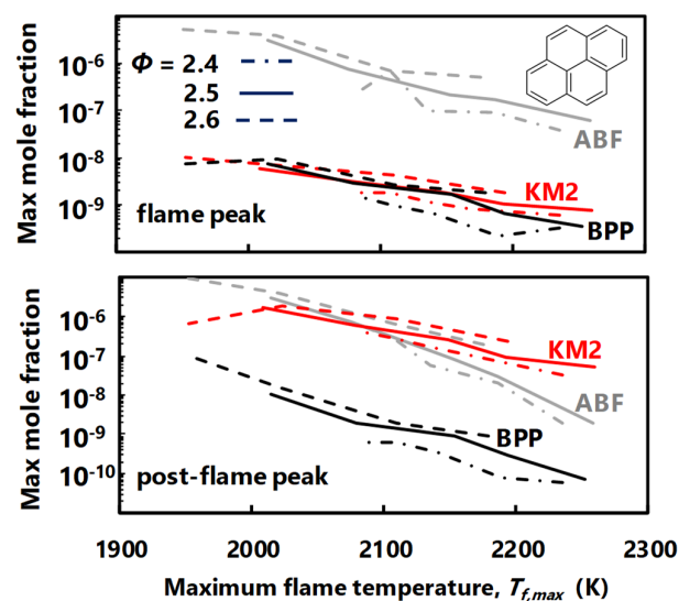
Figure 9: Summary of predicted pyrene concentrations for the series of flame computations using the three PAH mechanisms. The maximum mole fraction in the computed profile is plotted for each flame taking the maximum at the flame zone (top) and the maximum in the post-flame region (bottom).
