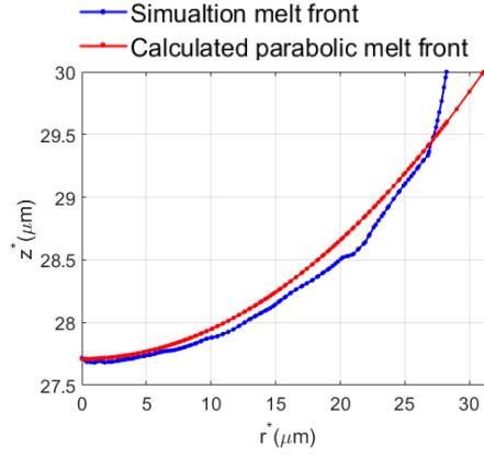
Figure 4: Melt front shape with a parabolic fit
