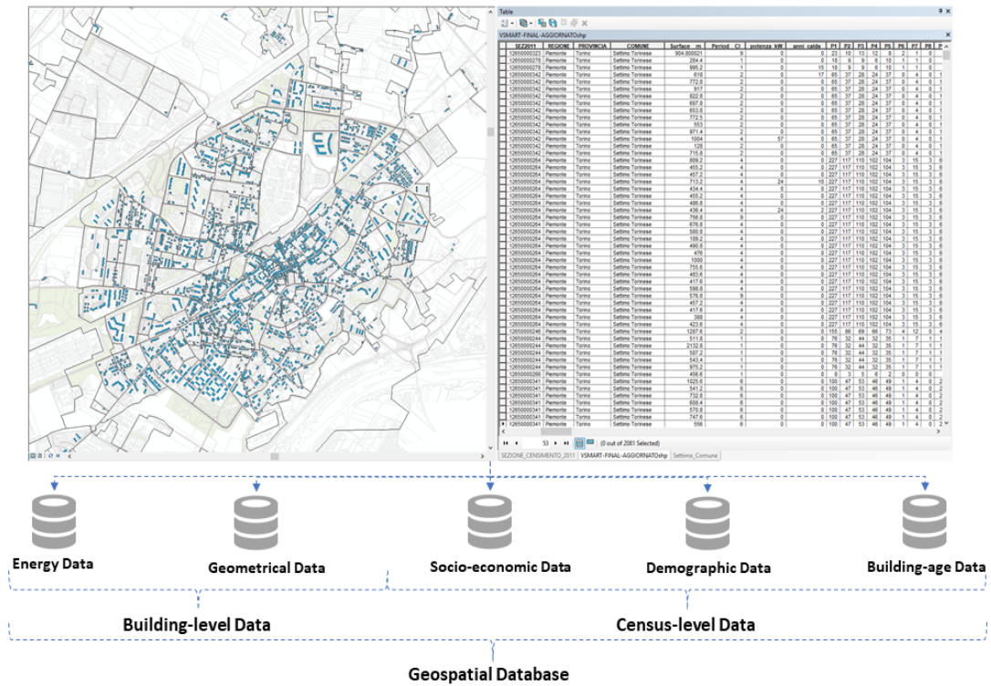
Figure 3. GIS-Database.
