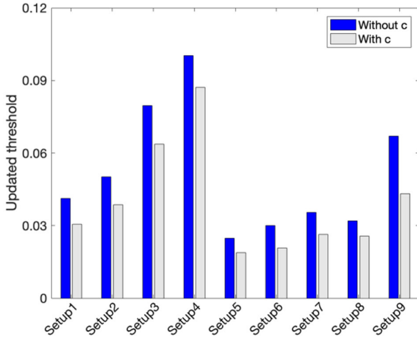
Figure 15. Updated threshold.
