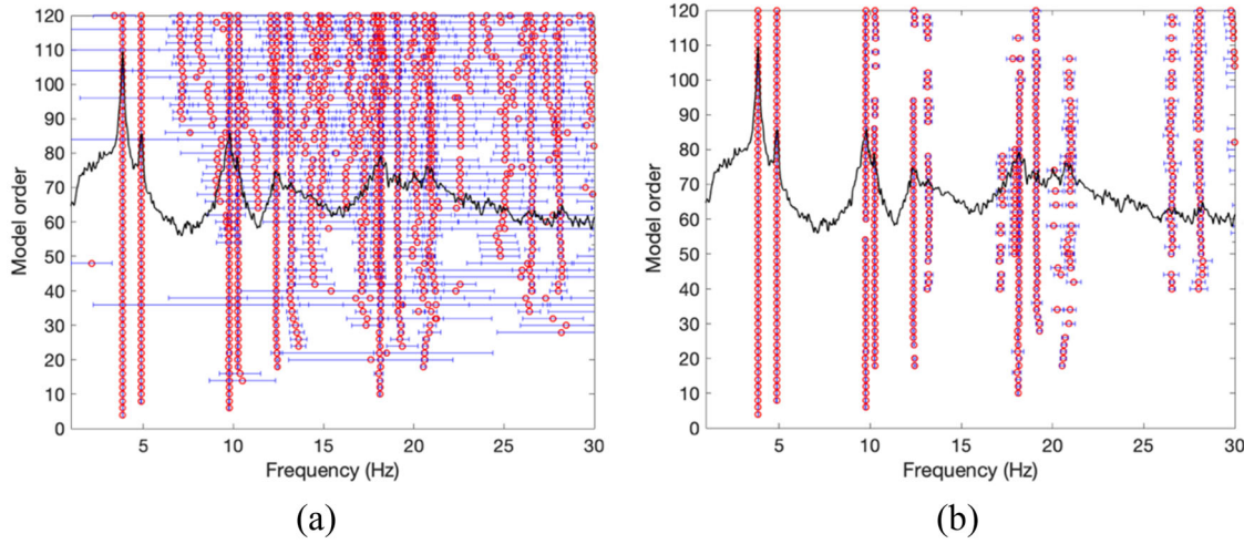
Figure 13. Pre-processing stage for No. 5 set-up: (a) after validation criteria; (b) after uncertainty criterion. Note: \omega is weighting factor in Eq. (9).
