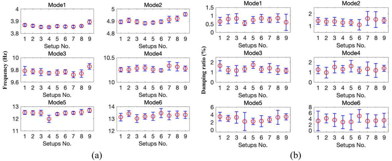
Figure 17. \pm 2\sigma standard deviation error bar ratio across nine setups: (a) frequency; (b) damping ratio.
