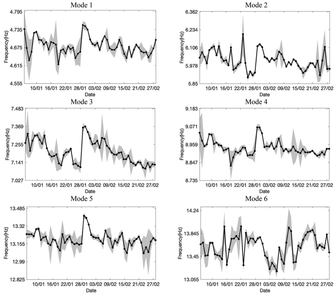
Figure 9. Identified frequency of modes 1–6 with 2-month data. Black solid lines: frequency estimates; grey shaded areas: \pm two standard deviations.
