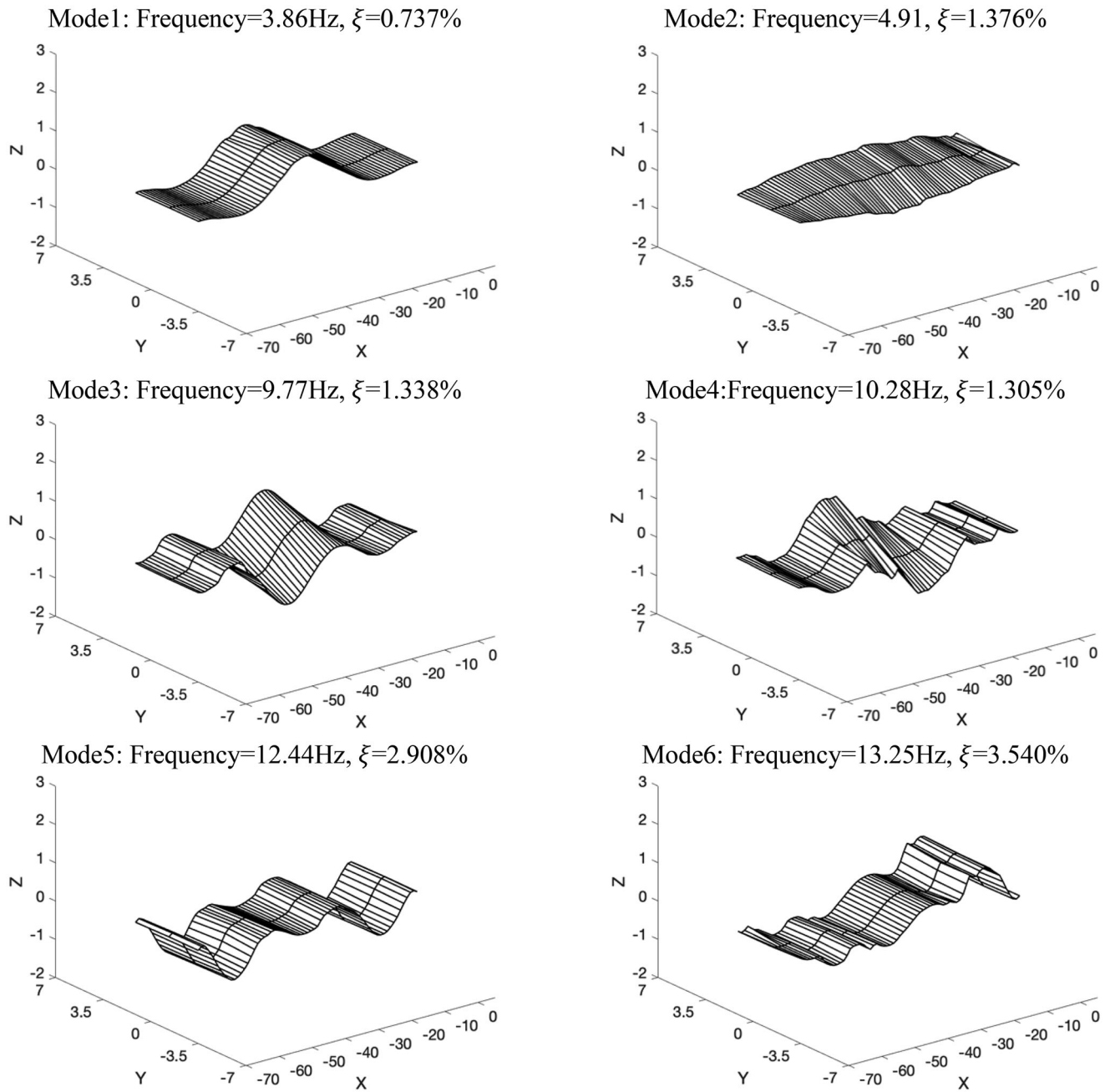
Figure 18. Mode shapes of the Z24 bridge.
