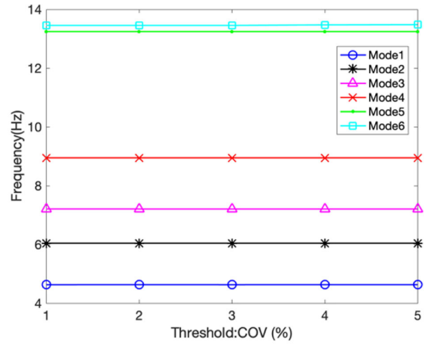
Figure 11. Frequencies at different COV threshold: ( i = 60 ; n_{\max} = 100 ).
