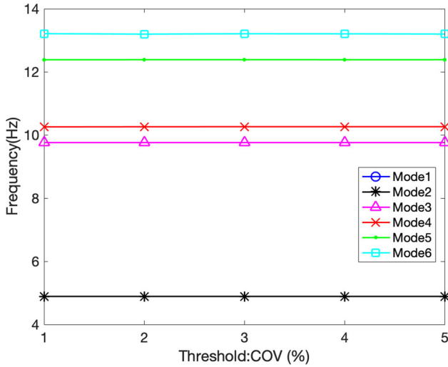
Figure 25. Frequencies at different COV threshold: ( i = 50 , n_{\max} = 120 ).
