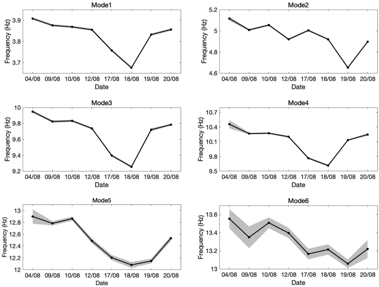
Figure 20. Mode shape at X-Y plane with \pm 2\sigma uncertainty bounds (not visible).
