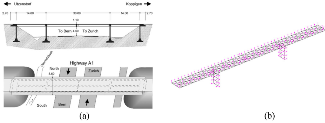
Figure 12. Description of the Z24 bridge: (a) Front and Top view (Maeck & De Roeck, 2003); (b) sensor layout (Döhler et al., 2013).
