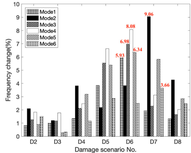
Figure 21. Identified frequencies for different damage scenarios.
