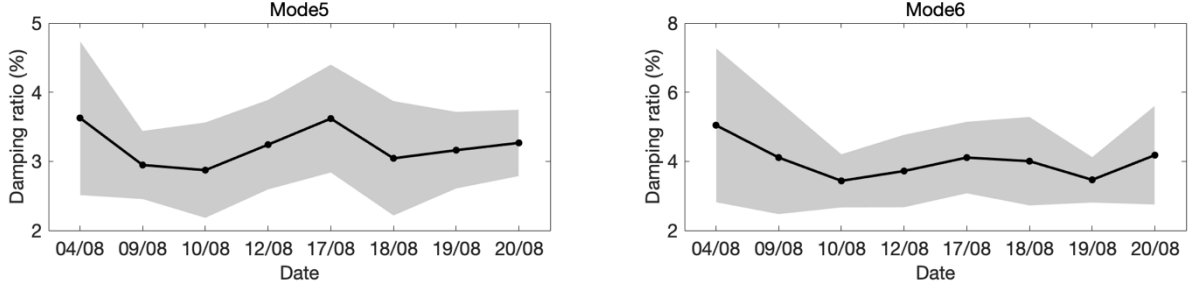
Figure 23. Identified damping ratio for different damage scenarios
