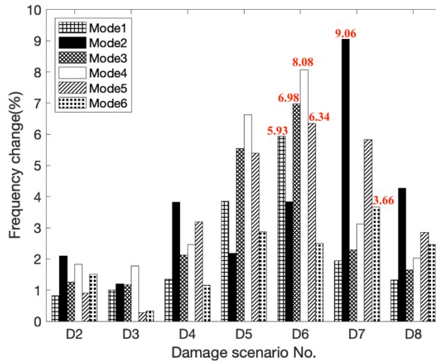
Figure 22. Frequency change due to damage
