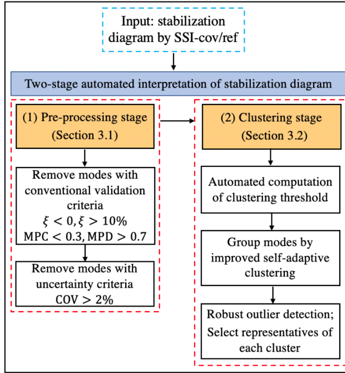
Figure 2. A flowchart of the proposed two-stage approach of automated modal identification
