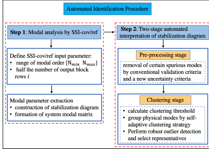
Figure 1. A framework of the proposed automated approach
