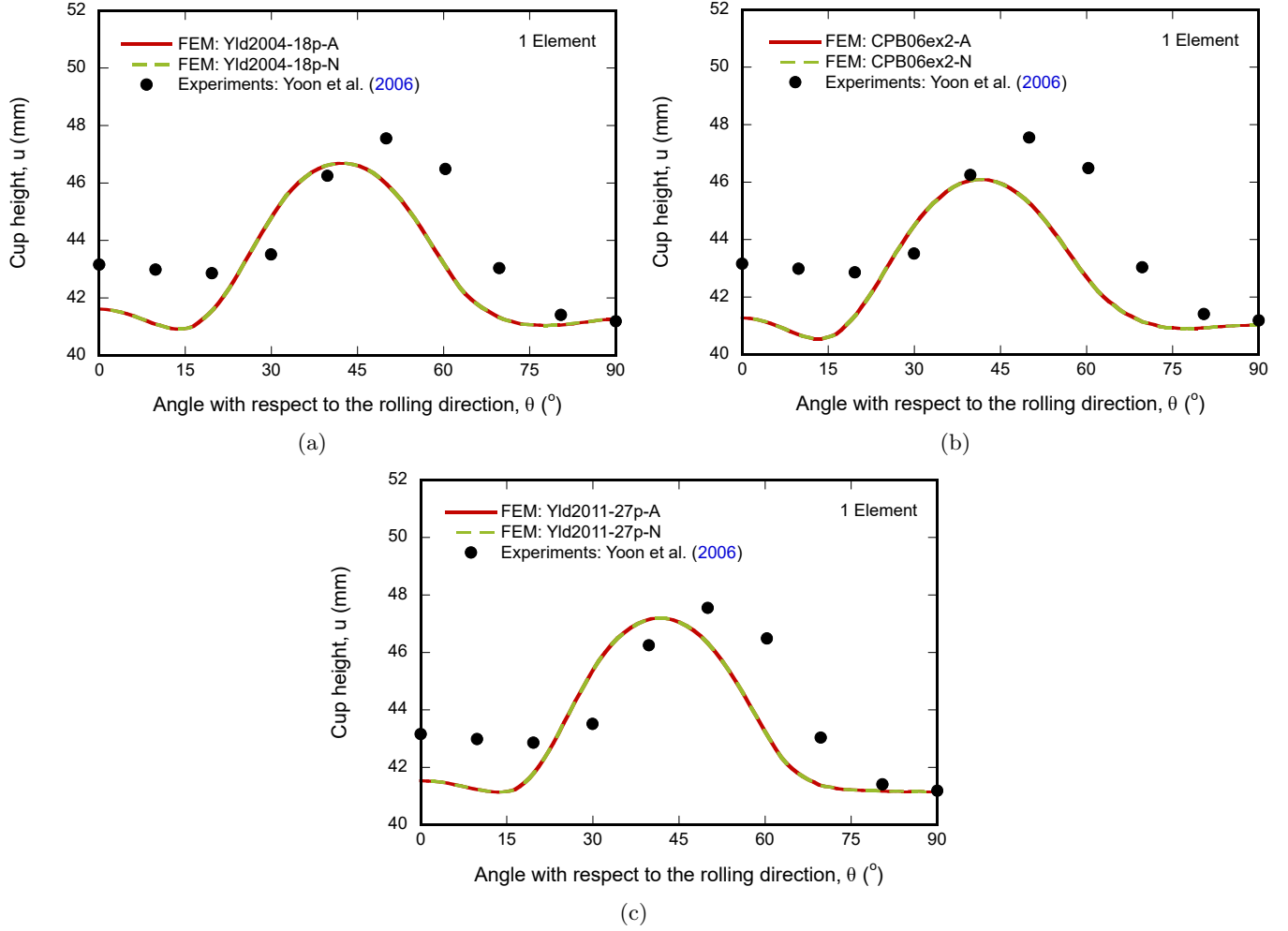
Figure 4: Comparison between finite element simulations (FEM) and experimental results. Cup height u as a function of the angle with respect to the rolling direction \theta . The experimental data are taken from Yoon et al. (2006). The finite elements results are obtained with the analytical derivatives of Appendix A (denoted with -A) and the numerical approximations of Section 5 (denoted with -N). The calculations are performed with 1 element trough the thickness of the sheet. (a) Yld2004-18p-A and Yld2004-18p-N. (b) CPB06ex2-A and CPB06ex2-N. (c) Yld2011-27p-A and Yld2011-27p-N. The simulations have been performed using a dynamic implicit analysis in ABAQUS/Standard and UMAT subroutines for the yield functions implementation.
