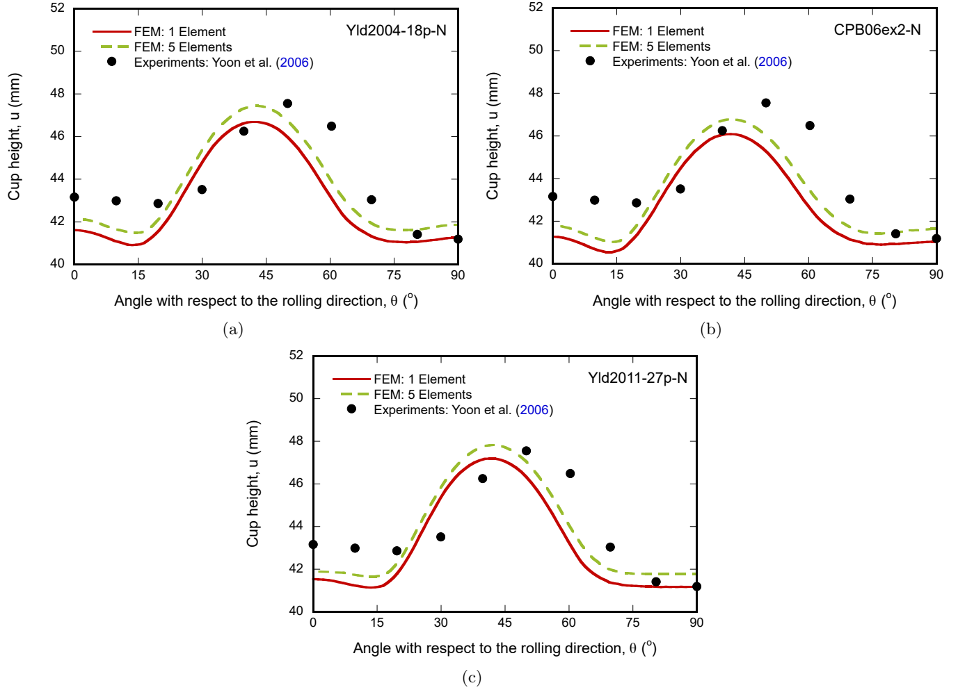
Figure 5: Comparison between finite element simulations (FEM) and experimental results. Cup height u as a function of the angle with respect to the rolling direction \theta . The experimental data are taken from Yoon et al. (2006). The finite elements results are obtained with the numerical approximations of Section 5 (denoted with -N). The calculations are performed with 1 element and 5 elements through the thickness of the sheet. (a) Yld2004-18p-N. (b) CPB06ex2-N. (c) Yld2011-27p-N. The simulations have been performed using a dynamic implicit analysis in ABAQUS/Standard and UMAT subroutines for the yield functions implementation.
