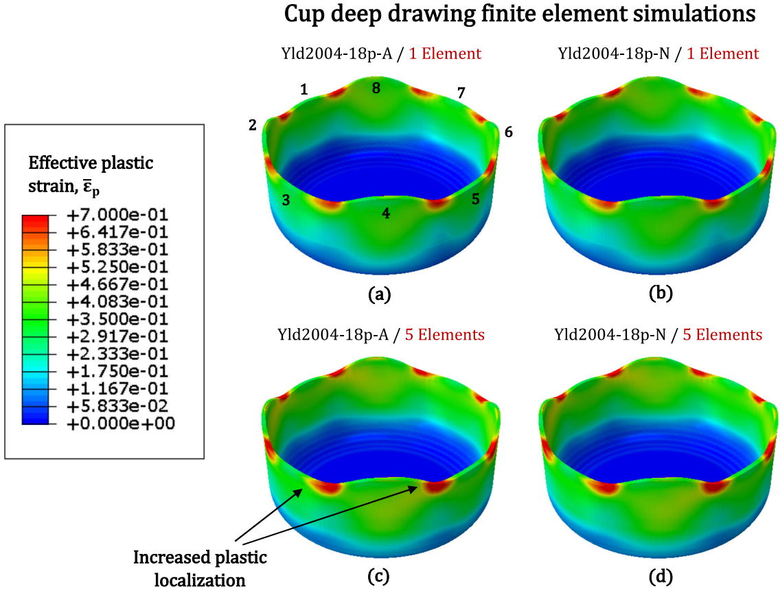
Figure 6: Finite element simulations. Cup deep drawing calculations. Contours of effective plastic strain \bar{\epsilon}_p corresponding to calculations performed with Yld2004-18p yield criterion. Comparison between results obtained with the analytical derivatives of Appendix A (denoted with -A) and the numerical approximations of Section 5 (denoted with -N). Calculations performed with 1 and 5 elements through the thickness. (a) Yld2004-18p-A and 1 element through the thickness. (b) Yld2004-18p-N and 1 element through the thickness. (c) Yld2004-18p-A and 5 elements through the thickness. (d) Yld2004-18p-N and 5 elements through the thickness. The simulations have been performed using a dynamic implicit analysis in ABAQUS/Standard and UMAT subroutines for the yield function implementation.
