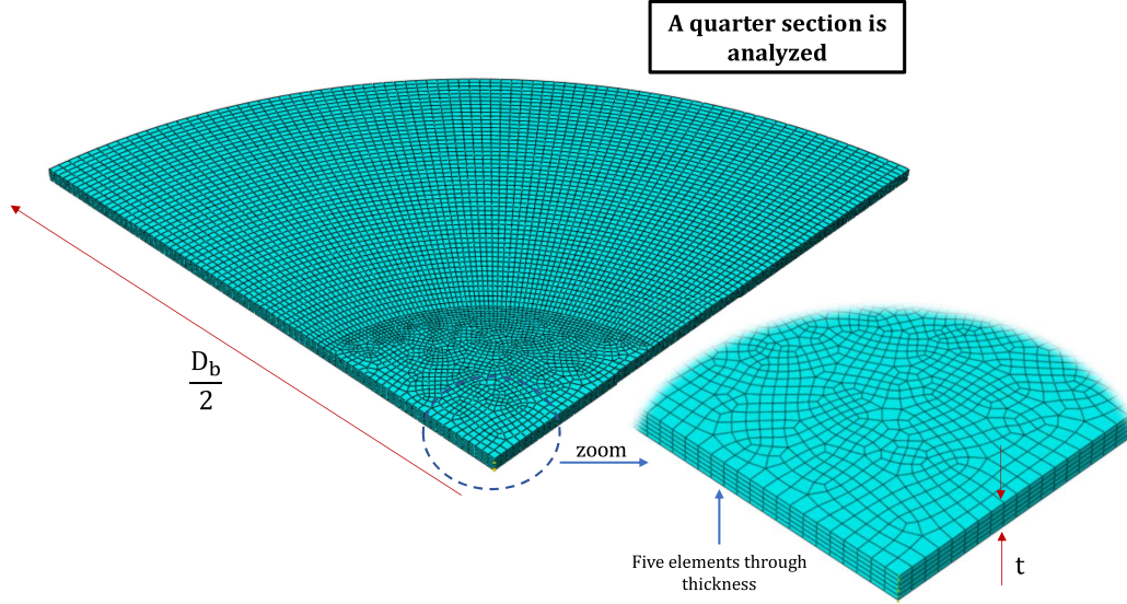
Figure 2: Blank mesh used in the finite element simulations. Five elements through the thickness of the sheet. Total number of elements: 29575.
