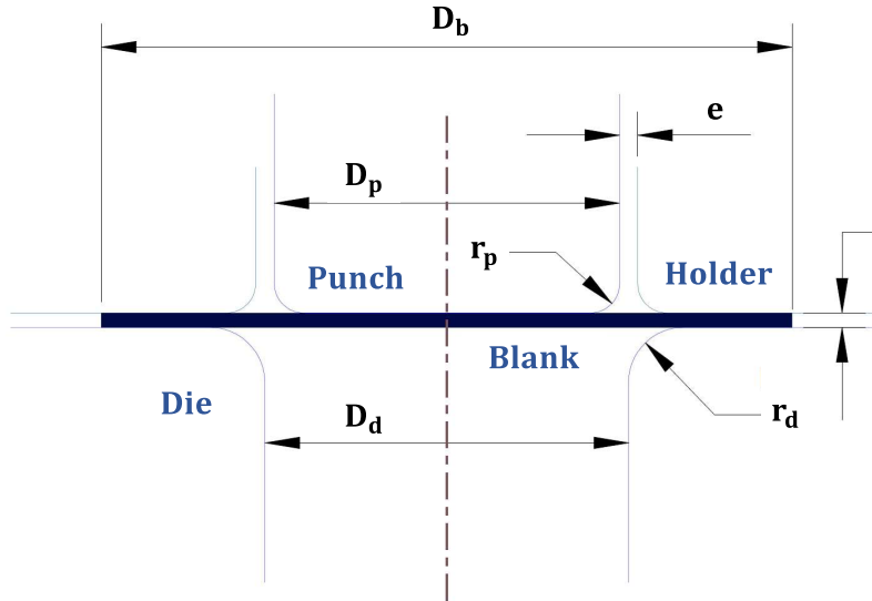
Figure 1: Tools and blank geometries for cylindrical cup deep drawing. This figure is adapted from Yoon et al. (1999, 2004).
