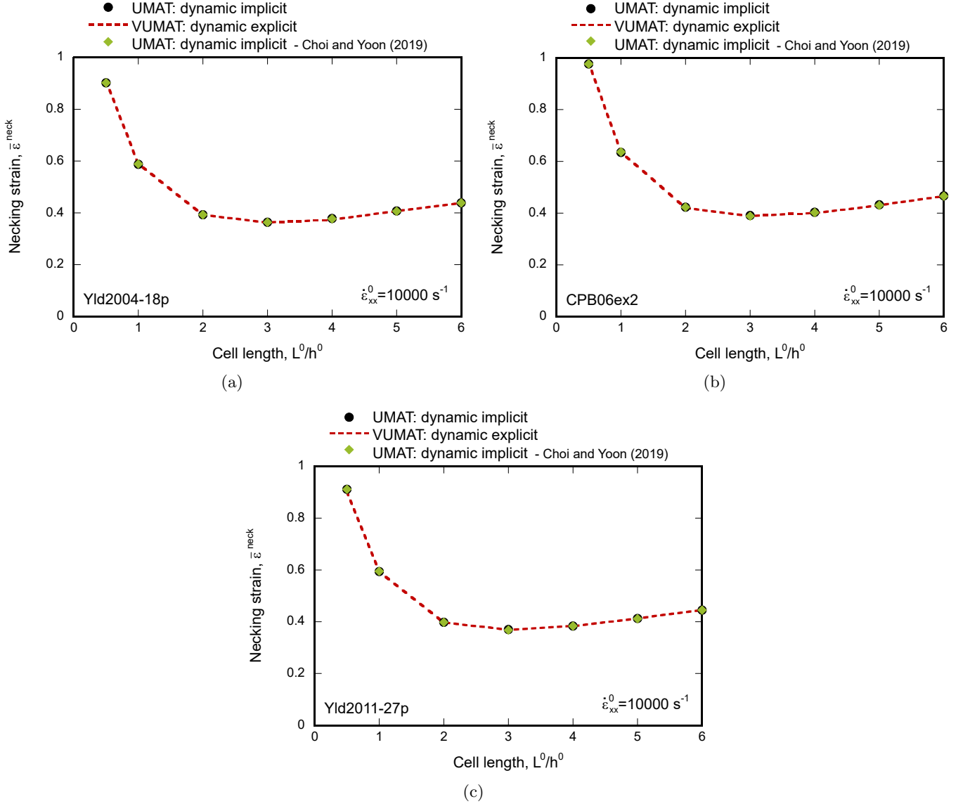
Figure 9: Finite element results. Evolution of the necking strain \bar{\varepsilon}^{neck} with the cell length L^0/h^0 . Comparison between dynamic implicit and explicit simulations performed with UMAT and VUMAT subroutines, respectively. The imposed initial strain rate is \dot{\varepsilon}_{xx}^0 = 10000 \text{ s}^{-1} . The results are obtained with the numerical approximation of the yield function gradients of Section 5 and the numerical differentiation scheme proposed by Choi and Yoon (2019), which is shown in Appendix B. The calculations are performed with three yield criteria: (a) Yld2004-18p-N, (b) CPB06ex2-N and (c) Yld2011-27p-N.
