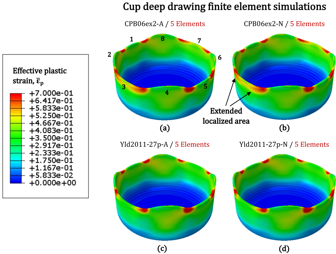
Figure 7: Finite element simulations. Cup deep drawing calculations. Contours of effective plastic strain \bar{\epsilon}_p corresponding to calculations performed with 5 elements through the thickness. Comparison between results obtained with the analytical derivatives of Appendix A (denoted with -A) and the numerical approximations of Section 5 (denoted with -N). (a) CPB06ex2-A. (b) CPB06ex2-N. (c) Yld2011-27p-A. (d) Yld2011-27p-N. The simulations have been performed using a dynamic implicit analysis in ABAQUS/Standard and UMAT subroutines for the yield functions implementation.
