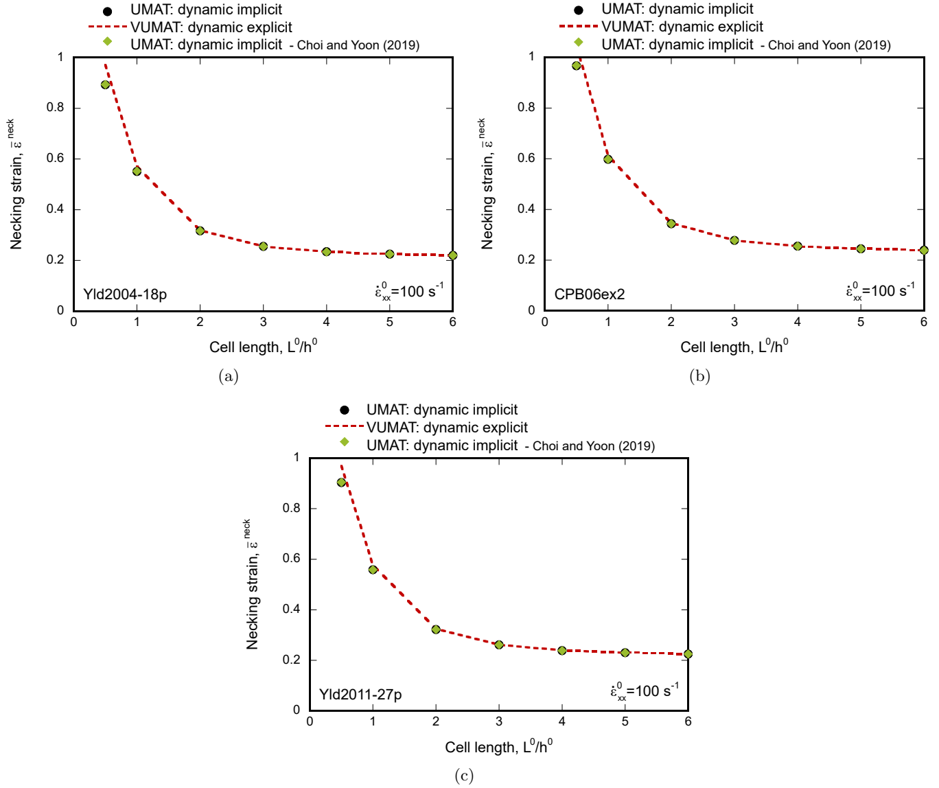
Figure 8: Finite element results. Evolution of the necking strain \bar{\varepsilon}^{neck} with the cell length L^0/h^0 . Comparison between dynamic implicit and explicit simulations performed with UMAT and VUMAT subroutines, respectively. The imposed initial strain rate is \dot{\varepsilon}_{xx}^0 = 100 \text{ s}^{-1} . The results are obtained with the numerical approximation of the yield function gradients of Section 5 and the numerical differentiation scheme proposed by Choi and Yoon (2019), which is shown in Appendix B. The calculations are performed with three yield criteria: (a) Yld2004-18p-N, (b) CPB06ex2-N and (c) Yld2011-27p-N.
