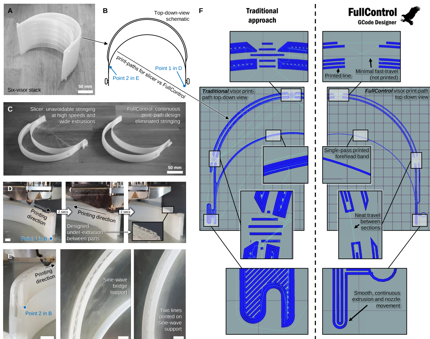
Figure 6 Comparison between traditional slicer software and FullControl print -paths for a visor frame that was printed over 1,000 times. A) Stack of six visor frames printed together. B) Simplified top-view schematic of the print-path. C) Slicing software led to stringing and blemishes when printing at higher speeds. D) FullControl allowed precise design of under-extrusion between parts in a stacked print, resulting in connected droplets that sufficiently supported subsequent parts, whilst allowing separation by hand. E) A sine wave was printed to act as support when a gap needed to be bridged. F) Print-path previews for the original GCode produced by slicing software and the GCode produced by FullControl. By using the FullControl design approach, production rate increased by 400% to 600%, post-processing time was reduced, material usage was reduced, aesthetics was improved, comfort for the end-user was improved and printer reliability was improved. Video S5 in supporting data [34] shows the printing process for (E). Grid in (F) = 10 mm. Scale bars = 5 mm unless otherwise indicated.
