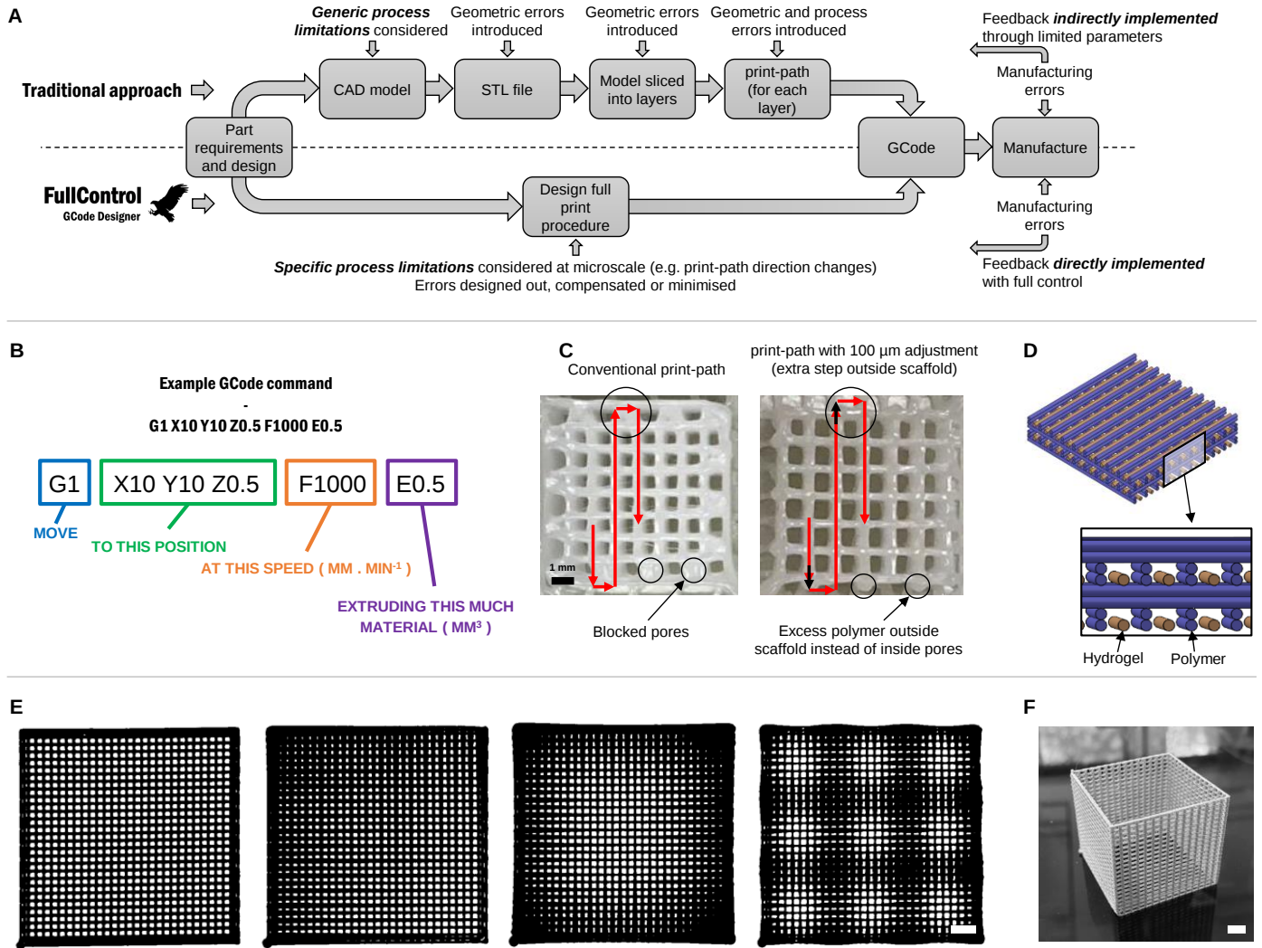
Figure 1 The FullControl design approach and example parts. A) Flow chart comparing the traditional approach using 3D printing slicing software and the FullControl approach, in which the geometric print-path and all non-geometric printing instructions are explicitly designed. B) Example line of GCode for one print-path segment. C) Example adjustment to the print-path (moving the nozzle outside of the structure) [30]. D) Example print-path with multiple materials printed at different heights above the print platform in a designed non-sequential manner [3]. E) An identical print-path was used to print several different graded meshes, by designing a variable extrusion width [31]. F) A single-filament-wide mesh wall printed by combining vertical extrusion (away from the print platform) with horizontal extrusion (parallel to the print platform). All parts of the figure, even when linked to publications, were created from original media. Scale bars = 5 mm unless otherwise indicated.
