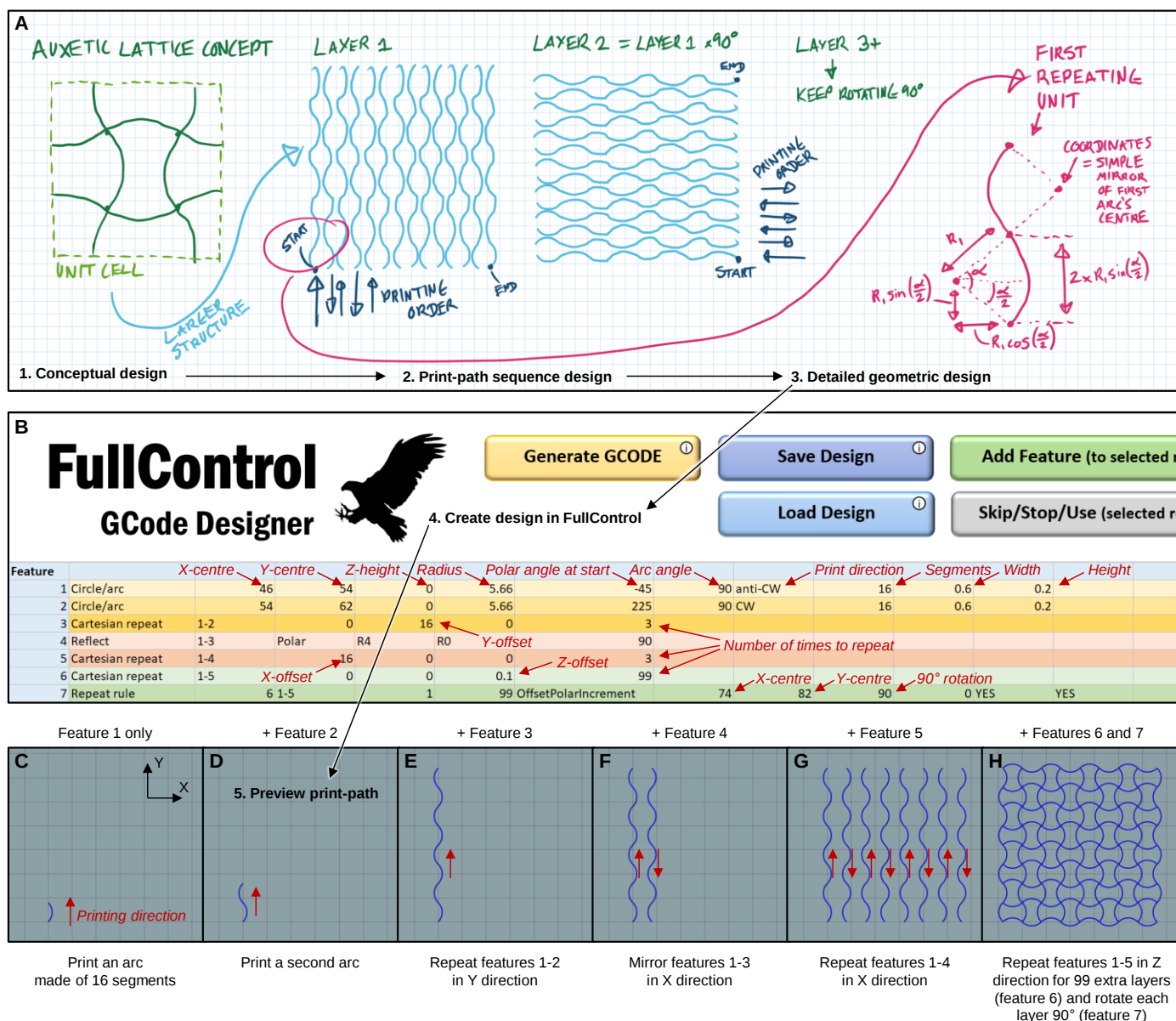
Figure 3 Design workflow for the FullControl design approach. A) Hand-drawn schematics are useful to (1) conceptually design the structure, (2) design the print-path sequence to achieve the concept structure, and (3) identify the detailed geometric information necessary for technical design of the structure in the FullControl software. B) User interface screenshot of FullControl GCode Designer, showing seven features that describe the design in (A) and are evaluated sequentially to generate GCode. Parameters of the 'Circle/arc' feature are identified with labelled arrows for cross-reference to Section 3.3. C-H) Previews of the GCode after sequential inclusion of each of the seven features in (B). The arrow-linked steps labelled 1 to 5 are listed and described in Section 3.4. Grid in (C-H) = 10 mm.
