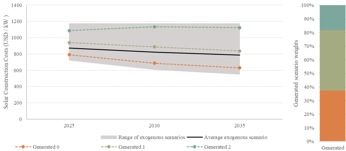
Figure 27 Generated scenarios and scenario weights compared to exogenous scenario range for solar PV construction costs.
