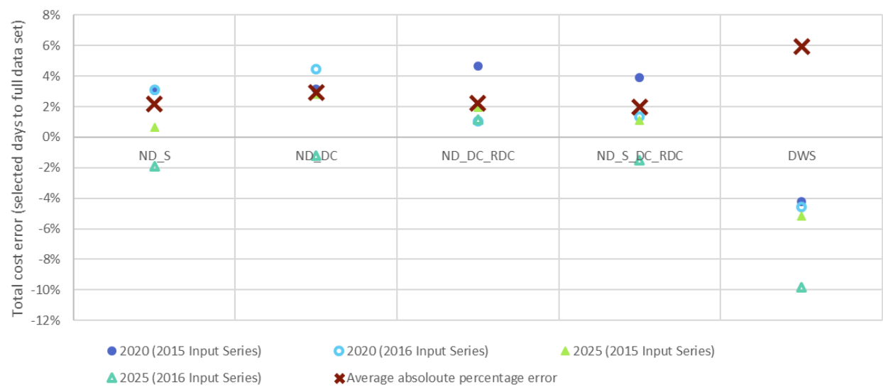
Figure 9 Percentage error in representative day cost estimation between GEP model with representative days and unit commitment results over full dataset by capacity expansion model year (2020 or 2025) and input data series year (2015 or 2016)
